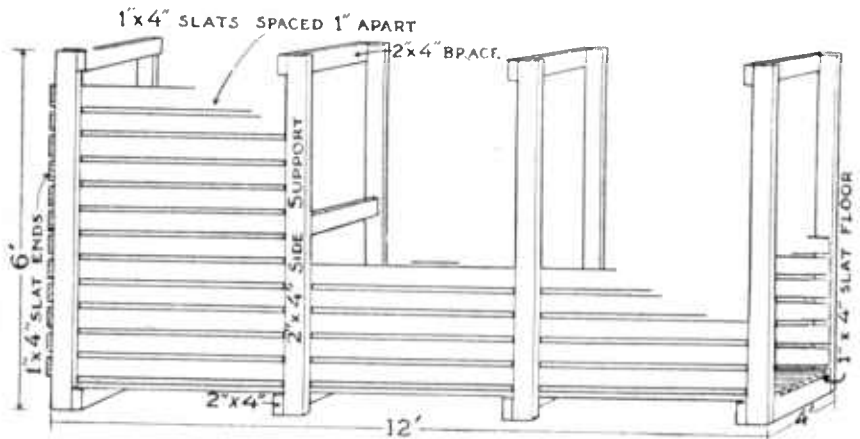
FIG. 6.—Diagram showing the construction of a bin for storing sweet potatoes in a tobacco barn.
