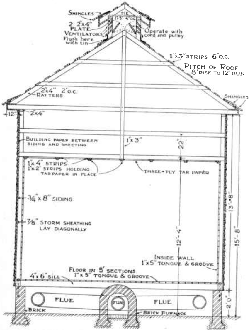
FIG. 5.—Plan showing the end of a frame tobacco barn when converted into a sweet-potato storage house.
