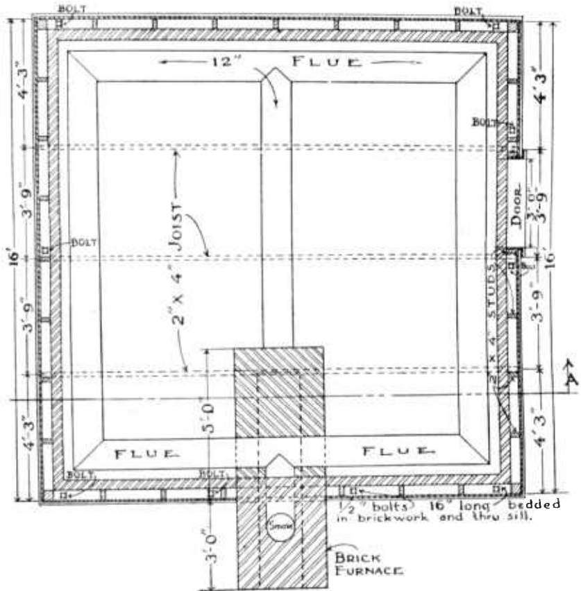
FIG. 4.—Ground-floor plan of a single-frame tobacco barn, showing the arrangement of the furnace and flues; also the foundation and side walls.
