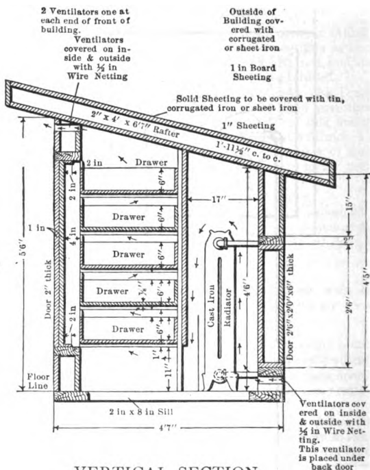
VERTICAL SECTION.
