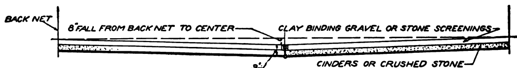
1356. Draining a tennis-court.
