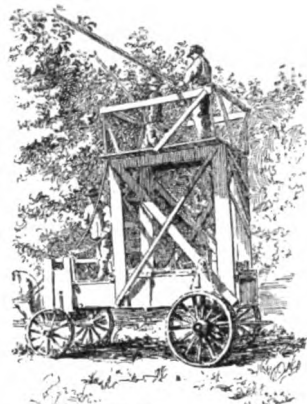
1332. Square tower, giving more working space for the nozzle-men than the conical form.
