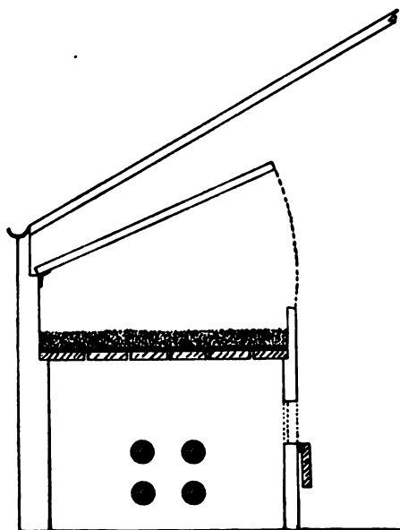
1160. Section of propagating-bed. Shows four pipes beneath, the door in the side, and the frame cover.
