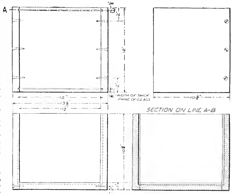
288. Working drawings for making box shown in Fig. 287.
