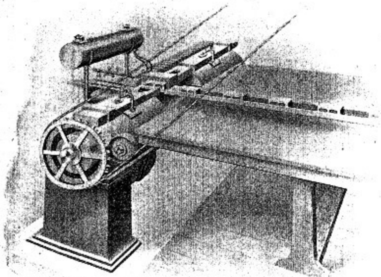
Fig. 18.—Automatic stamper.
