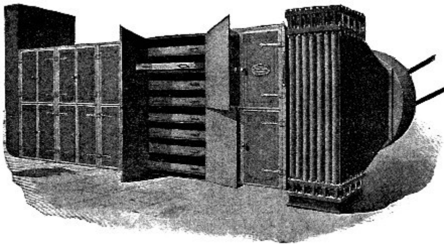
Fig. 21.—Soap-drying apparatus.
