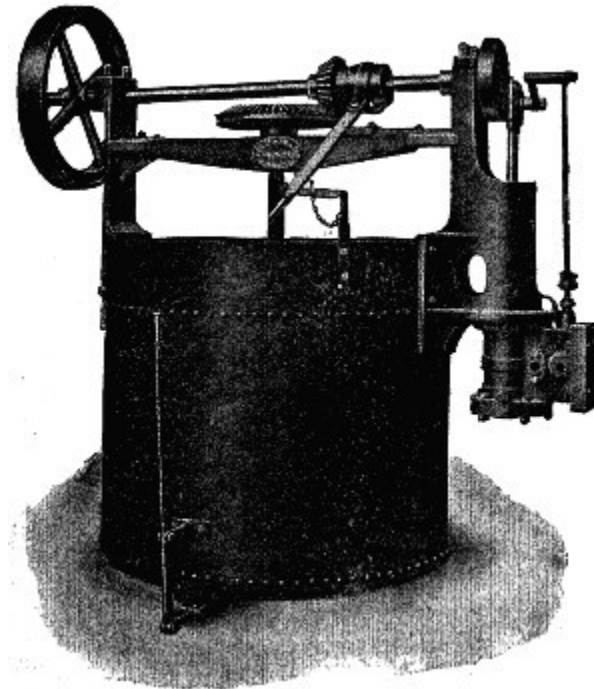
Fig. 6.—Mechanical crutcher.
