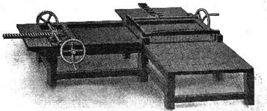
Fig. 14.—Tablet-cutting machine.
