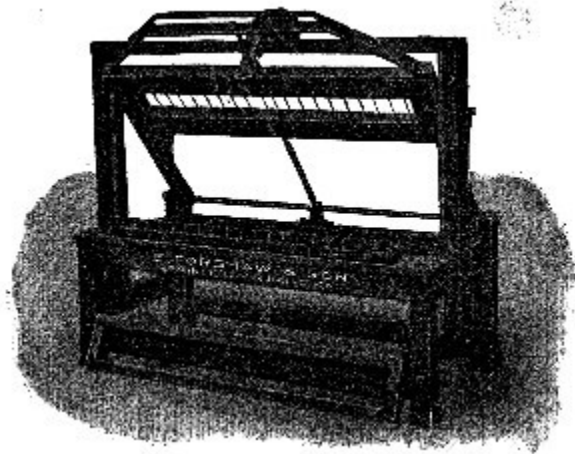
Fig. 12.—Barring machine.
