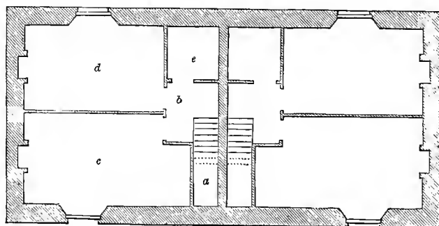
Fig. 749.—Chamber-floor plan of fig. 748.
