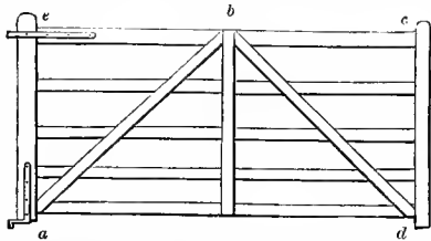
Fig. 604.—Common wooden field-gate.
