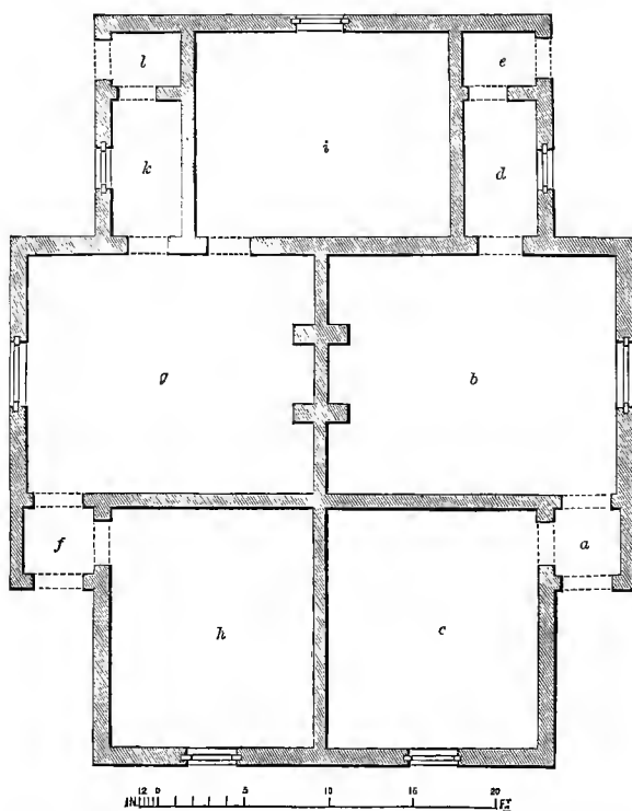
Fig. 762.—Ground-plan of single-storeyed double cottages, consisting of larger and smaller houses.
