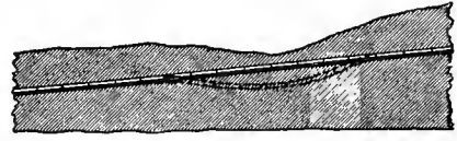
Fig. 655.—Showing the line of pipes truly laid with regular fall, and pipes improperly laid on uneven bottom.
