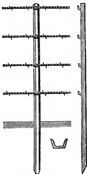
Fig. 586.—Standard for barb-wire.
