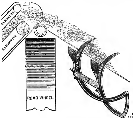
Fig. 509.—Conveyor-roll.
