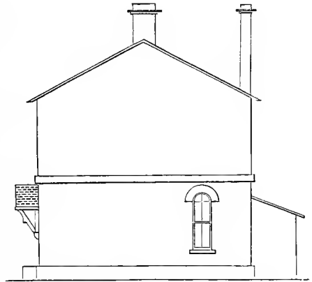
Fig. 751.—End elevation of cottages in fig. 748.
