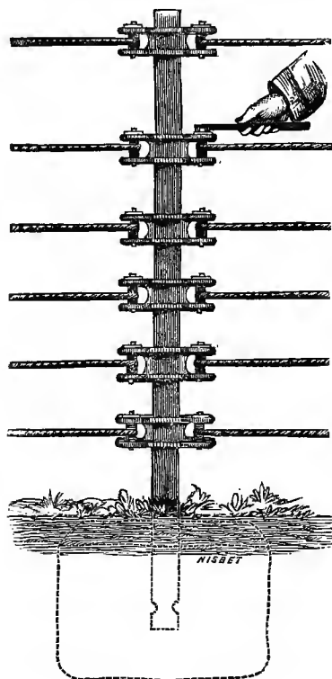
Fig. 583.—Winding-pillar.
