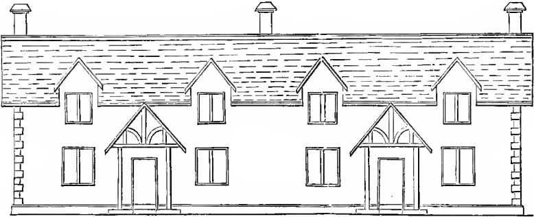
Fig. 754.—Front elevation of cottages in fig. 752.
