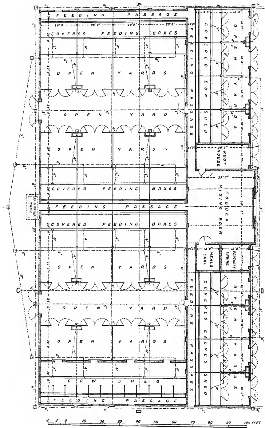
Fig. 681.—Ground-plan of complete steading for farm of 500 acres.
