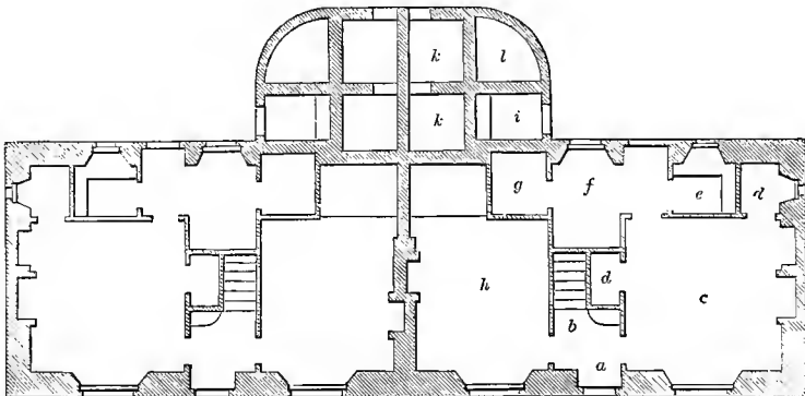
Fig. 752.—Ground-plan of two-story double-detached cottages.
