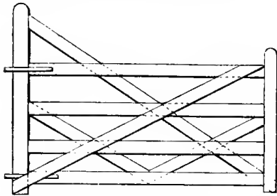
Fig. 603.—Strong field-gate.
