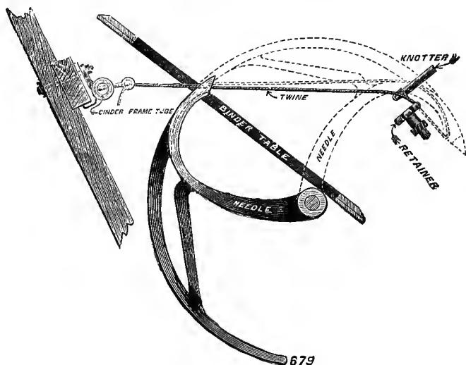
Fig. 510.—Needle.
