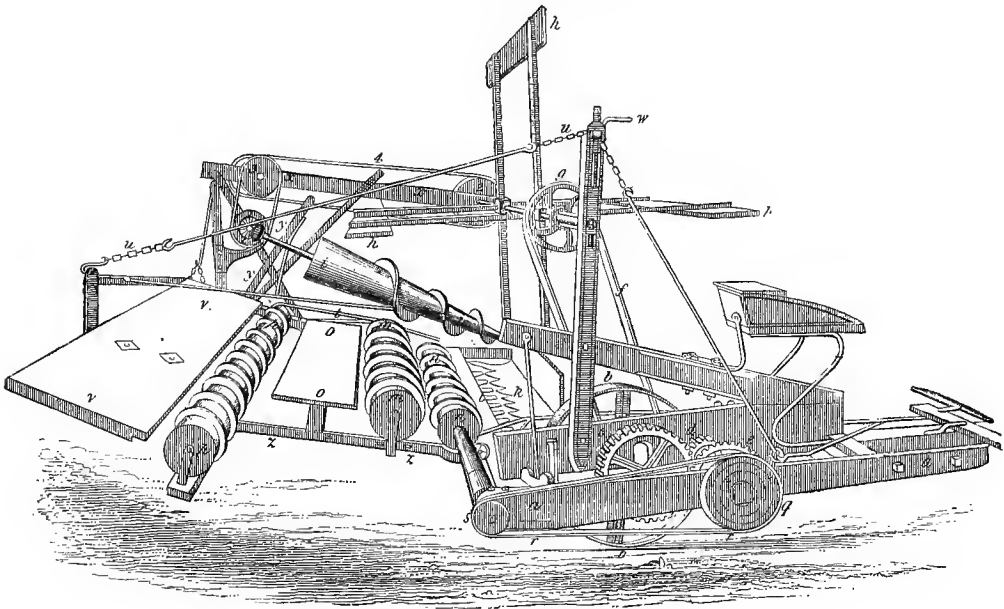
Fig. 498.—M'Cormick's reaping-machine.
