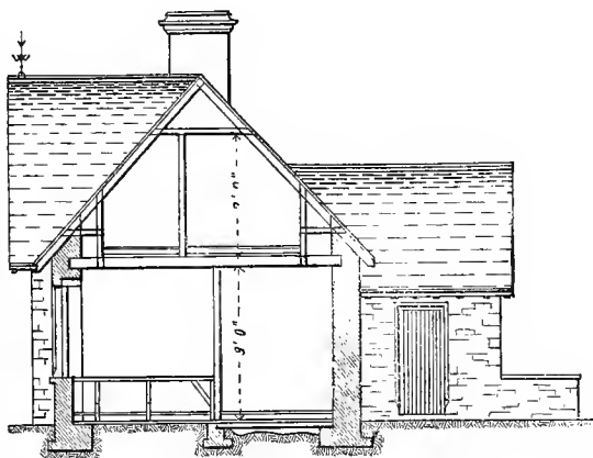
Fig. 757.—Section.
