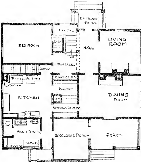
FLOOR PLAN FOR FARMHOUSE.
