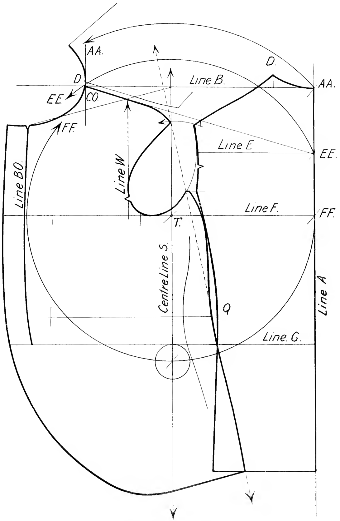
PROOF DRAFT OF FOUNDATION.
