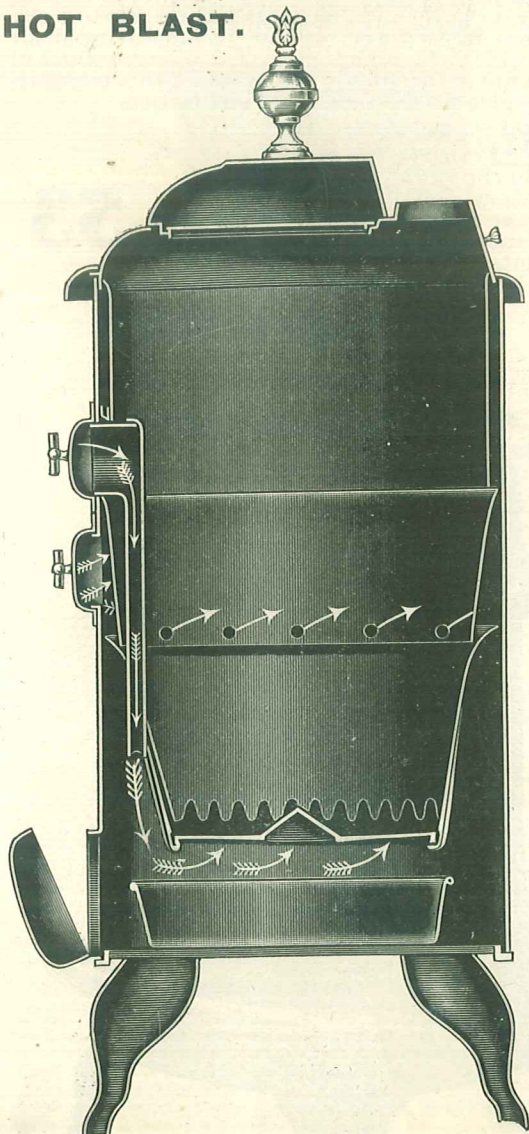
Skeleton illustration showing inner construction of Acme Hotspur.
