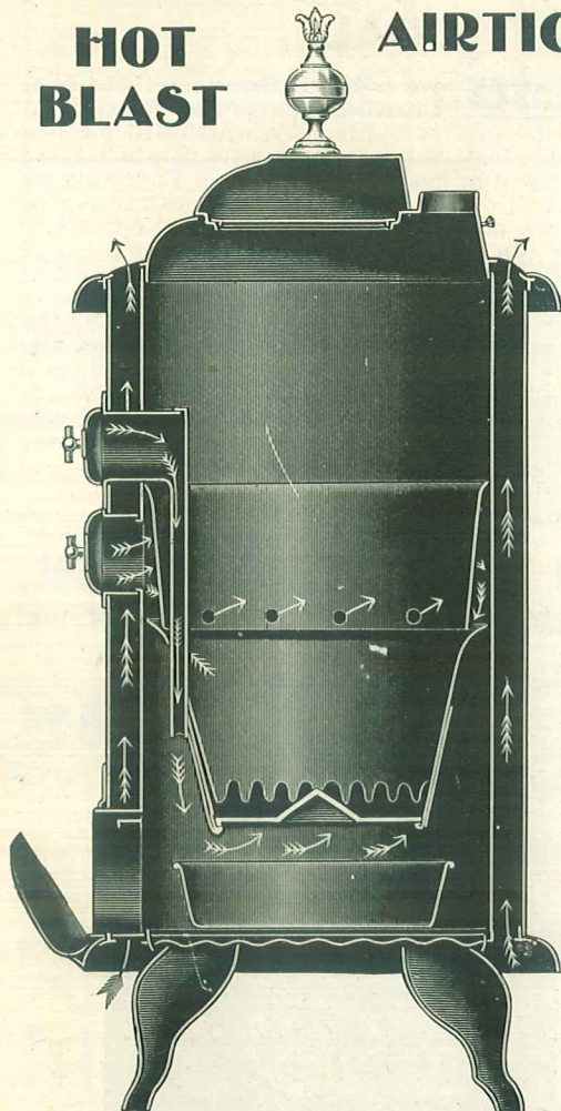
Skeleton illustration showing inner construction Hot Blast for Coal, with Hot Air Circulation.
