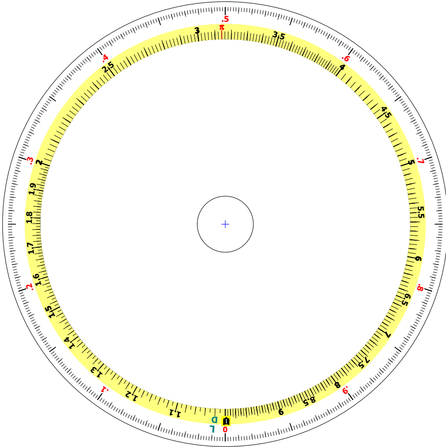
Stationary Disc
