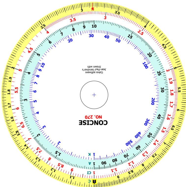
Movable Disc
