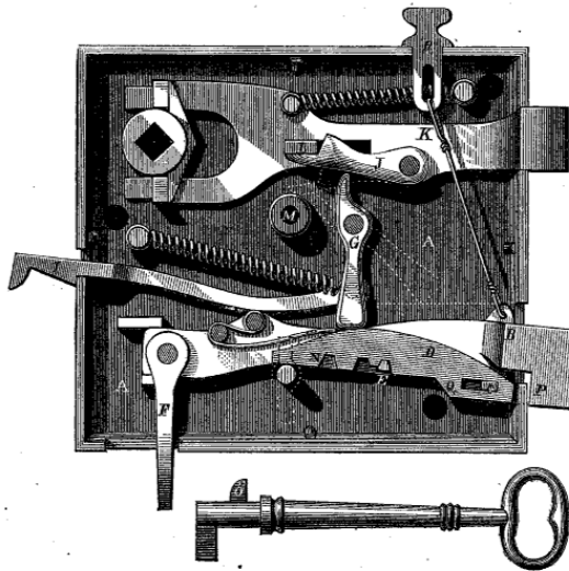
MILLER'S COMBINED BOLT AND LOCK.
