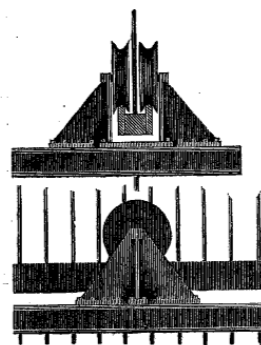
THE PULLEYS.
