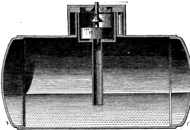
COCHRANE'S LOW-WATER STEAM PORT.
