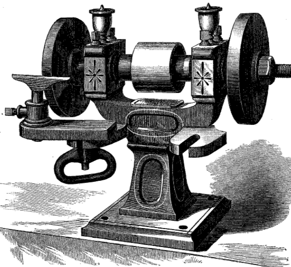
IMPROVED EMERY WHEEL GRINDING MACHINE.
