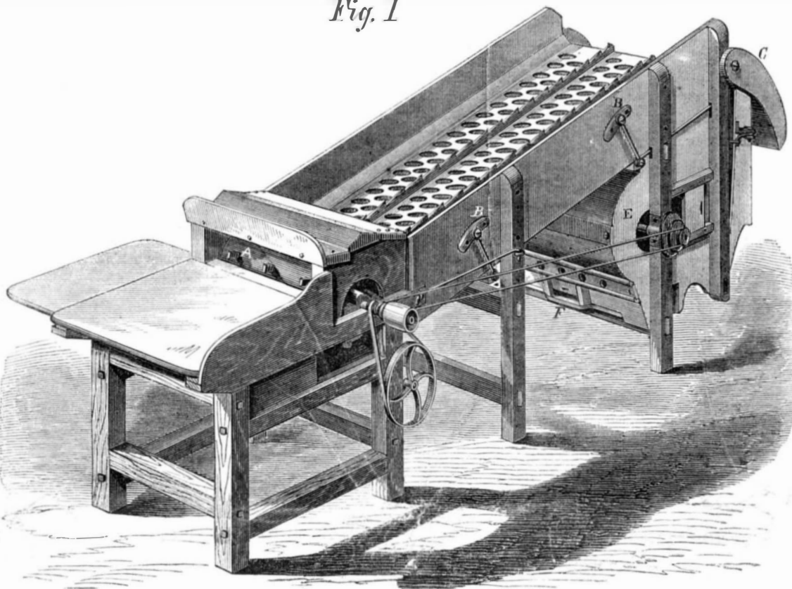
SEIP & SCHMEIER'S COMBINED THRASHER AND FANNING MILL.
