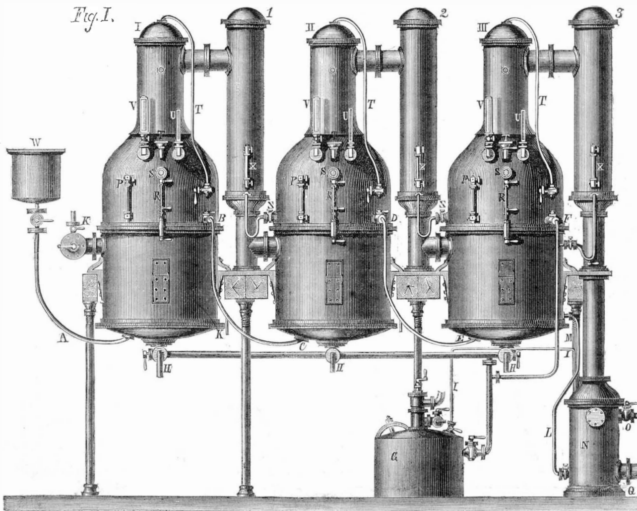
ROBERT'S TRIPLE-EFFECT VACUUM PAN.
