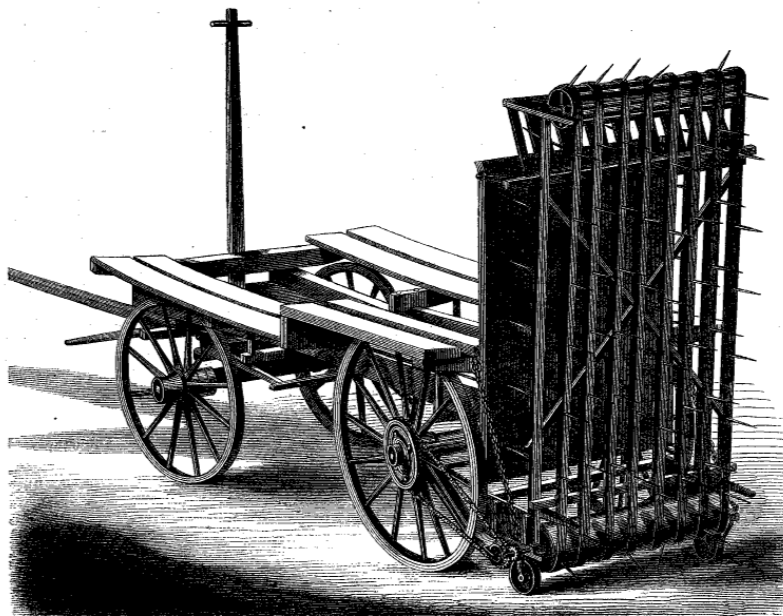
DOUGLAS' PATENT HAY LOADER.
