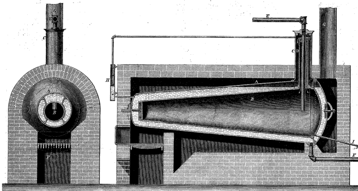
THE GERNER PATENT BOILER.
