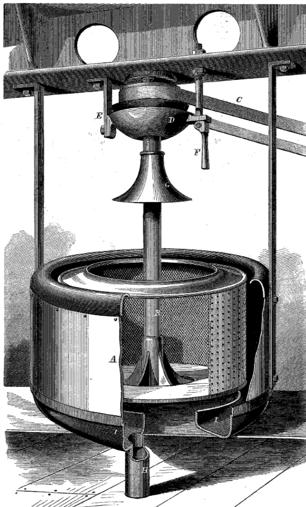
WESTON'S PATENT IMPROVED CENTRIFUGAL.
