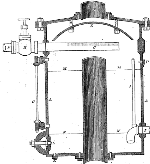
WATERS' FEED-WATER HEATER.
