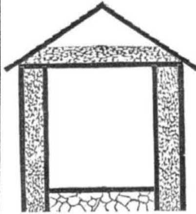
Section of an Ice-house above Ground.
