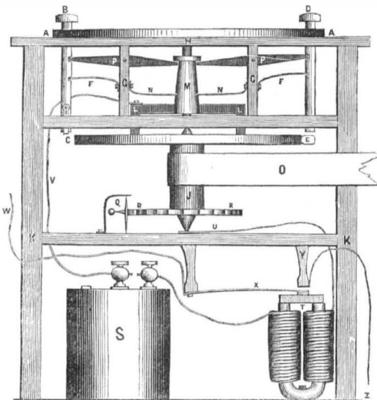
LETTER PRINTING TELEGRAPH.—Figure 1.
