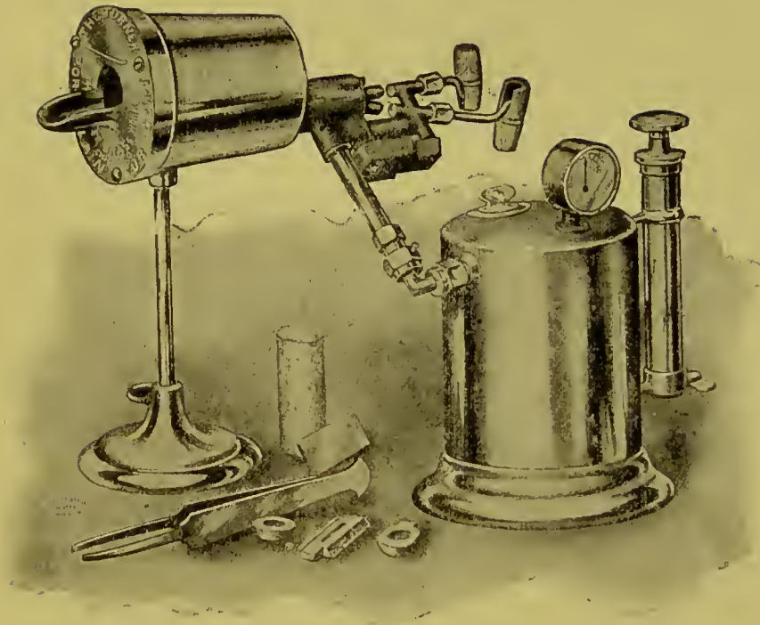
TURNER GASOLINE FURNACE No. 140
