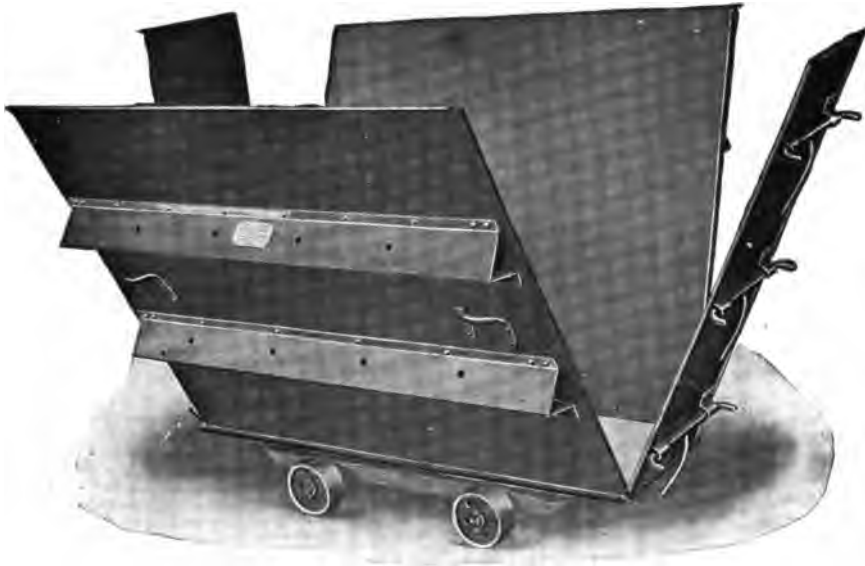
FIG. 78.—Soap-frame.
