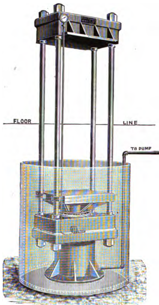
FIG. 169.—Cold-press.
