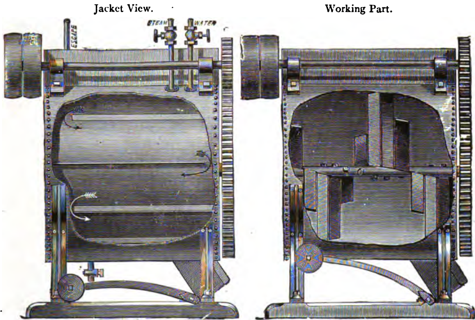
FIG. 66.—Strunz Crutcher.
