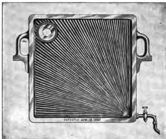
FIG. 32.—Filter-press Plate.
