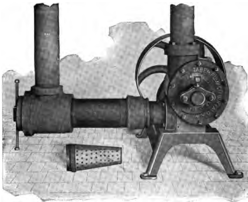
FIG. 62.—Soap-pump with Strainer Attached.
