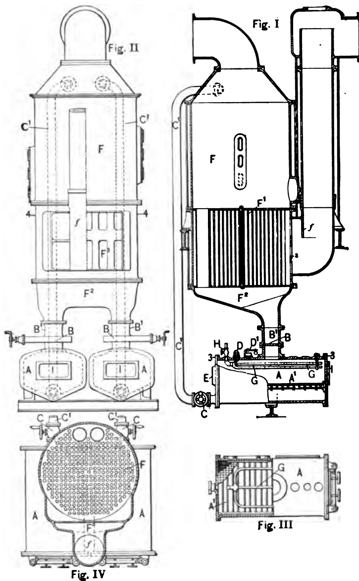
FIG. 240.—Foster Waste Soap Lye Evaporator.
