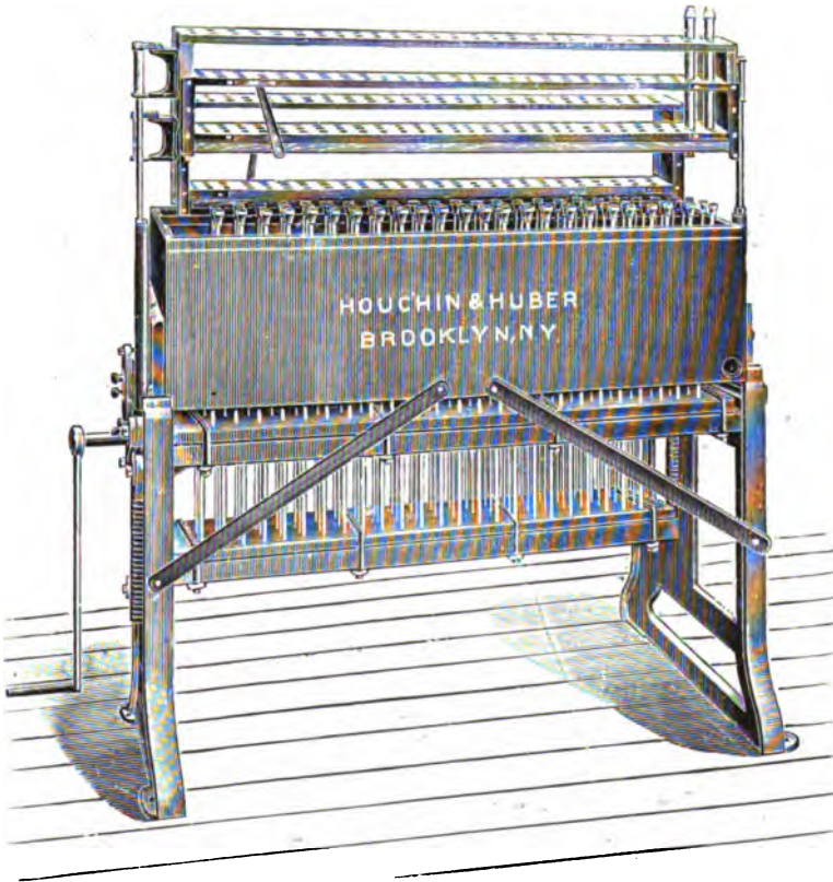
FIG. 200.—144-mould Self-fitting End Candle-machine.
