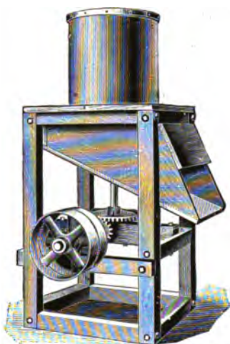
FIG. 127.—Slab-chipper.
