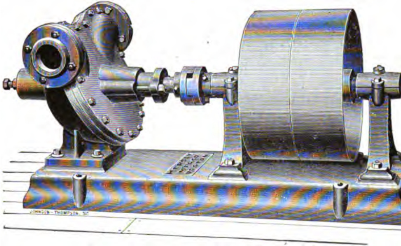
FIG. 54.—Hersey Rotary Pump.
