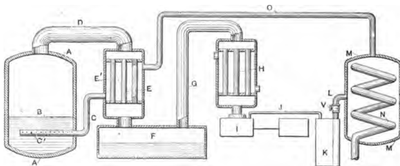
FIG. 220.—Diagram of Garrigues System for the Production and Distillation of Crude Glycerin.
