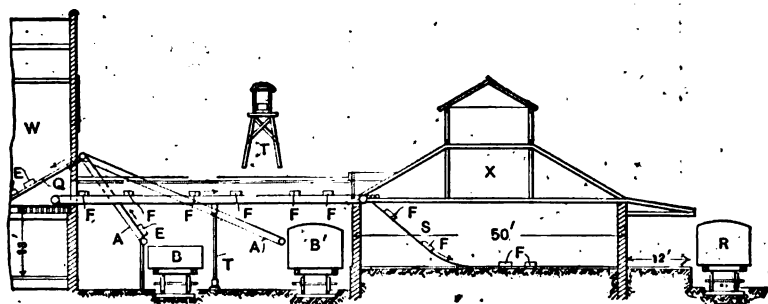
FIG. 118.—Box Conveyers.
