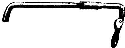
FIG. 75.—Adjustable Clamp for Soap-frame.
