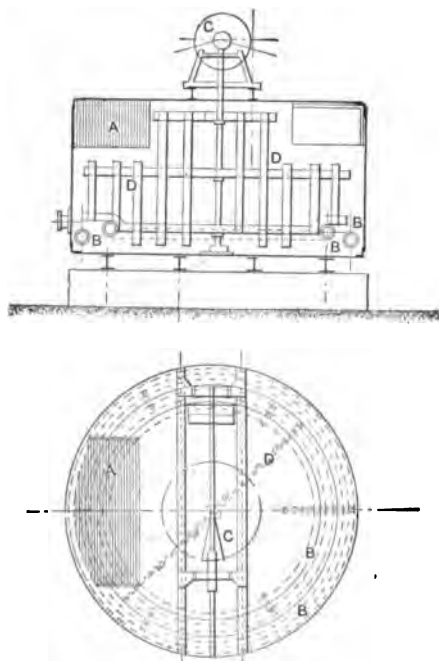
FIG. 28.—Soda-ash Dissolving-tank.
