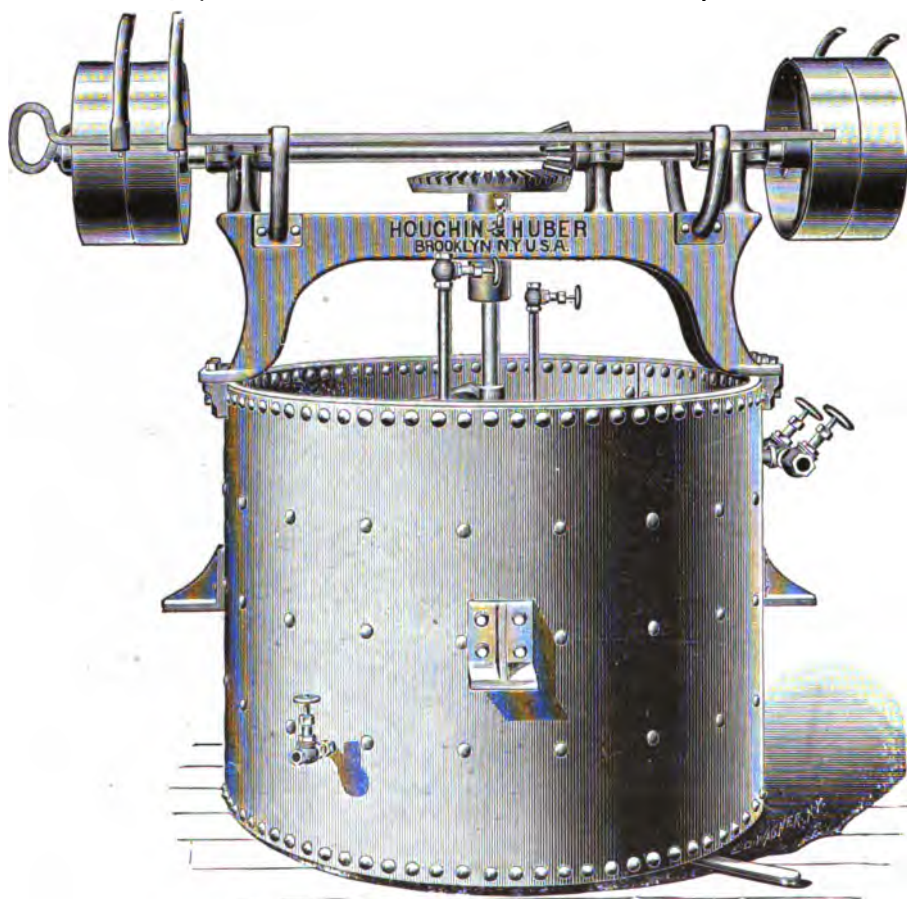
FIG. 67.—Soap-crutcher, Belt-driven.
