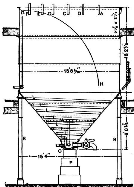
FIG. 43.—Soap-kettle, Cone Bottom.
