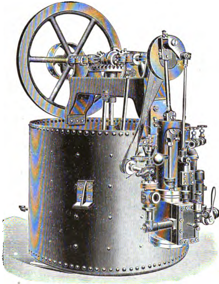
FIG. 68.—Soap-crutcher, Driven by Direct-connected Engine.
