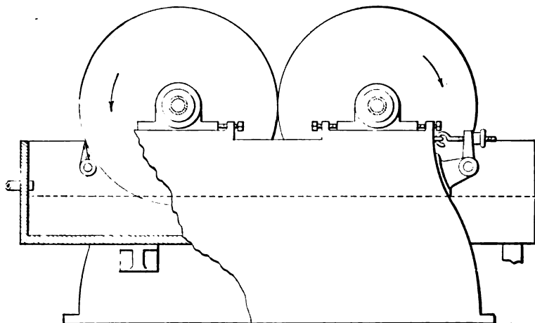
FIG. 206.—Double-roll Film Evaporator.
