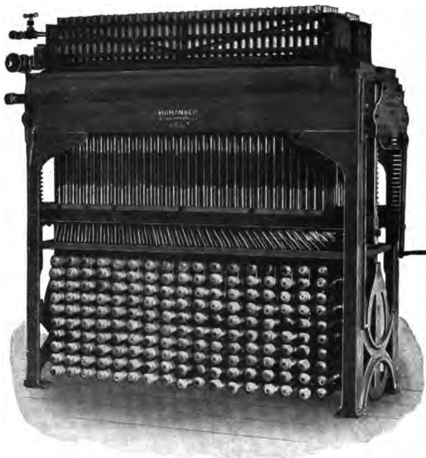
FIG. 189.—A 360-mould Candle-machine.
