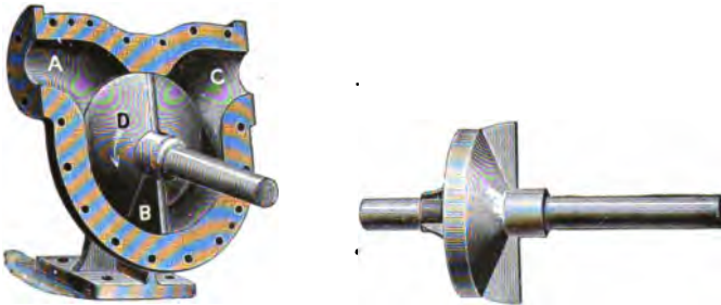
FIG. 55.—Working Parts of Hersey Rotary Pump.
