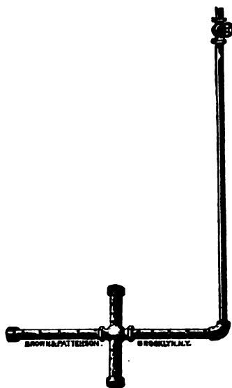
FIG. 47.—Criss-cross for Open Steam.
