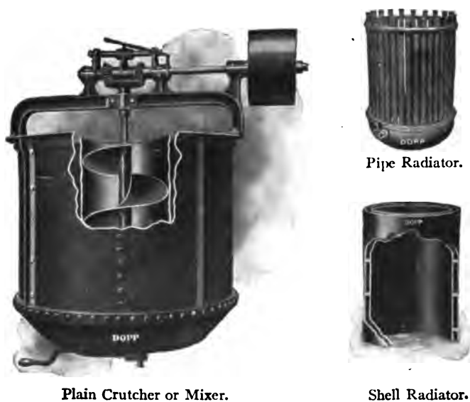
FIG. 69.—Crutchers.
