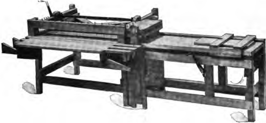
FIG. 87.—Ralston Cutting-table, with Hand-spreader.
