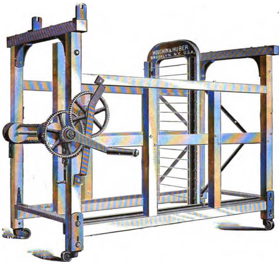
FIG. 83.—Champion Soap-slabber.
