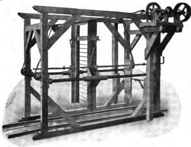
FIG. 85.—Automatic Power-slabber.
