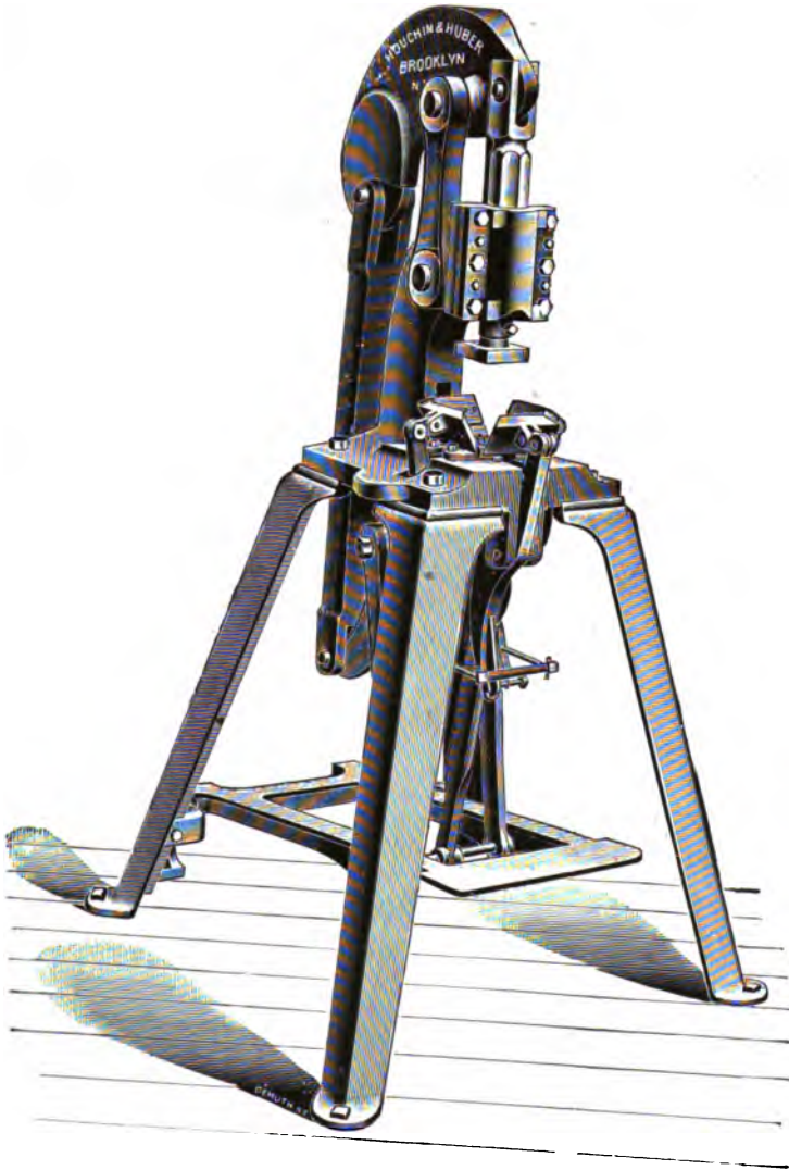
FIG. 105.—Foot-power Press for Impressions on all Sides of Cake.
