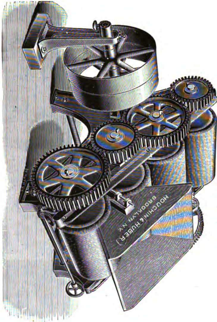
FIG. 156.—Four-roll Mill.
