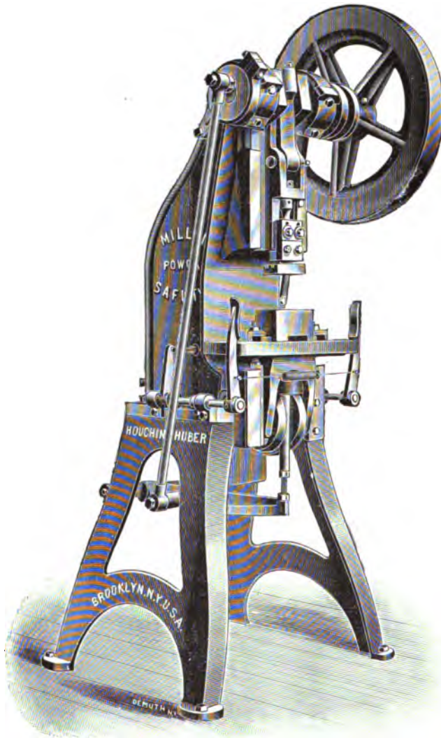
FIG. 111.—The Miller Safety Automatic Power-press.
