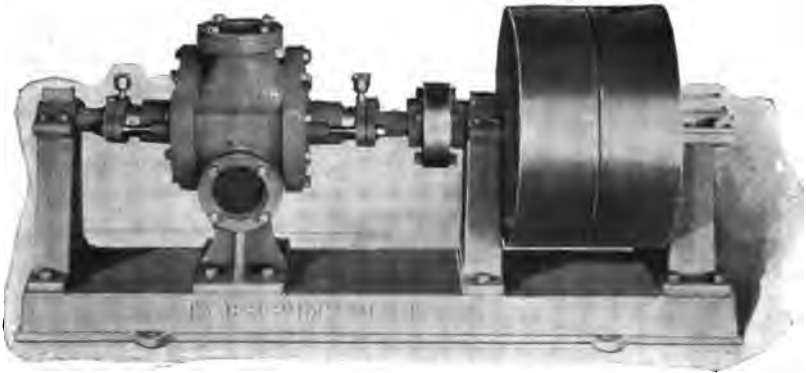
FIG. 57.—Taber Rotary Pump.
