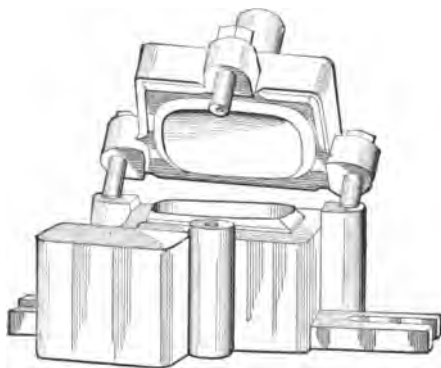
FIG. 114.—Combination Box and Pin-and-shoulder Die.
