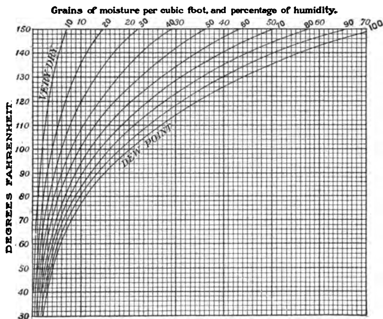
FIG. 96.—Hygrometric Chart.
