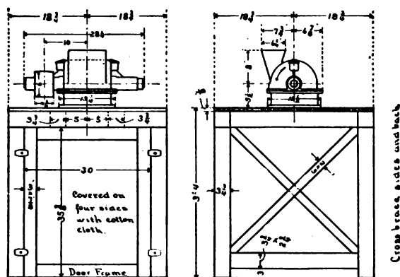
FIG. 141.—Diagram for Setting up Mill to Discharge into Barrels.
