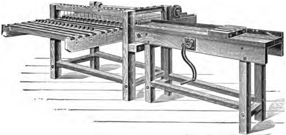
FIG. 88.—Cutting-table, with Automatic Spreader.
