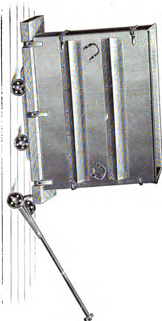
Fig. 76.—Device for Moving Frame, as applied.
