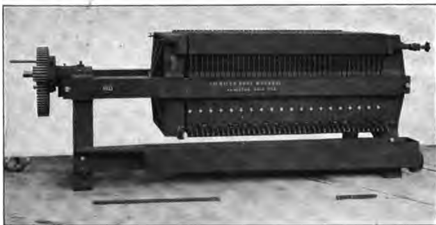
FIG. 36.—Filter-press with Steel Panel Plates.
