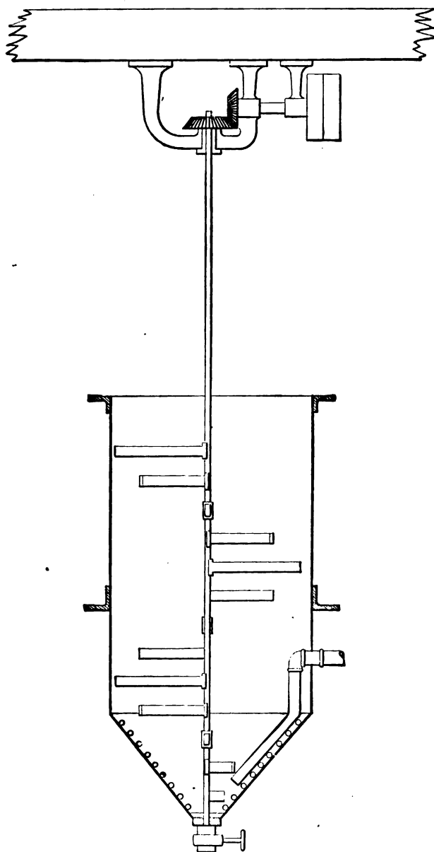
FIG. 12.—Lard-refining Kettle.
