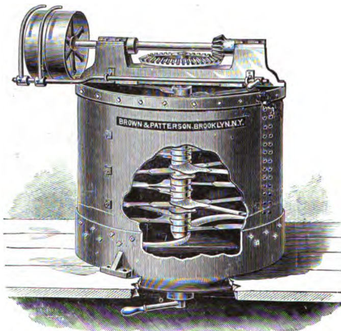
FIG. 65.—Soap-crutcher.
