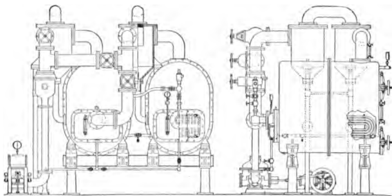
FIG. 217.—Garrigues Double-effect Evaporator, Convertible into Two Single-effects.
