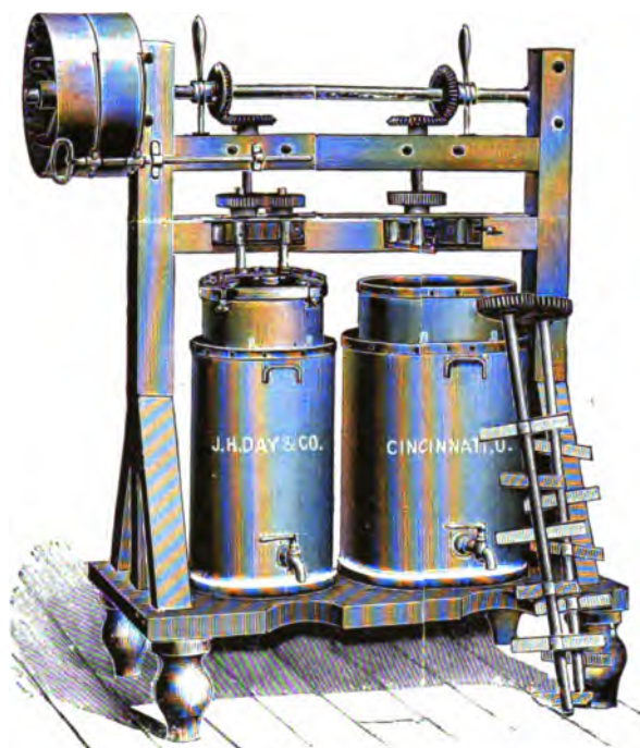
FIG. 145.—Pomade-washer.
