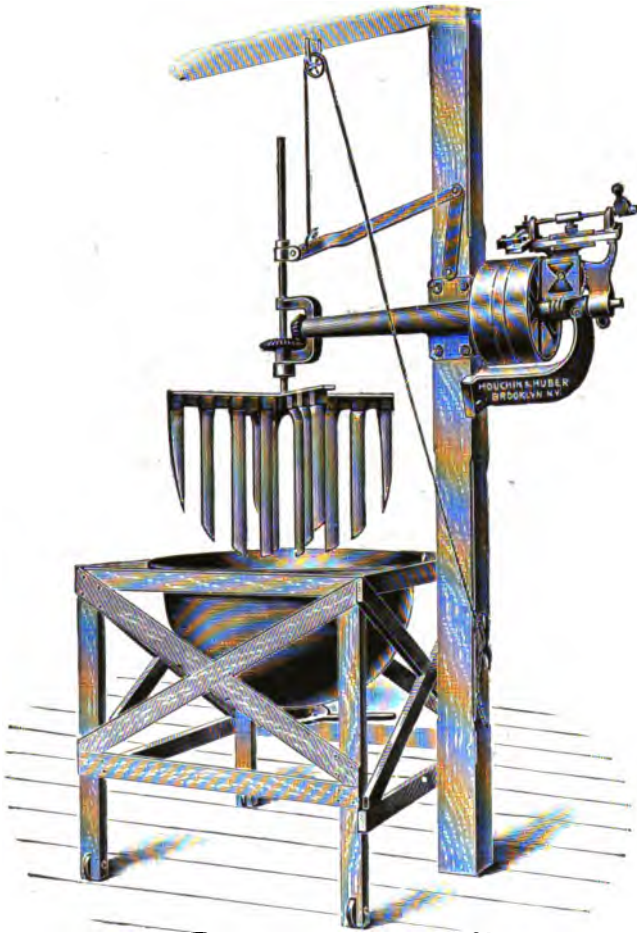
FIG. 124.—Cold-process Soap-mixer.
