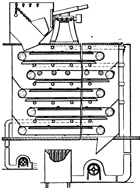
FIG. 128.—Chipper and Continuous-drying Device.
