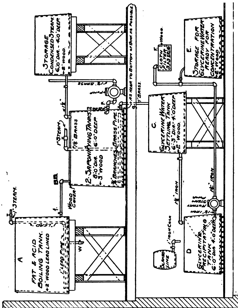
FIG. 174.—Apparatus for Saponifying 50,000 Pounds of Stock per Week. Twitchell process.
