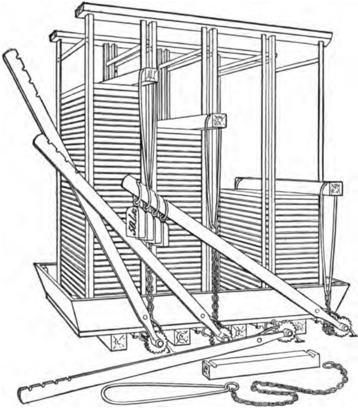
FIG. 10.—Lever Lard-press.
