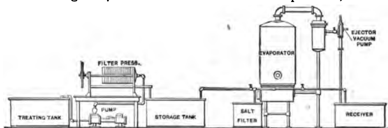
FIG. 207.—Crude Glycerin Plant with Steam-jacketed Evaporator.
