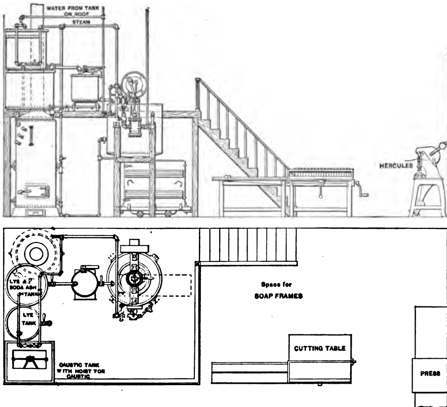
FIG. 122.—Plant for Cold-process Soap.
