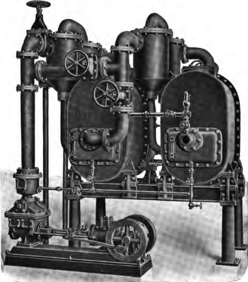
FIG. 219.—Rear View of Double-effect, Convertible, Vacuum Evaporator.
