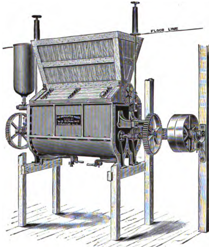
FIG. 138.—Soap-powder Mixer.
