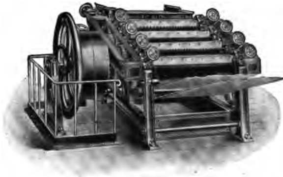
FIG. 154.—Eight-roll Toilet-soap Mill.
