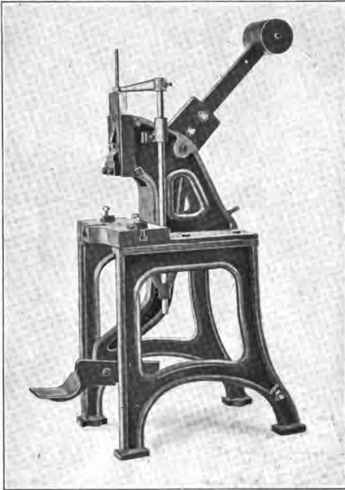
FIG. 102.—Foot-power Soap-press.
