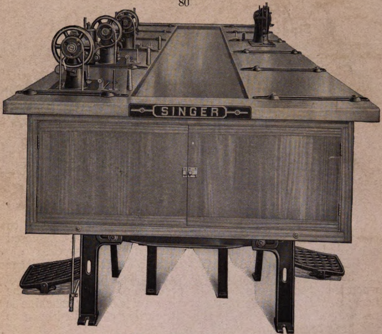
End View Showing Doors Closed
