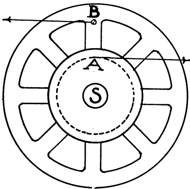
Balance Wheel
