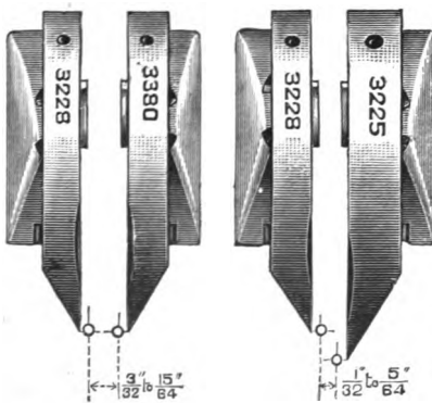
Shuttles for Different Gauges on Two-Needle Machines
