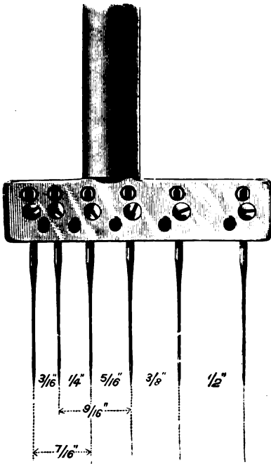
Spacing of Needles on Singer Machine No. 41-6
