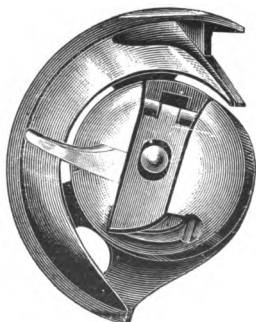
Oscillating Shuttle and Central Bobbin in its case
