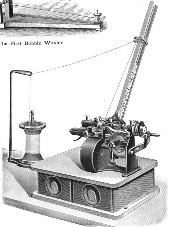
Singer Self-Feeding Bobbin Winder No. 27738
