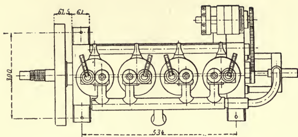
FIG. 73.—Wright Motor.
