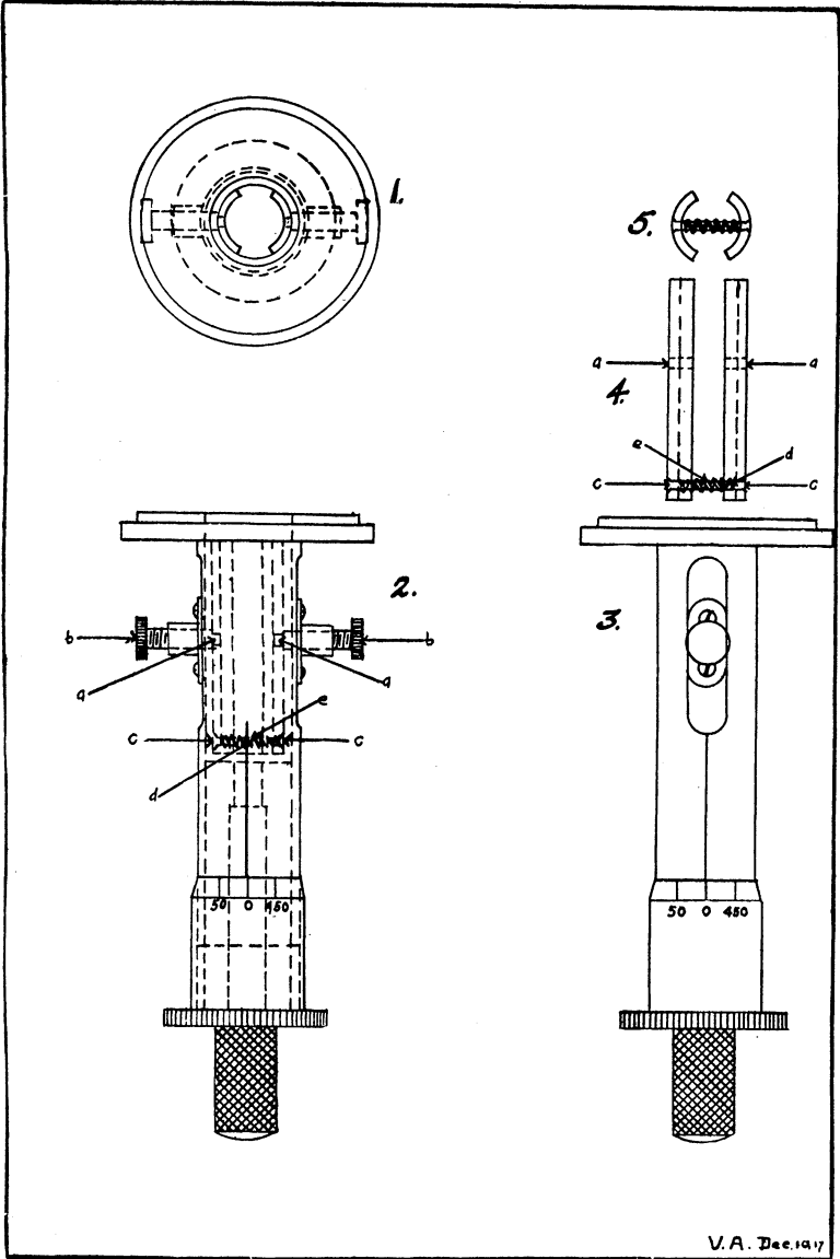
FIG. 1.—Modification of hand micrometer
