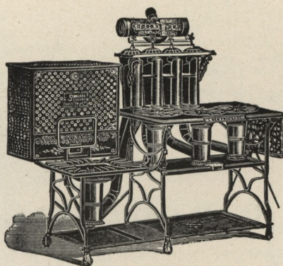
This cut represents our 1894 “NEW PROCESS” Step Stove.
