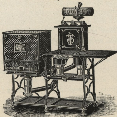
This cut represents our 1897-1898 “NEW PROCESS” Step Stove.
