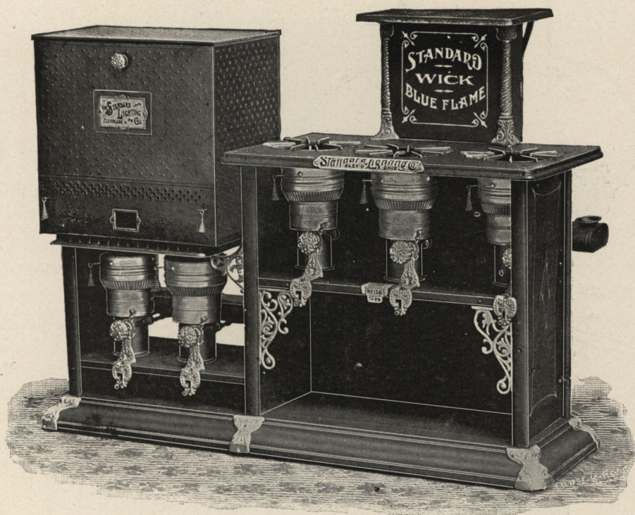
No. 106. "Standard" Wick Blue Flame Oil Stove. Price $24.00.
