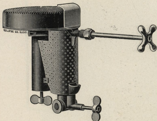
Cut shows "Standard" Giant Burner With Smokeless Lighter.
