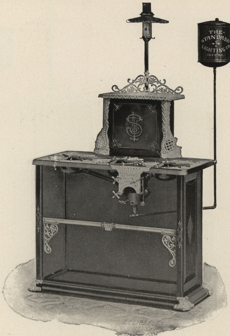
No. 521. "Standard" Ther-Lite Gasoline Stove.
