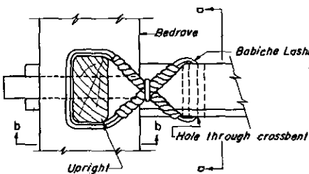
PLAN VIEW DETAIL AT C
