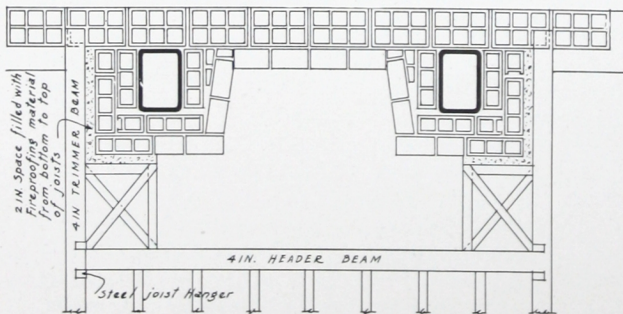
FIG. 32. APPROVED HOLLOW TILE CONSTRUCTION FOR FIREPLACES.
