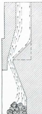
FIG. 26. THIS CONSTRUCTION WITHOUT A THROAT DAMPER OR SMOKE SHELF IS BAD. IT DIRECTS THE DOWN DRAFT SO THAT IT MEETS THE UP DRAFT ALMOST AT THE THROAT.
