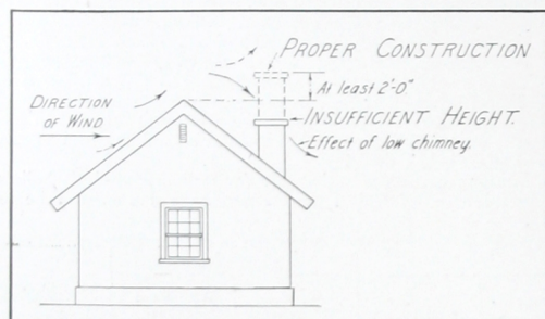
FIG. 9. TOP OF CHIMNEY SHOULD BE AT LEAST TWO FEET ABOVE THE TOP OF RIDGE IN ORDER THAT THE WIND CURRENTS MAY NOT BE DEFLECTED DOWN THE CHIMNEY.
