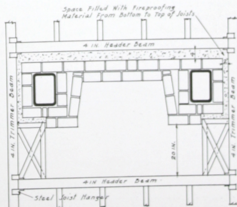
FIG. 30. FLOOR FRAMING AROUND A SINGLE FIREPLACE. NOTE FILLING BETWEEN FRAMING AND BRICKWORK, WHICH SERVES BOTH AS INSULATOR AND FIRE-STOP.
