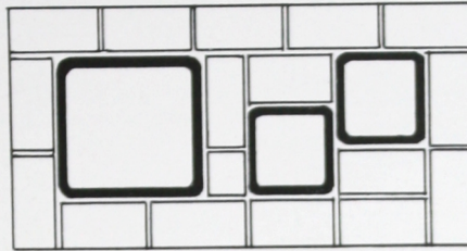
FIG. 11. CHIMNEY BUILT WITH TWO FLUES NOT DIVIDED BY "WITHE" BUT THIRD FLUE SEPARATED BY FOUR INCHES BRICK DIVISION WALL.
