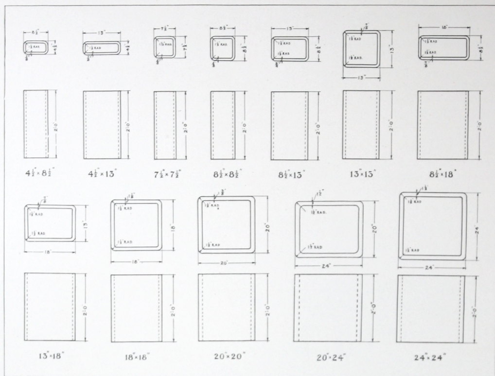
FIG. 5. STANDARD SIZES OF RECTANGULAR FIRE CLAY FLUE LININGS
