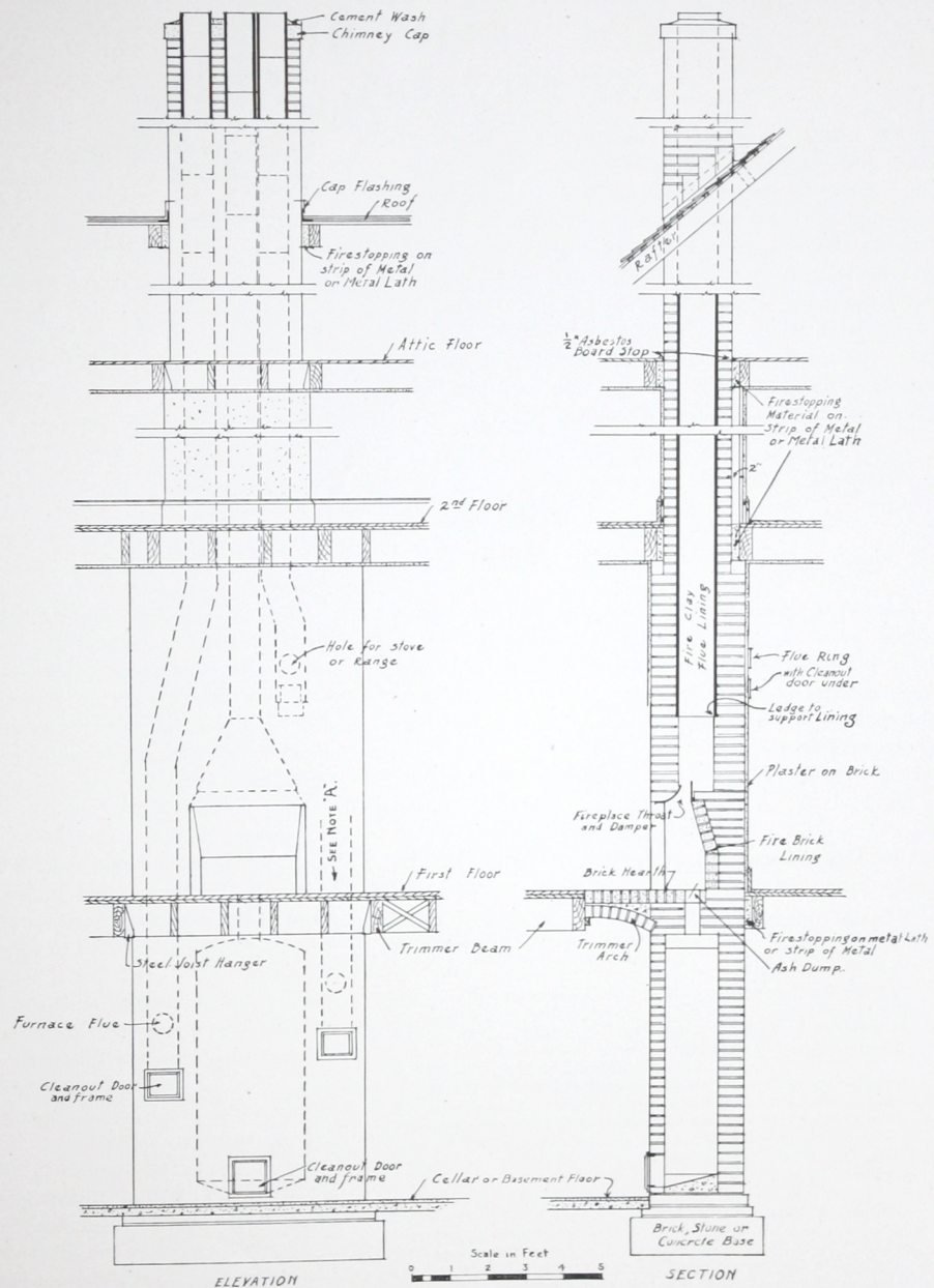
FIG. 34. ELEVATION AND SECTION OF AN INTERIOR INDEPENDENT CHIMNEY SHOWING RECOMMENDED CONSTRUCTION. NOTE A. —IT IS RECOMMENDED THAT AN EXTRA FLUE ALWAYS BE BUILT IN A CHIMNEY BREAST. THE MASONRY DISPLACED FROM THE CHIMNEY BREAST WILL PRACTICALLY PAY FOR THE COST OF THE LINING AND THE ONLY ADDITIONAL COST WILL BE FOR THE LINING AND BRICKWORK FOR THREE ADDITIONAL 4" WALLS SURROUNDING IT IN THE CHIMNEY ITSELF. SUCH A FLUE WILL BE FOUND INVALUABLE FOR DOMESTIC HOT WATER HEATER, LAUNDRY STOVE OR OTHER APPLIANCES NOT PERHAPS ORIGINALLY CONTEMPLATED.
