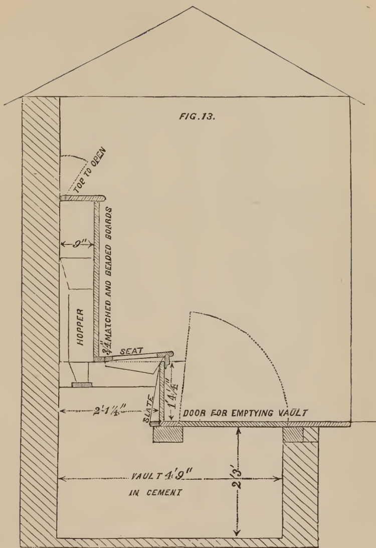
Section of Vaulted Privy showing Hopper filled and Vault emptied from Inside.
