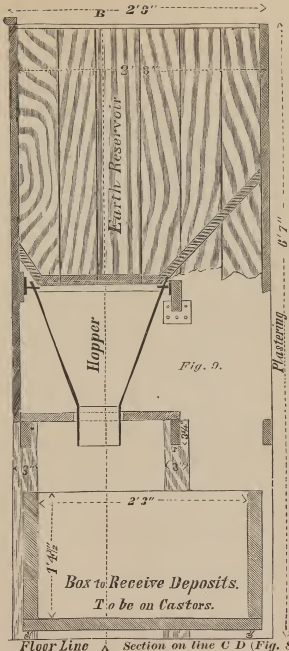
Section of Closet shown in Fig. 7.
