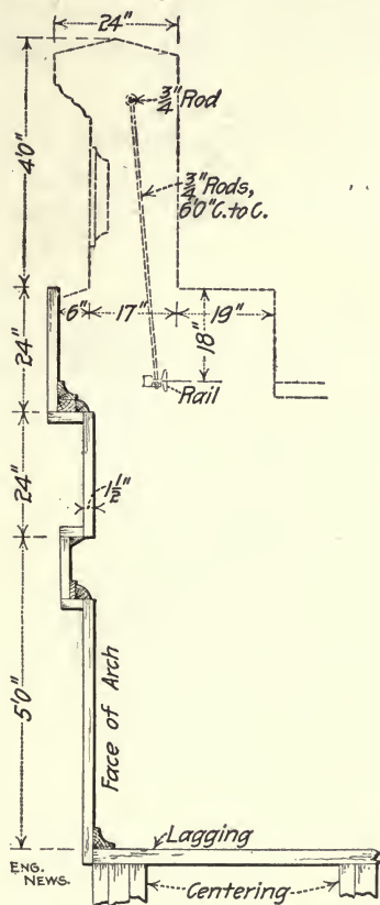
Fig. 293.—Spandrel Wall Mold for Arch Bridge.
