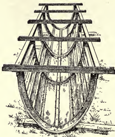
Fig. 263.—Invert Form for Sewer Construction.
