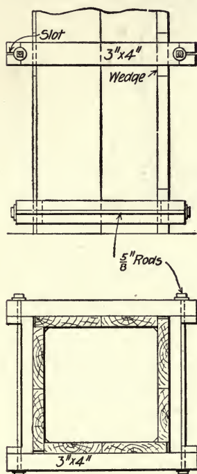
Fig. 178.—Form for Rectangular Column for Warehouse at St. Paul, Minn.
