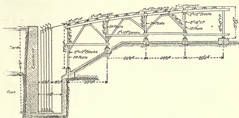
Fig. 254.—Section of Gas Holder Tank, New York City.
