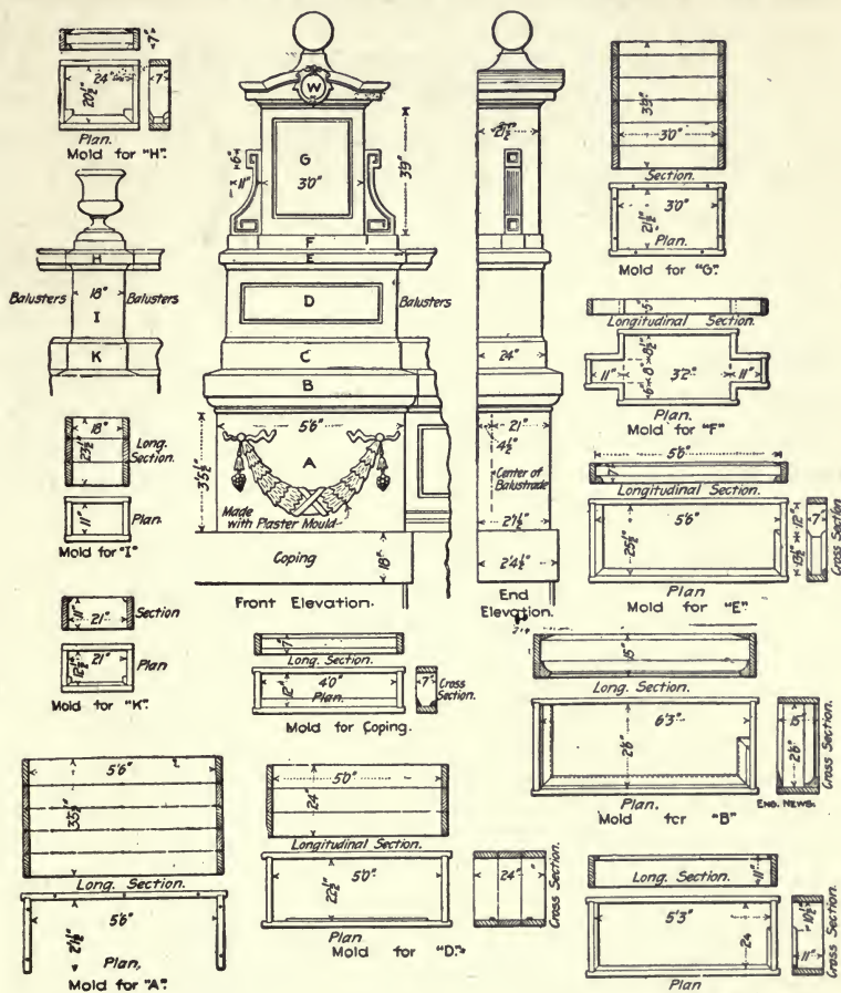
Fig. 289.—Molds for Ornamental Railing Posts for Concrete Facade for Bridge.
