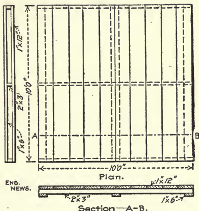
Fig. 44.—Portable Wooden Panels for Covering Floors.
