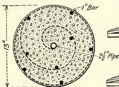
Fig. 65.—Cross-Section of Chenoweth Rolled Pile.
