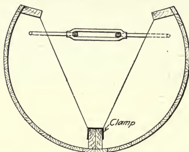
Fig. 249.—Invert Form for Conduit Construction.
