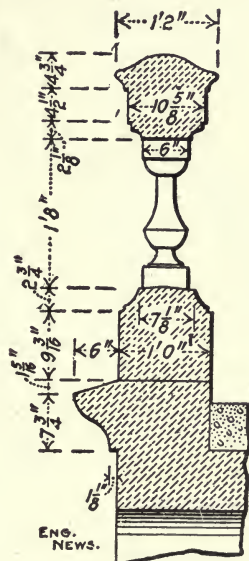
Fig. 302.—Cornice and Balustrade for Arch Bridge.
