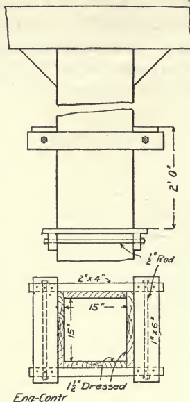
Fig. 226.—Column Form for 6-Story Building.
