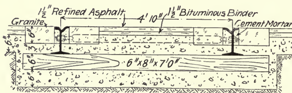
Fig. 114.—Concrete Foundation for Street Railway Track.
