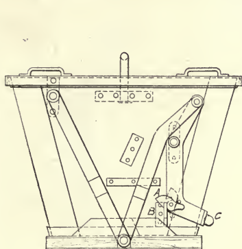
Fig. 29.—Stuebner Bucket for Depositing Concrete Under Water (Closed Position).
