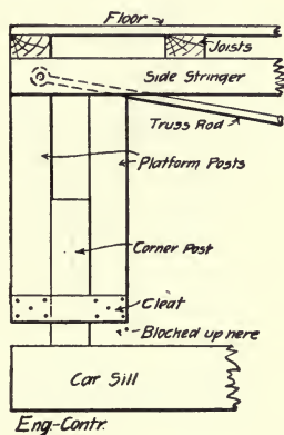
Fig. 141.—Sketch Showing Telescope Support for Concreting Platform, Burton Tunnel.
