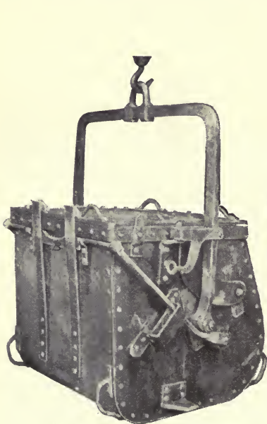
Fig. 27.—Cyclopean Bucket for Depositing Concrete Under Water (Closed Position).
