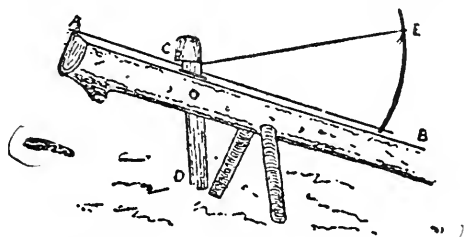
Fig. 53.—Shaving Horse
