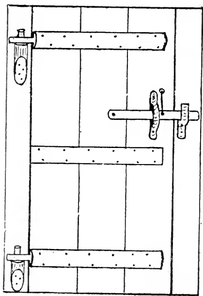
Fig. 77.—Cabin door (wooden hinges and latch)
