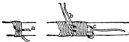
Fig. 165. Rod Winding.
