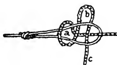
Fig. 170. Tiller Hitch.
