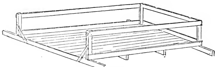
Fig. 17.—Tent Floor, with Wall Rail, Base-board, and End Joists Projecting that Corner Stakes May Be Nailed to Them
