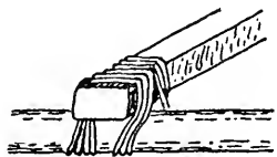
Fig. 159. Putlog Lashing.
