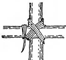
Fig. 158. Ledger Lashing.
