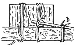
Fig. 162. Lever Knot
