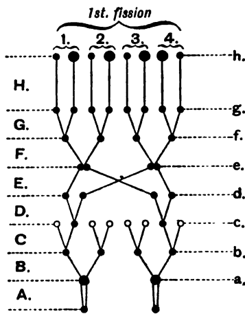
Colpidium colpoda (after Maupas).
