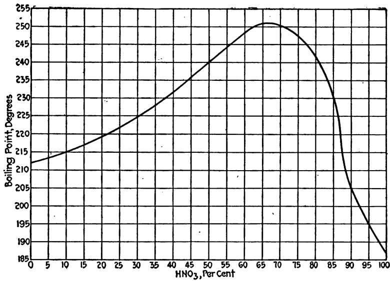
FIG. 83.—Boiling points of nitric acid.
