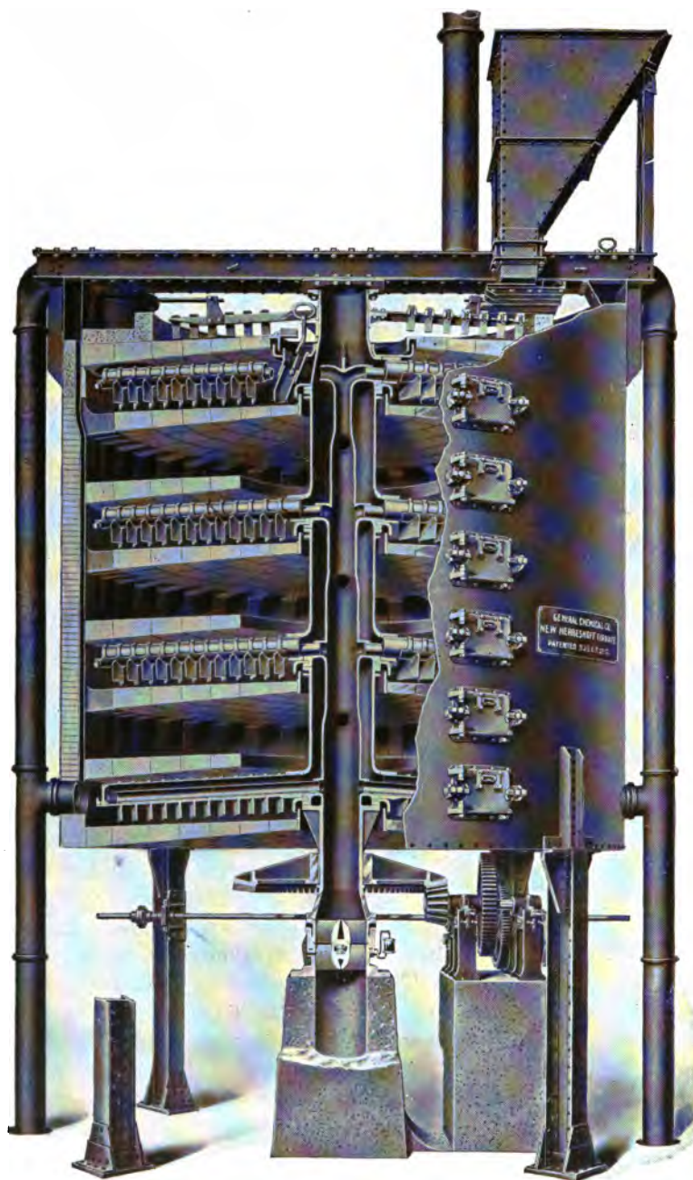
FIG. 6A.—Herreshoff furnaces.
