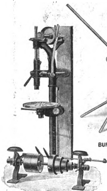
BUFFALO POWER DRILL, No. 87.
