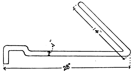
A HANDY DEVICE FOR THE ANVIL.
