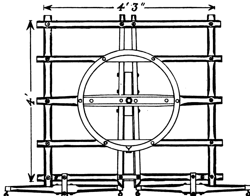
Fig. 8. PLAN OF GEAR. SCALE, 1 INCH EQUALS 18 INCHES.
