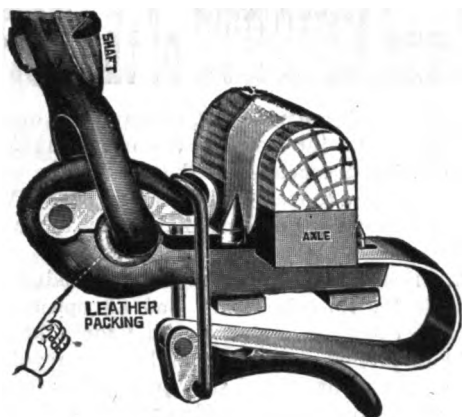
Coupling Closed
