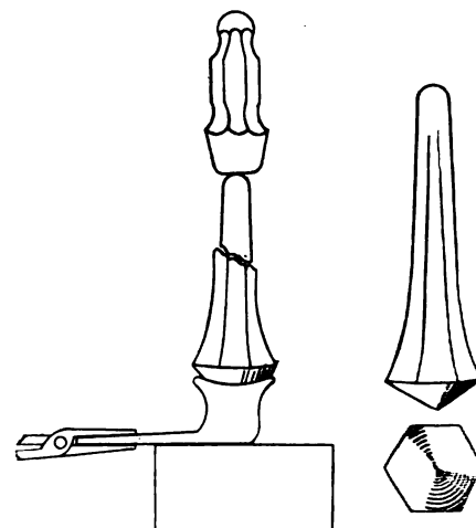
Fig. 3.—TOOL USED IN SHAPING GAFFS.
