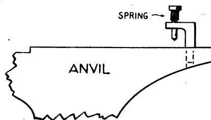
A USEFUL ANVIL PUNCH.
