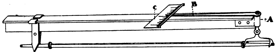
AN ACCURATE AXLE GAGE.
