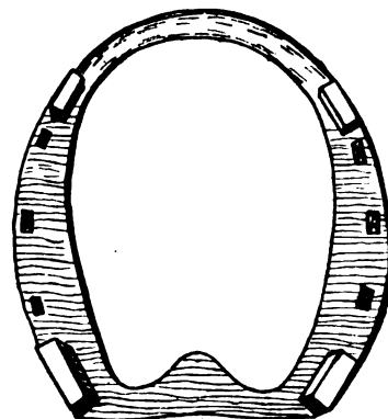
Fig. 15. B—HEEL WEIGHT BAR SHOE, WITH HALF ROUND ROLLER MOTION TOE.
