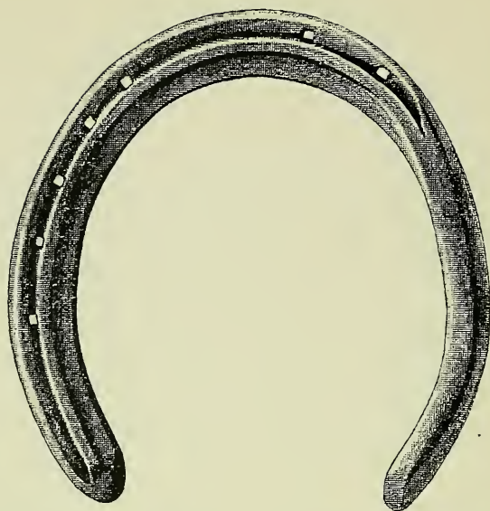
FIG. 294.—Fullered feather-edged concave fore shoe. Made from \frac{5}{8} \times \frac{3}{8} inch iron.
