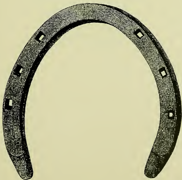
FIG. 223.—Charlier hind shoe, made from Charlier steel, \frac{7}{16} inch square.
