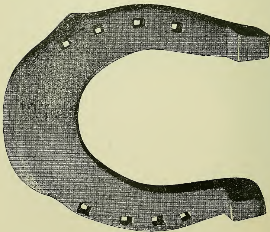
FIGS. 326, 327.—Stamped hind shoe (for cart horse). Made from 1\frac{1}{2} \times \frac{5}{8} inch iron.
