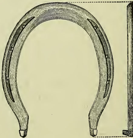
FIG. 229.—Steel hind shoe for trotter, one-third natural size. Weight, 5\frac{1}{4} ounces.
