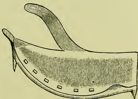
FIG. 401.—Voigtland shoe for oxen.
