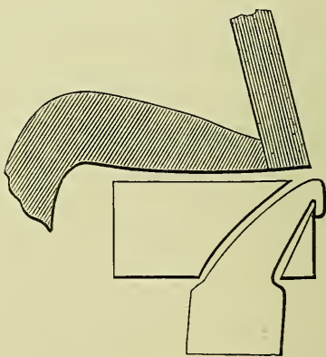
FIG. 108.—Section of shoe with Delp  rier's nail inserted.
