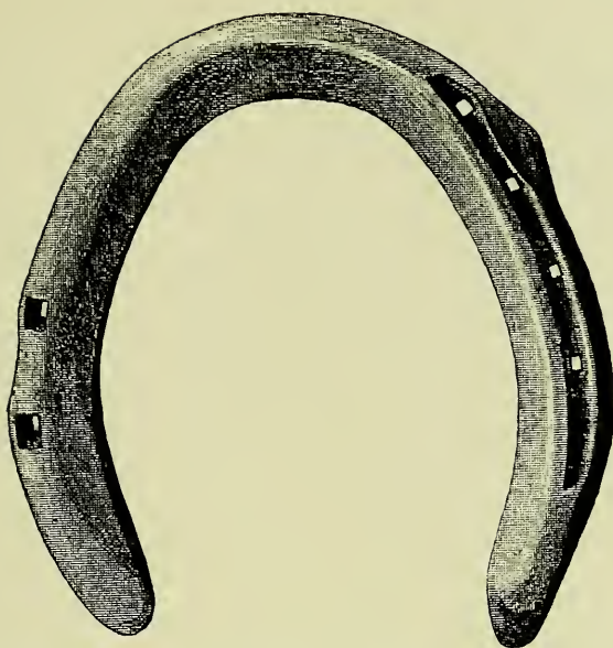
FIG. 220.—Concave partially-fullered hind shoe. Made in concave tool from \frac{3}{4} \times \frac{1}{2} inch iron or (preferably) from old shoes.
