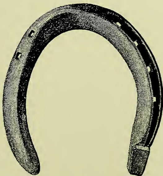
FIG. 221.—Concave partially-fullered hind shoe. Made of \frac{3}{4} \times \frac{1}{2} inch iron in concave tool.
