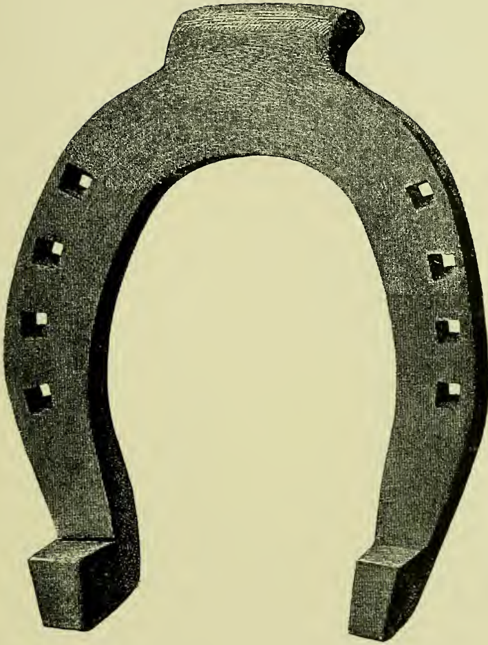
FIG. 328.—Stamped cart hind shoe, with toe-piece. Made from 1\frac{1}{4} \times \frac{5}{8} inch iron.
