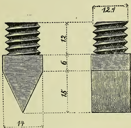
FIG. 115.—Screws (full size) provided with Whitworth thread.
