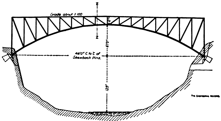
DRIVING PARK HIGHWAY BRIDGE, ROCHESTER.
