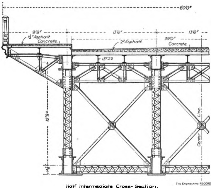
Half Intermediate Cross-Section.
