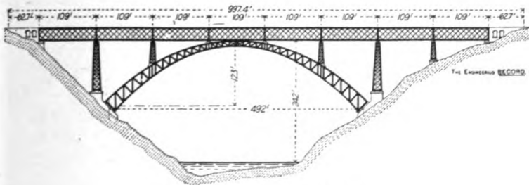
PADERNO VIADUCT, ITALY.
