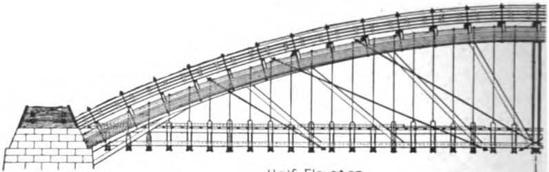
Half Elevation.
