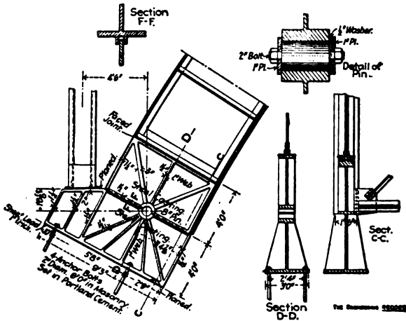
SKEWBACK HINGE AND PEDESTAL.
