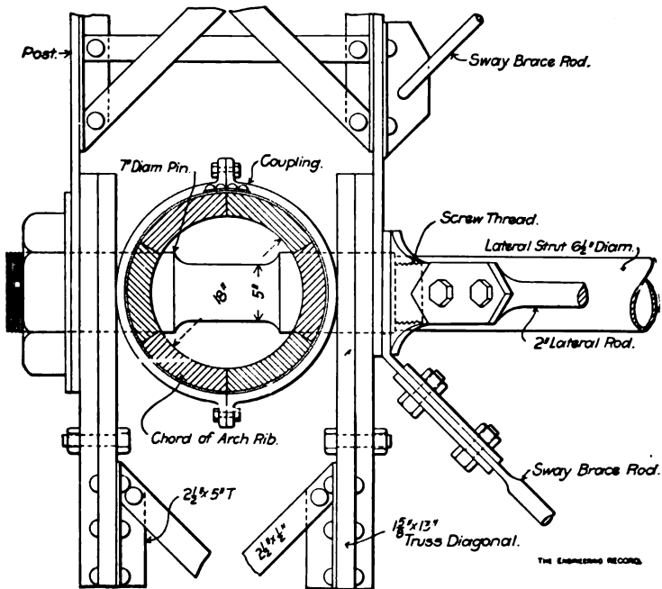
Sectional Elevation at Top Chord Panel Point.
