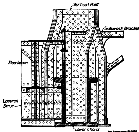
Connections at Foot of Portal.
