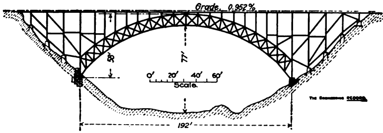
MENDOTA WOODEN ARCH.
