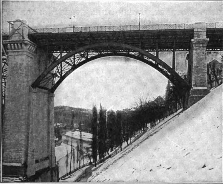
113½-FOOT SIDE SPAN OF CORNHOUSE BRIDGE, BERNE, SWITZERLAND.
