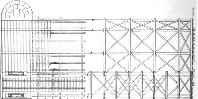
Half Plan.
