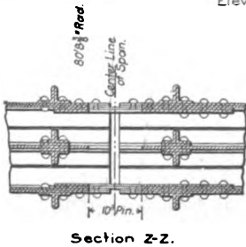
Grown Hinge connection.
