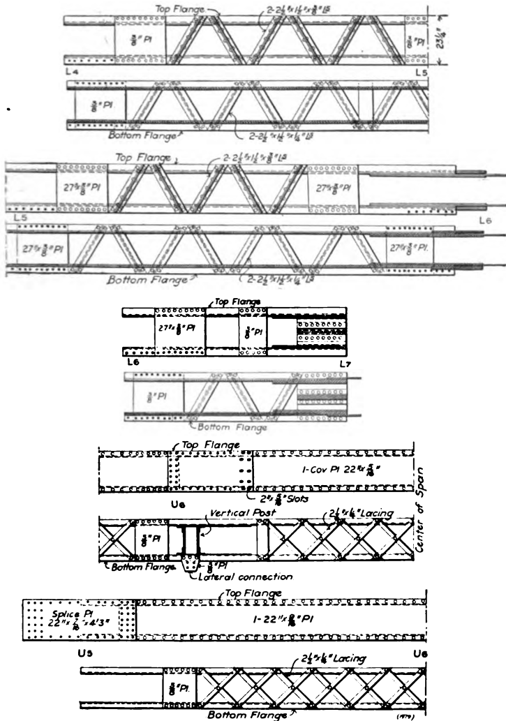
Top and Bottom Flanges of Chords.
