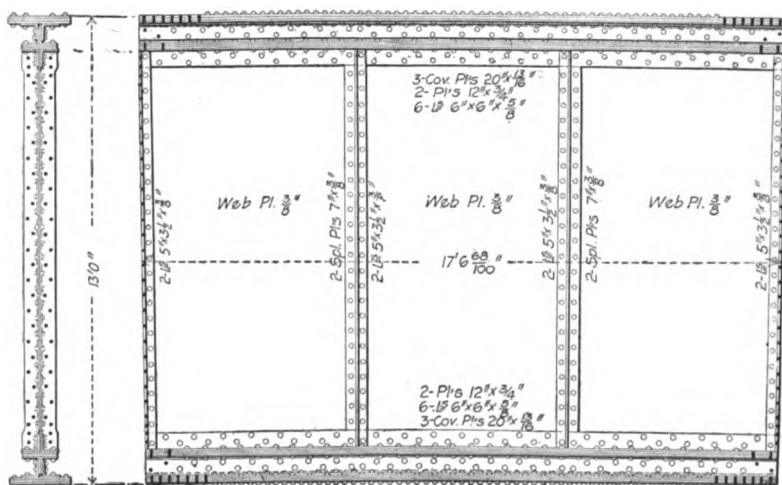
Intermediate Section of Arch Rib.
