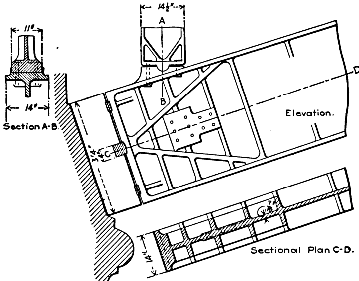
Skewback connections and Pedestal.
