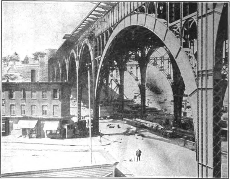
RIVERSIDE VIADUCT, NEW YORK, 128½ AND 65½-FOOT SPANS.
