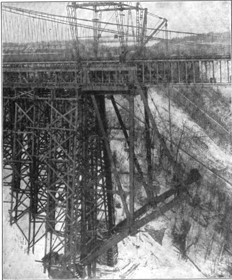
ERECTING SECOND PANEL OF ARCH TRUSS AS A CANTILEVER.
