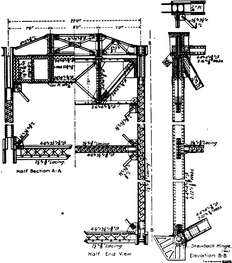
MENOMINEE BRIDGE.
