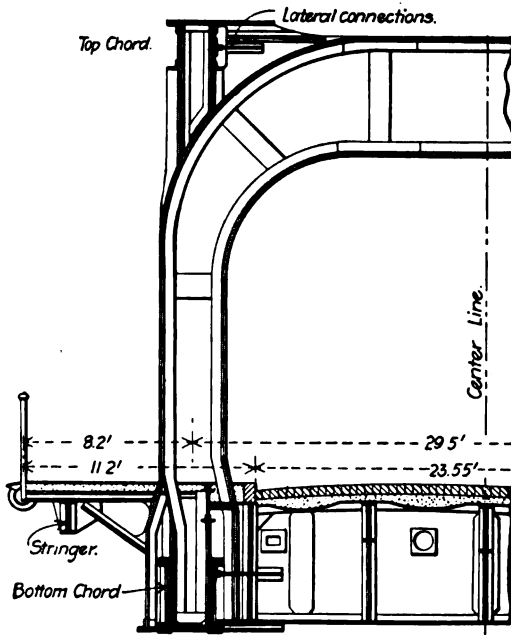
Portal at Panel No.3.
