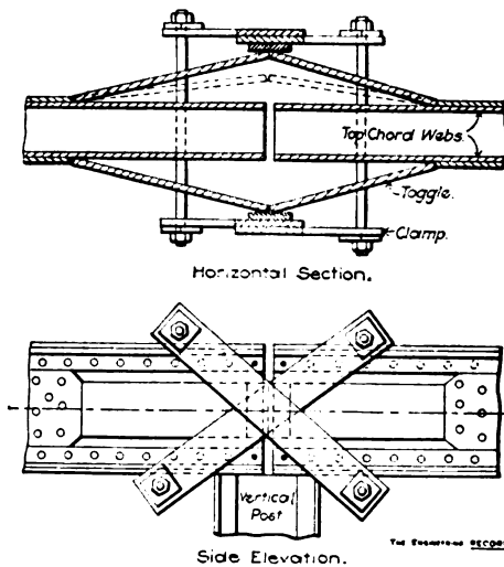
TEMPORARY ADJUSTMENT TOGGLE AT CROWN.
