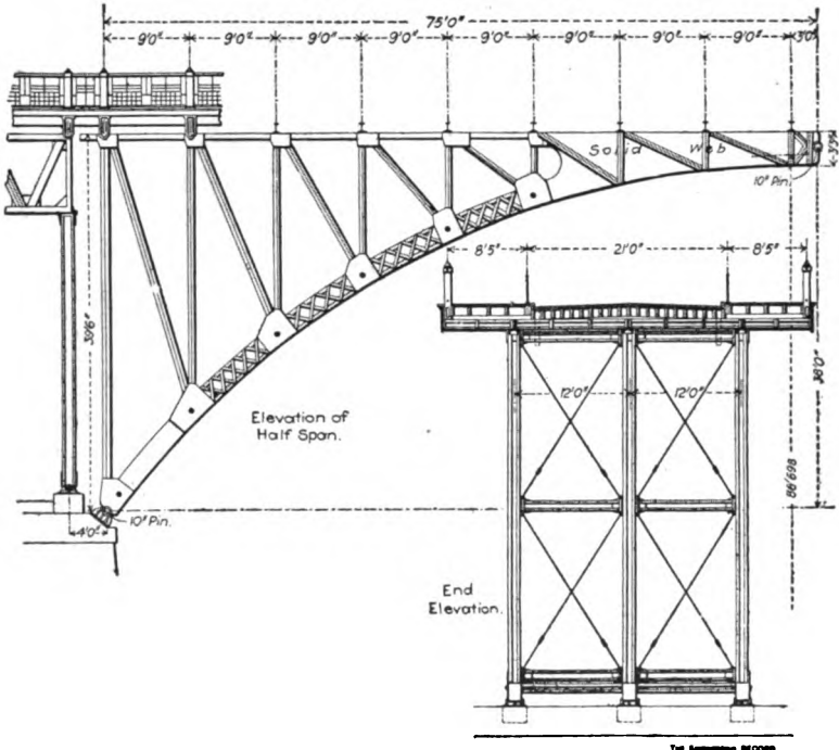
DRUID HILL PARK BRIDGE, CEDAR AVENUE, BALTIMORE.
