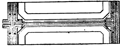
Section of Main Girder at Haunches. The Lanchester RECORD
