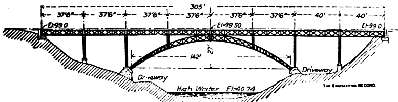
RIVERSIDE CEMETERY BRIDGE, CLEVELAND.
