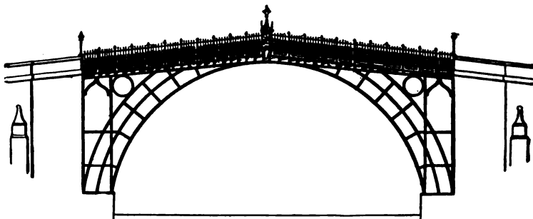
SEVERN RIVER 100-FOOT CAST-IRON SPAN.
