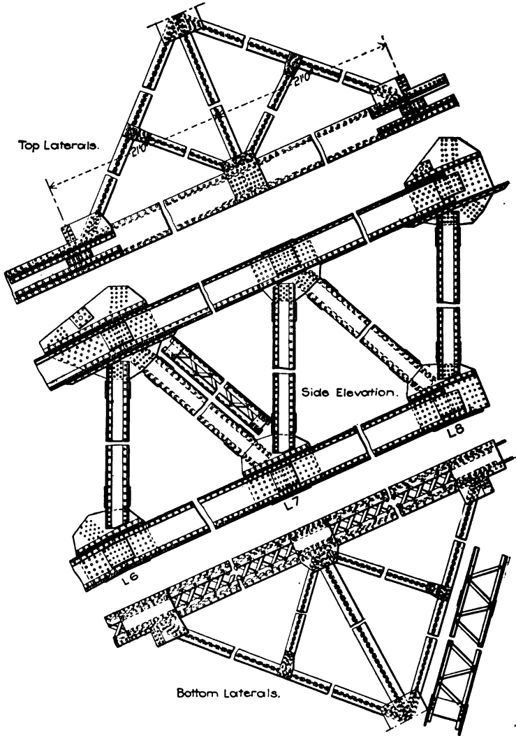
Intermediate Panels of Main Truss and Laterals.
