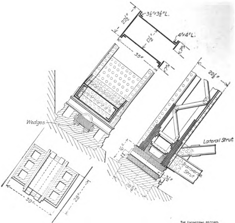
SKEWBACK CONNECTIONS.
