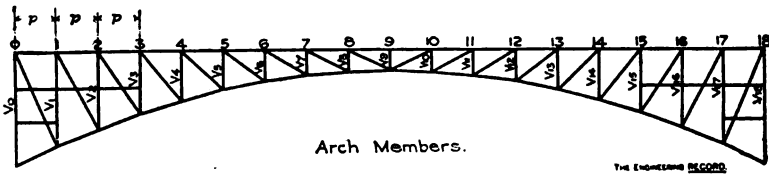
RIO GRANDE BRIDGE, COSTA RICA, 448-FOOT 8¼-INCH SPAN.
