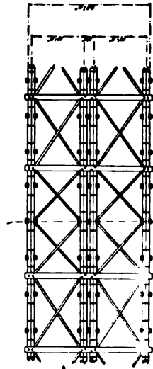
CASCADE GLEN HIGHWAY BRIDGE.
