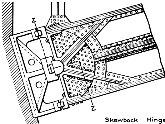
Skewback Hinge
