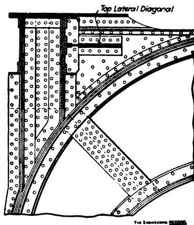
Connection of Portal to Top Chord.
