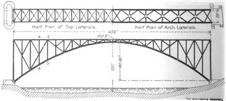
LAKE STREET HIGHWAY BRIDGE.
