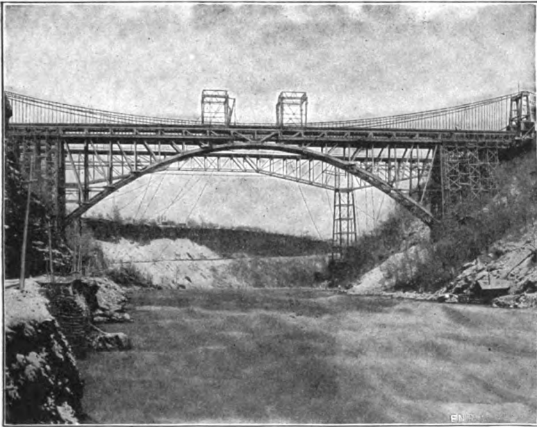
COMPLETED 550-FOOT ARCH SPAN ENCLOSING SUSPENSION SPAN, CANTILEVER SPAN IN BACKGROUND. THE THREE TYPES OF LONG-SPAN RAILROAD BRIDGES.
