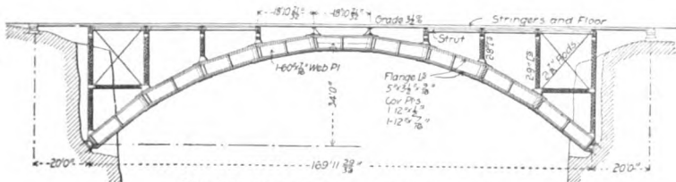
Elevation of Arch Rib and Spondrel Bracing.
