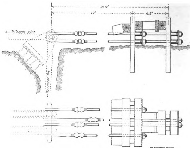
Horizontal Anchorage for Erection Adjustment.
