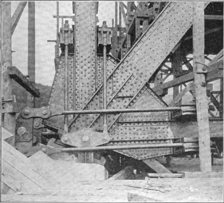
TEMPORARY SKEWBACK ADJUSTMENT.
