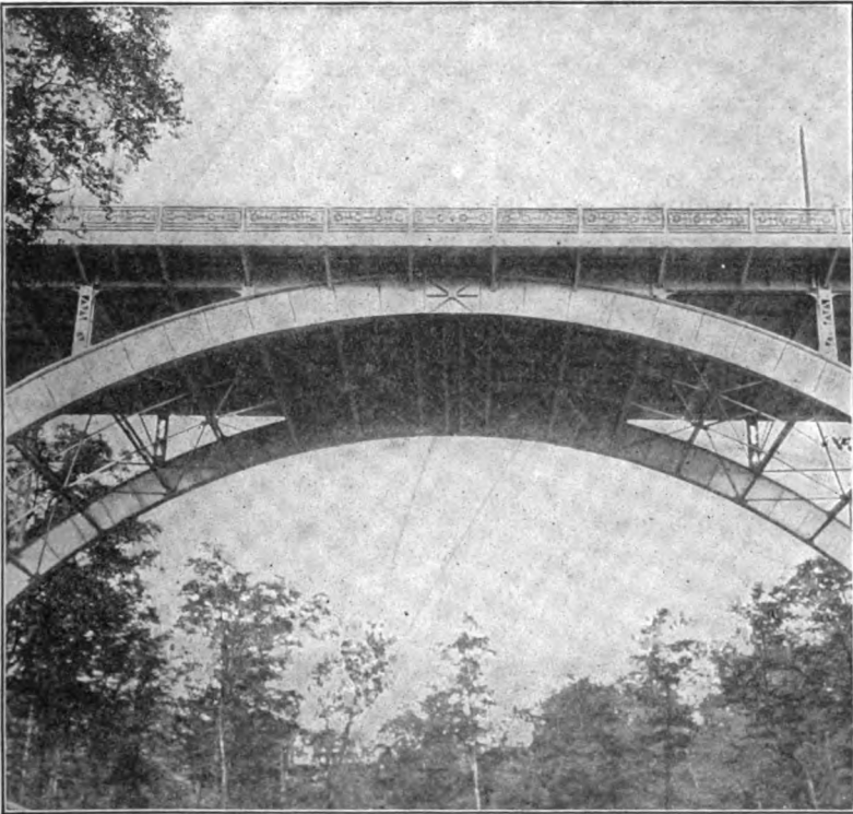
VIEW OF LATERAL BRACES.
