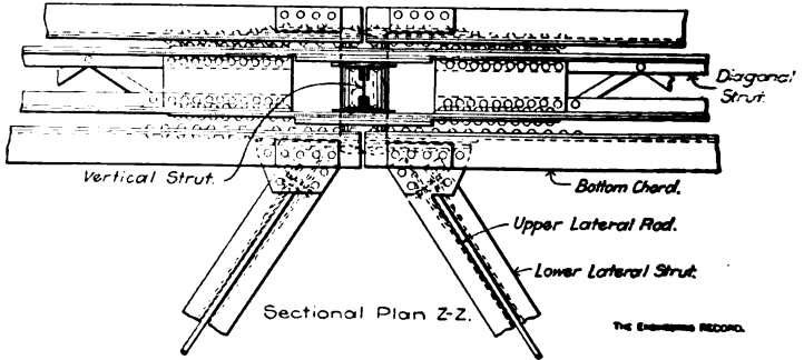
Connections at Crown.
