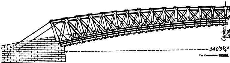
COLOSSUS BRIDGE.
