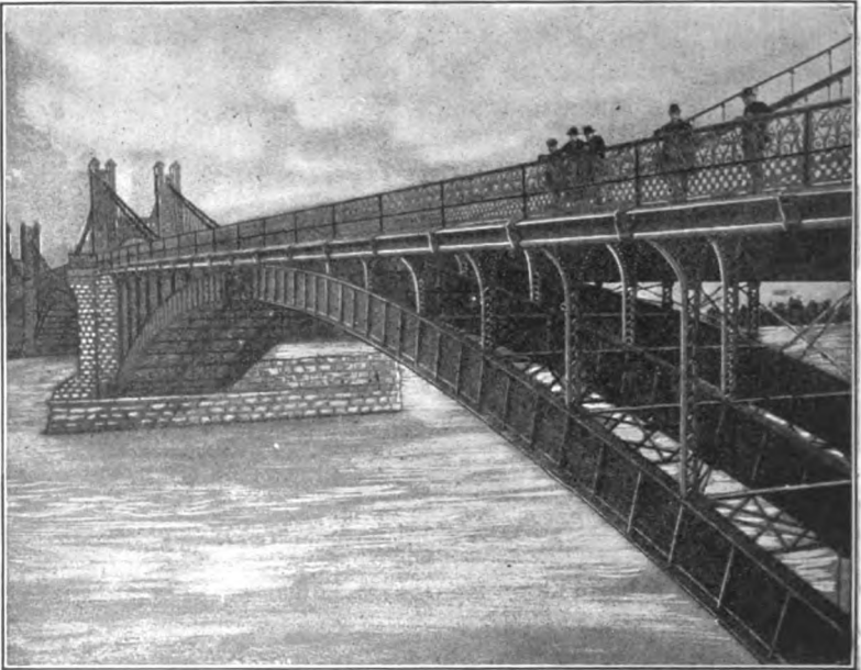
CITY BRIDGE ACROSS THE MISSISSIPPI RIVER AT MINNEAPOLIS. SPAN 258 FEET.
