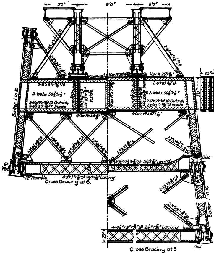
TYPICAL SEMI-CROSS SECTION.
