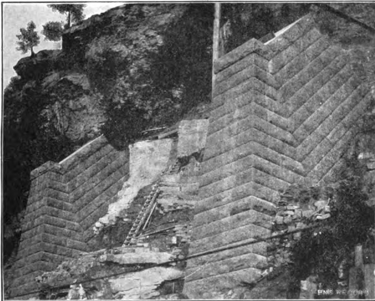
PIERS, AMERICAN SIDE.
