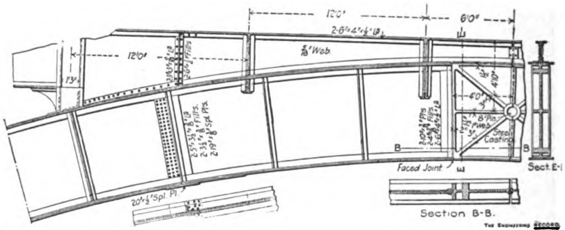
CROWN HINGE AND SPECIAL LONGITUDINAL GIRDERS.
