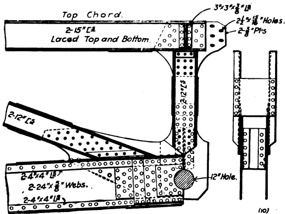
Center Panel and Crown Hinge.
