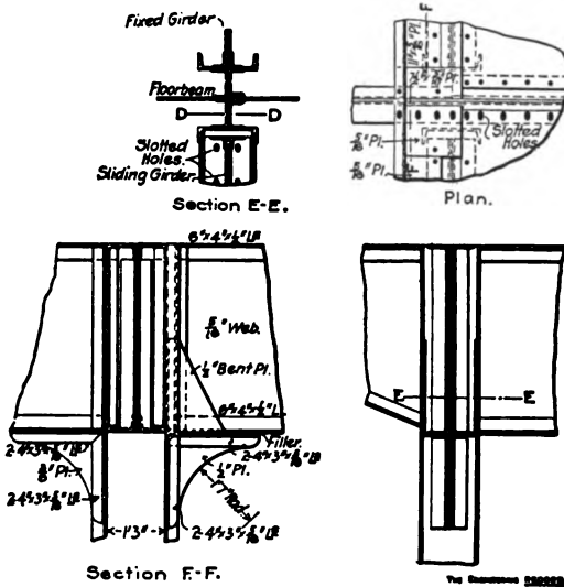
GIRDER AND COLUMN CONNECTION.
