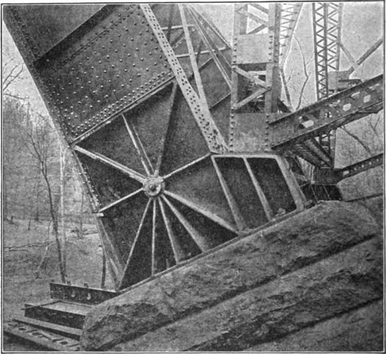
SKEWBACK HINGE AND PEDESTAL.
