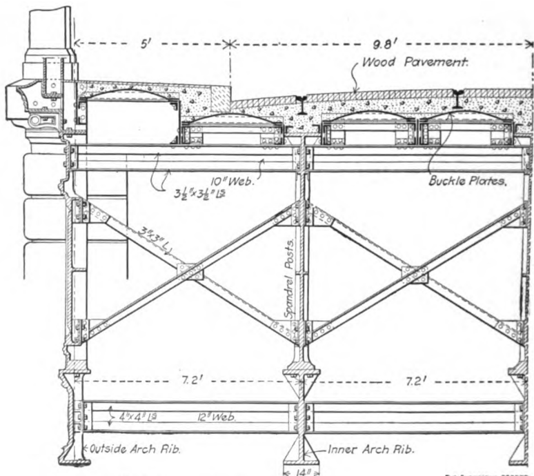
Half Cross-Section near Skewbacks.
