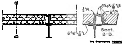
ROADWAY EXPANSION JOINTS.
