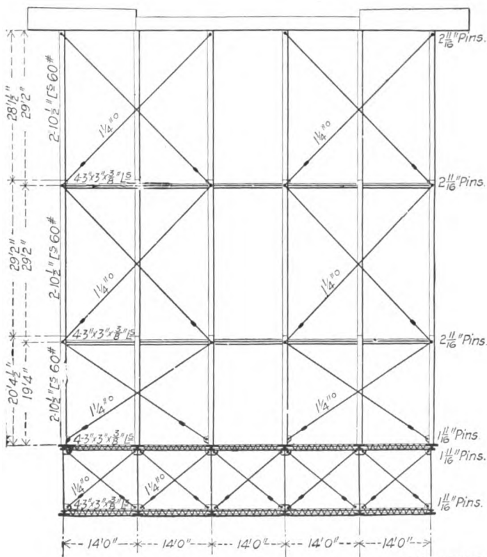
Cross-Section near Skewbacks.
