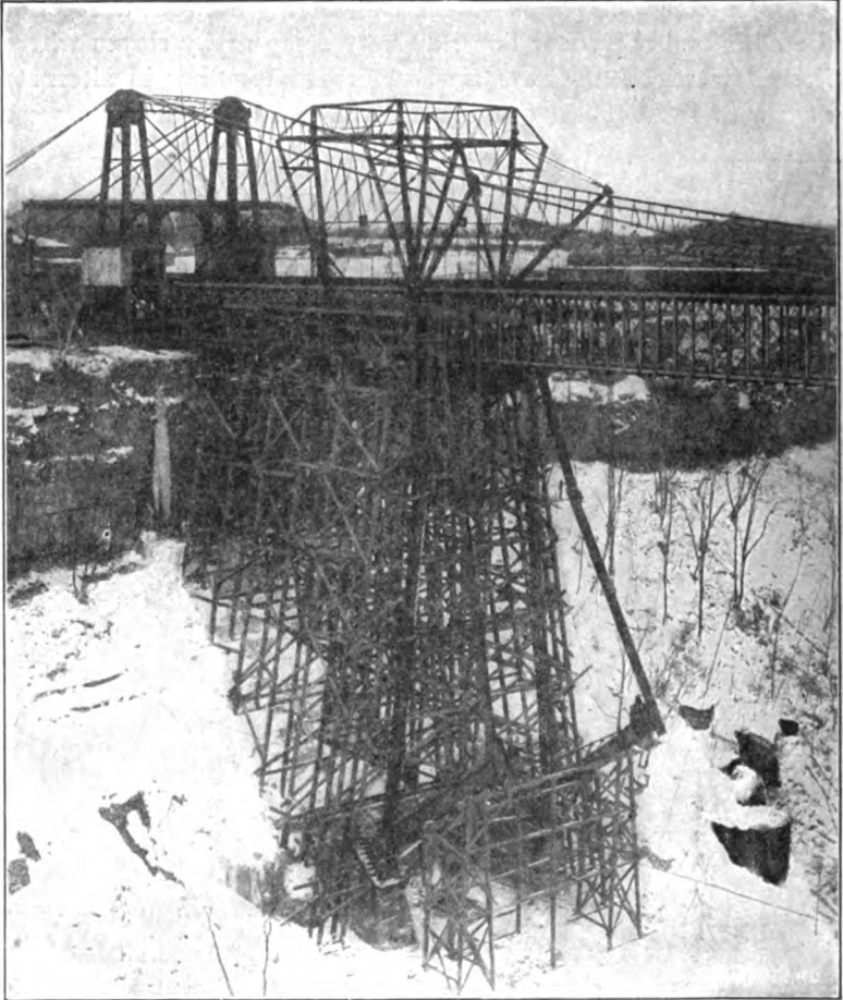
APPROACH FALSEWORK AND FIRST PANEL OF MAIN SPAN, ON CANADIAN SIDE.
