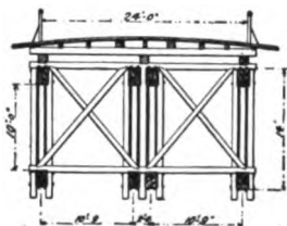
Cross Section at Crown.
