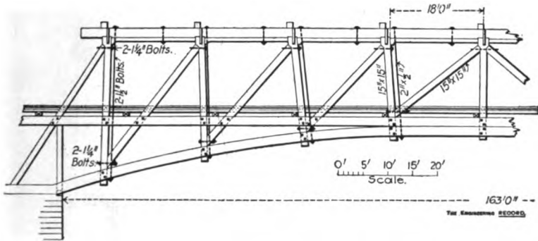
EASTON BRIDGE.
