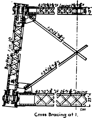
Cross Bracing at 1.
