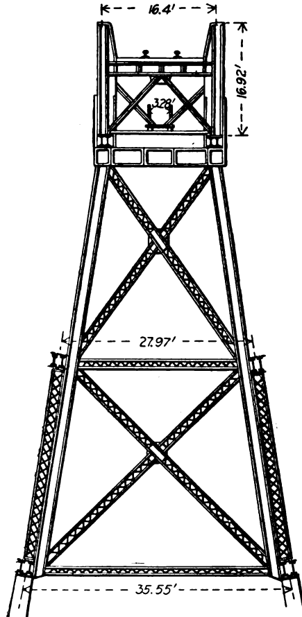
Transverse Sectional Elevation of A-A.
