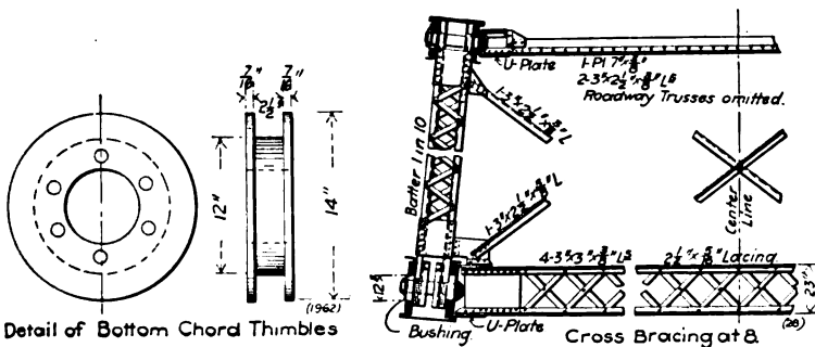
Detail of Bottom Chord Thimbles
