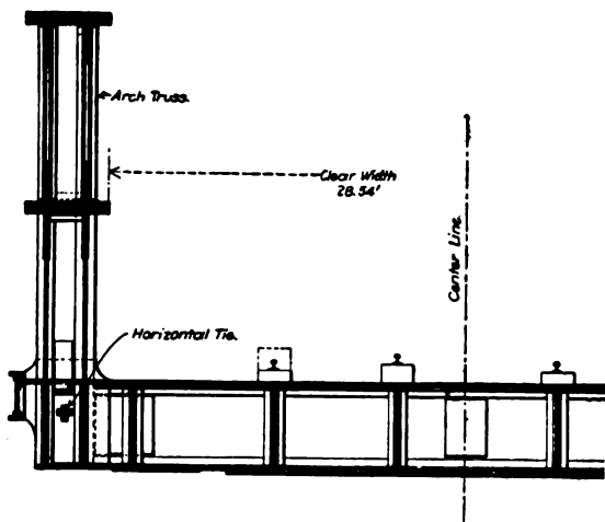
Half Section at Fifth Panel.
