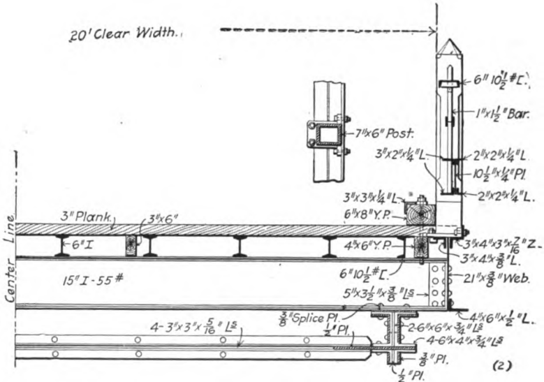
Half Section of Floor.
