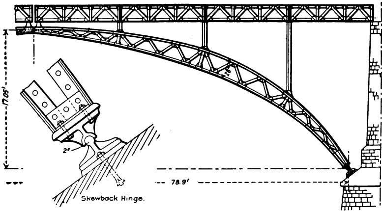
THE BRUNSWICK BRIDGE.
