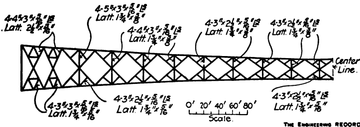
Lateral System of Top and Bottom Chords.
