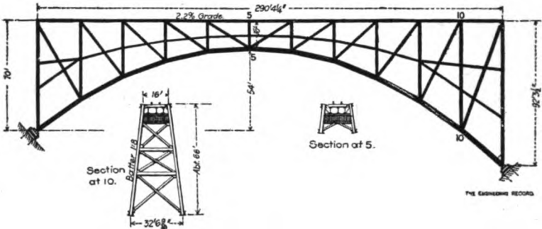
SURPRISE CREEK ARCH, CANADIAN PACIFIC RAILWAY.
