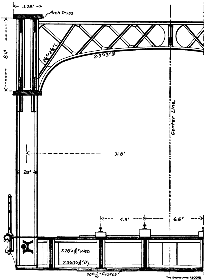
Half Cross-Section at Center.
