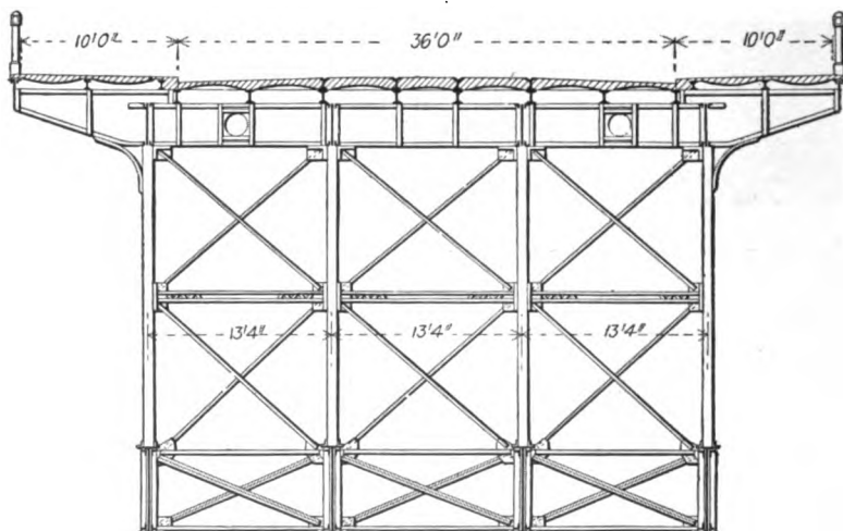
Cross - Section at Panel Point.
