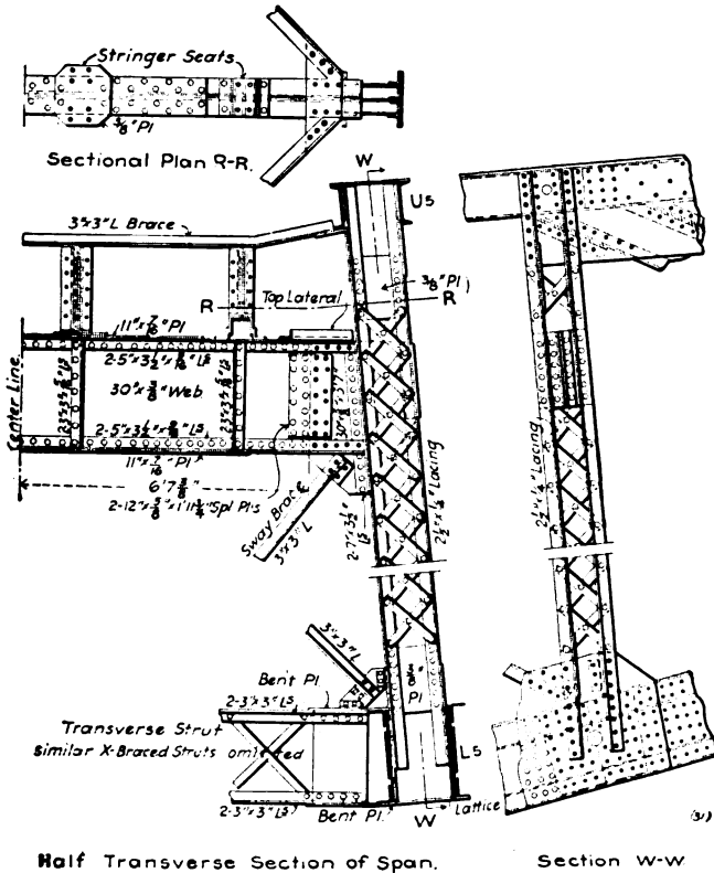
Half Transverse Section of Span.
