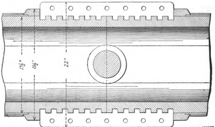
Sectional Elevation of Chord Coupling.
