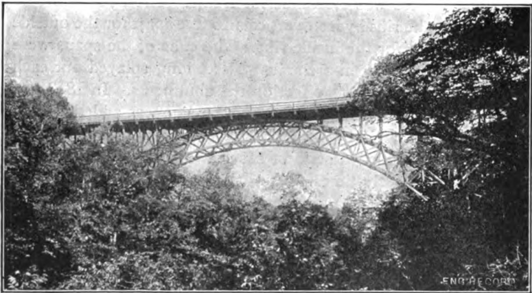
MENDOTA HIGHWAY BRIDGE, ST. PAUL, 192-FOOT SPAN.
