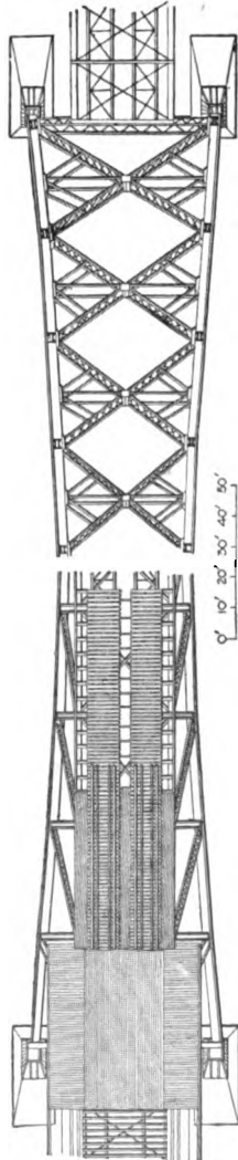
Part Top Plan. DOUBLE-TRACK RAILROAD SPAN ACROSS NIAGARA RIVER. Part Plan of Bottom Lateral. The Lateral Load.
