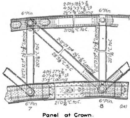
Panel at Crown.
