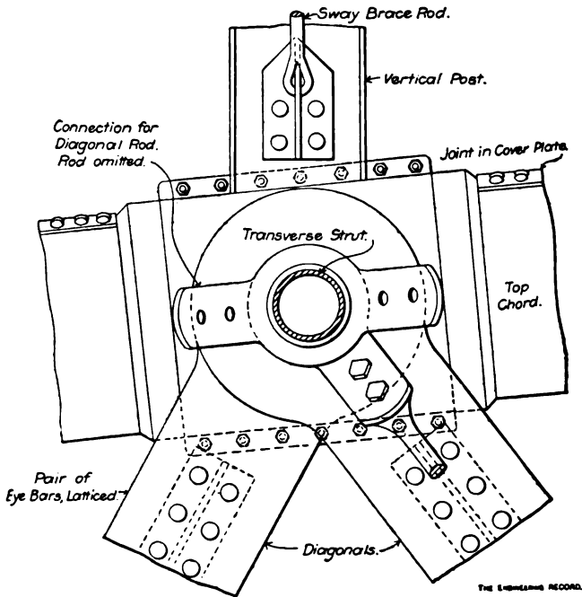
Side Elevation of Joint.
