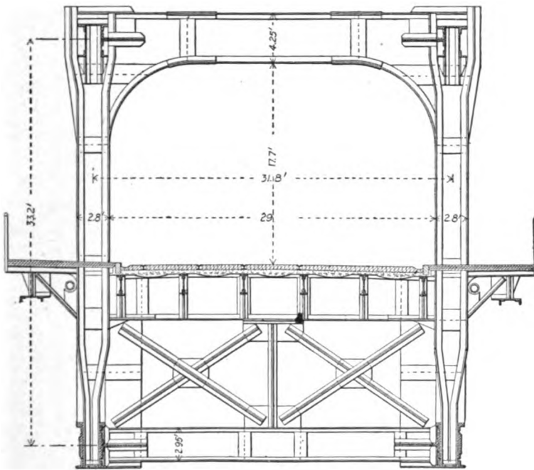
Portal and Sway; Bracing at Second Panel Point.
