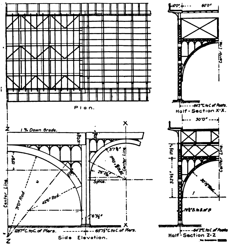
RIVERSIDE VIADUCT.
