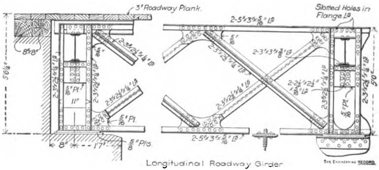
Longitudinal Roadway Girder THE ENGINEERING RECORD
