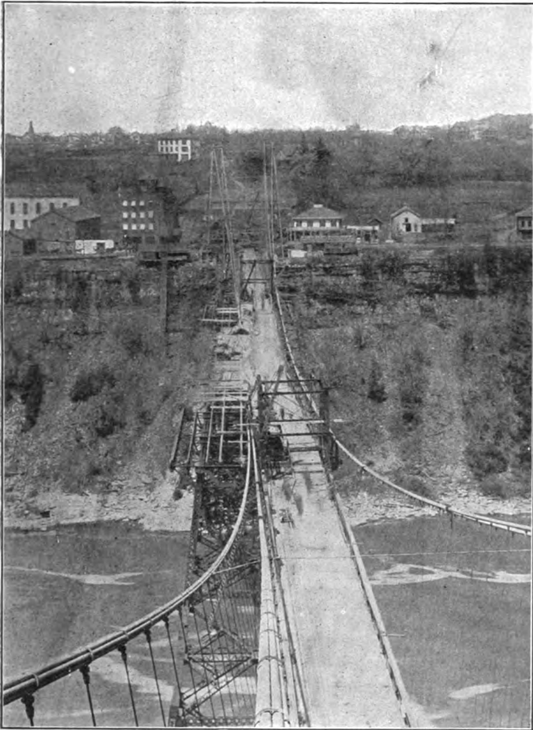
VIEW FROM TOP OF OLD TOWER OF ERECTION OF ARCH TRUSSES UNDER SUSPENSION BRIDGE IN SERVICE.
