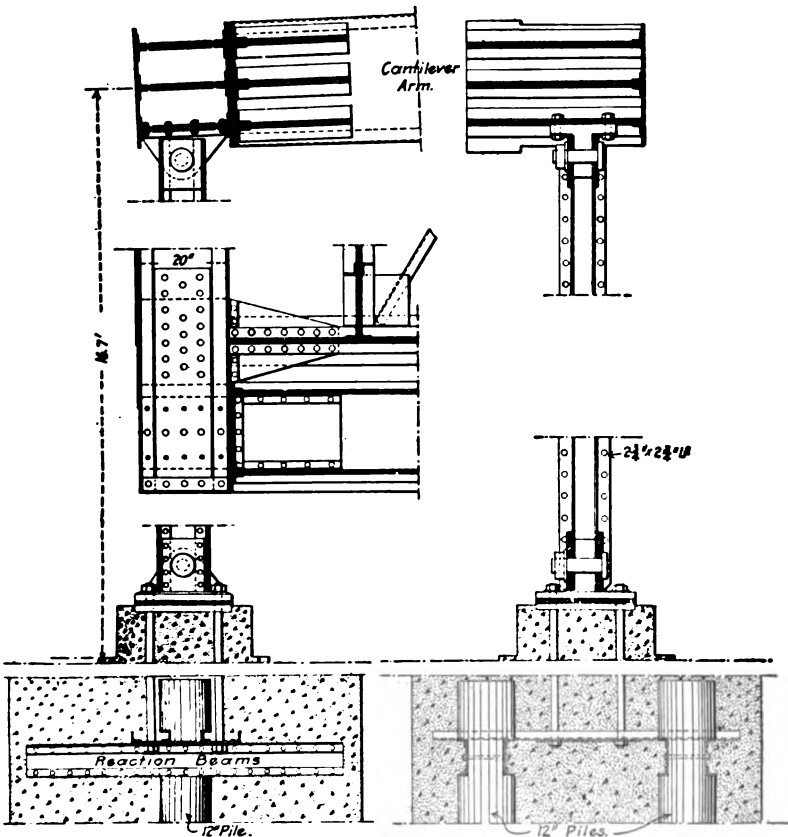
Rocker Bent and Anchorage.
