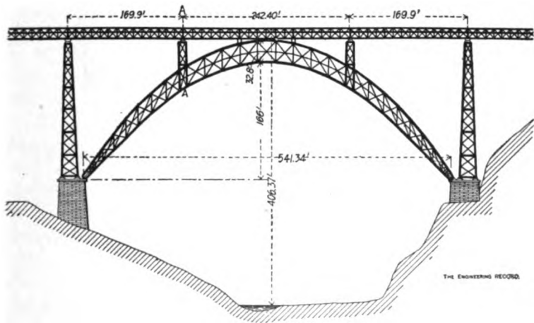
THE GARABIT VIADUCT.
