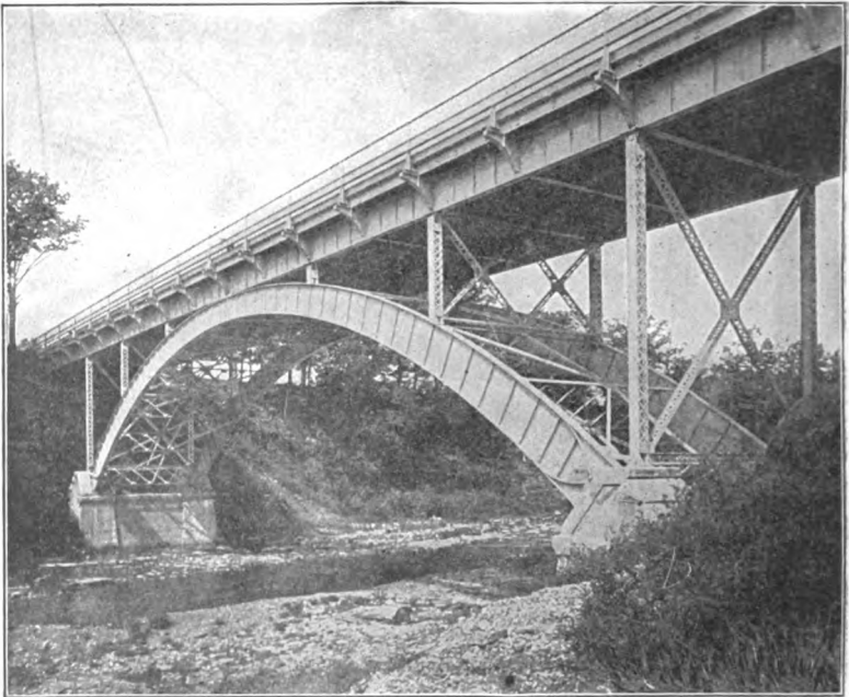
THE CHAGRIN RIVER HIGHWAY BRIDGE, 116-FOOT 9-INCH SPAN.
