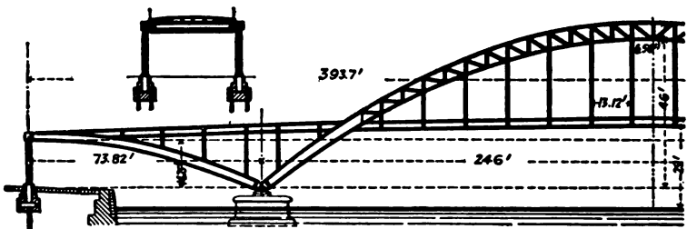
BRIDGE OVER THE SEINE, PARIS.
