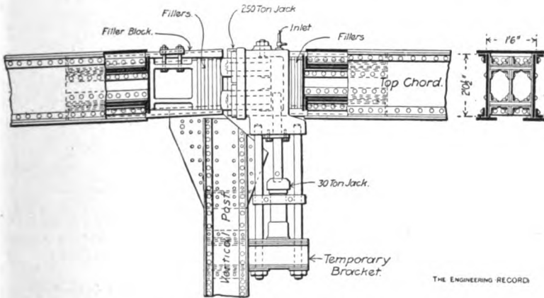
Top Rib Center Adjustment.
