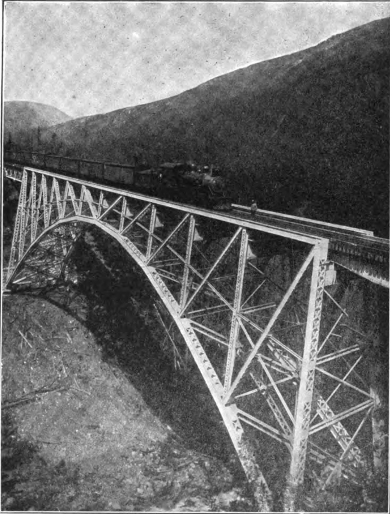
SURPRISE CREEK, 293-FOOT SINGLE-TRACK SPAN.
