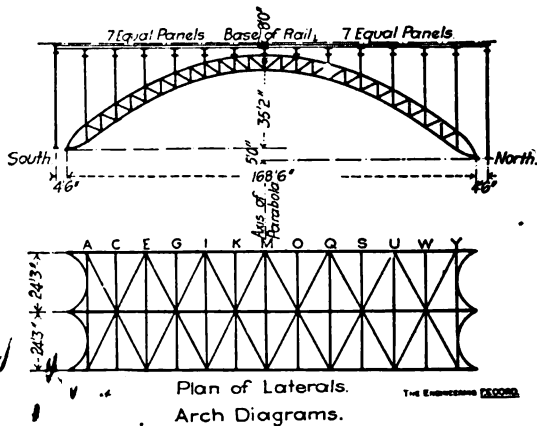
MANHATTAN VIADUCT, NEW YORK RAPID TRANSIT RAILWAY.
