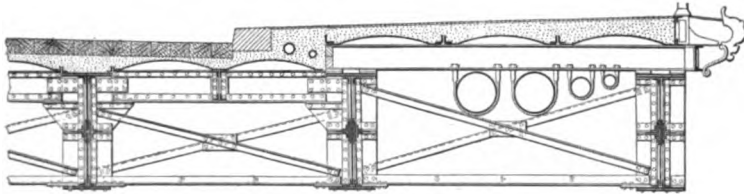
Half Cross-Section at Crown.
