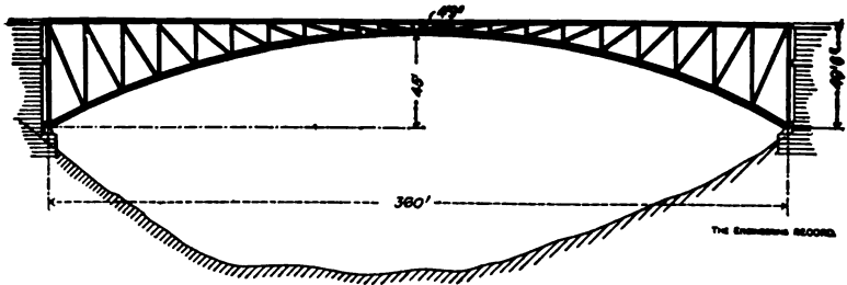
PANTHER HOLLOW BRIDGE, SCHENLEY PARK, PITTSBURG.
