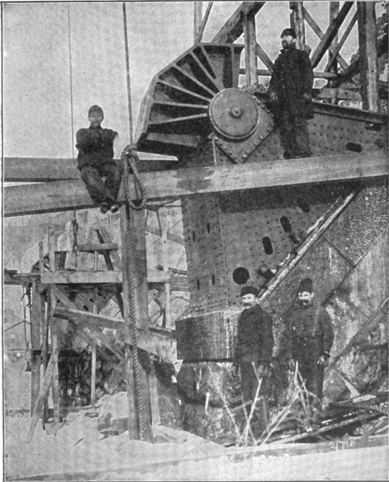
SKEWBACK HINGE.
