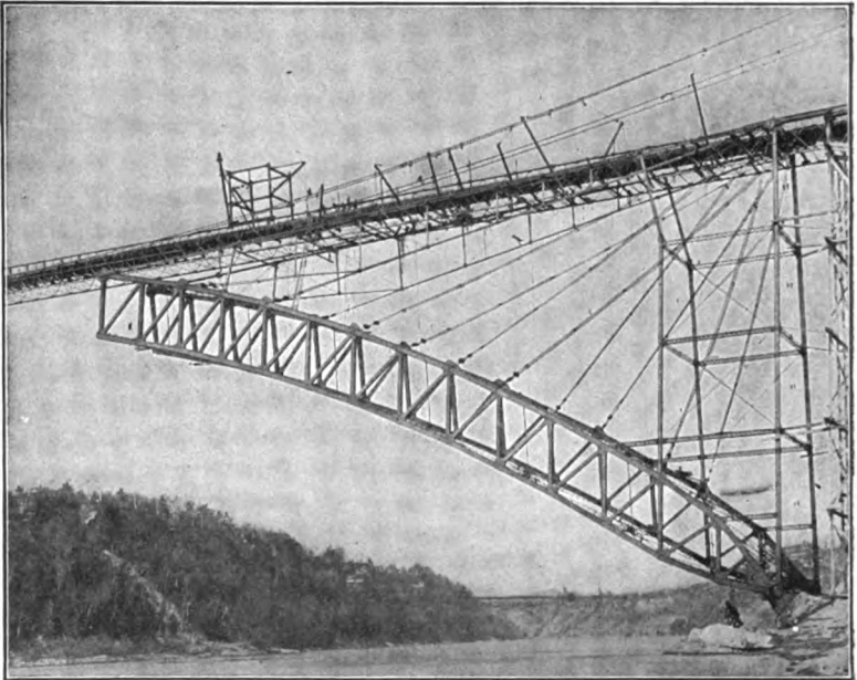
GUYED CANTILEVER ERECTION OF SEMI-SPAN.
