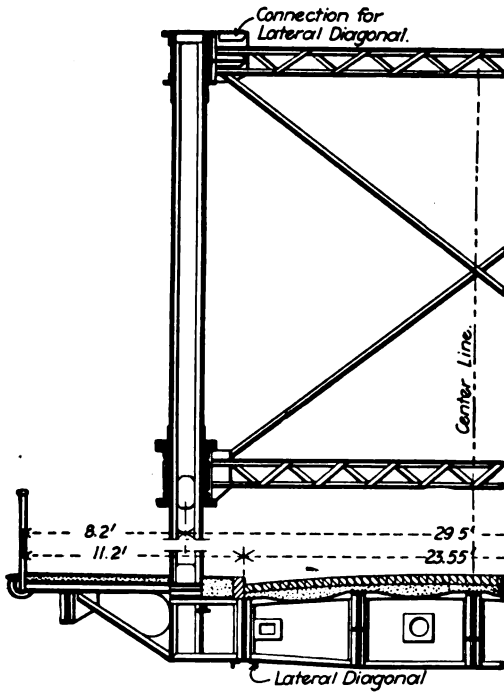
Sectional Elevation at Panel 5.
