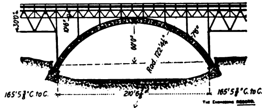
MAHONING RIVER BRIDGE, YOUNGSTOWN, OHIO.
