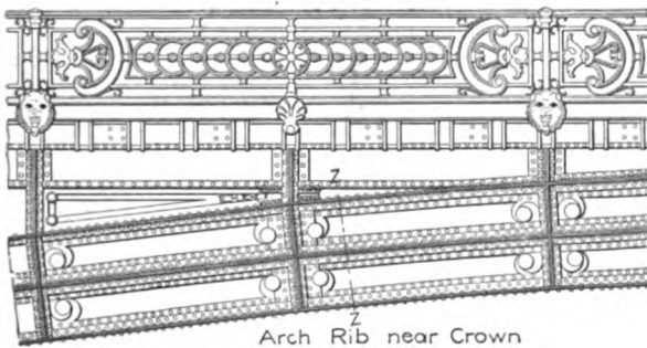
Arch Rib near Crown
