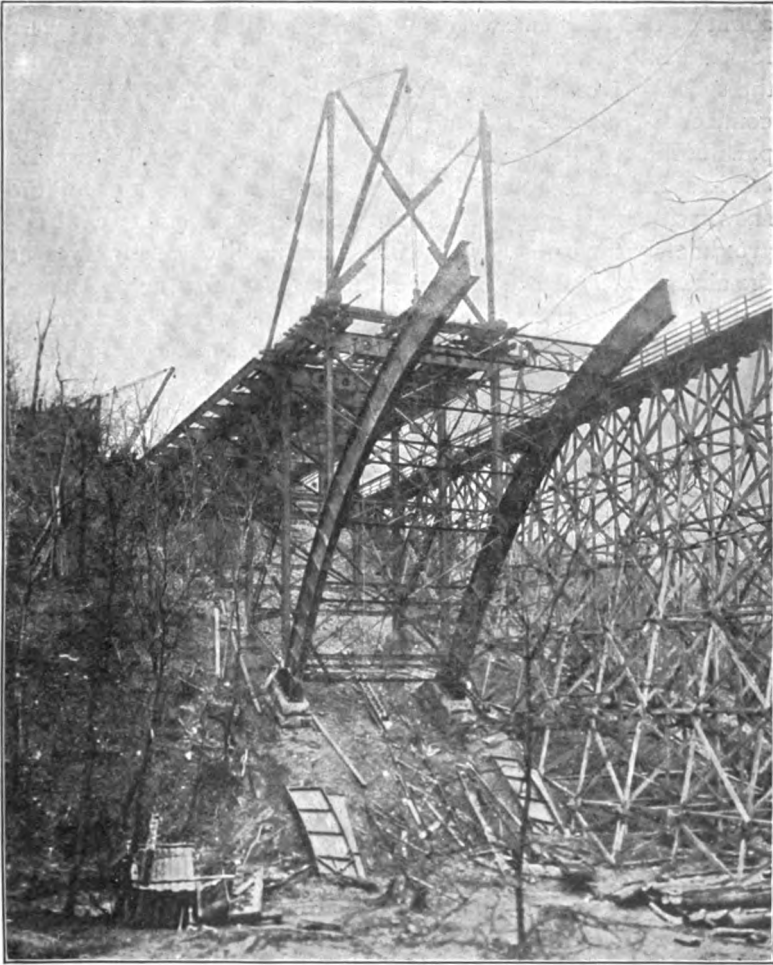
GUYED CANTILEVER ERECTION OF FERN HOLLOW BRIDGE, 195-FOOT SPANS.
