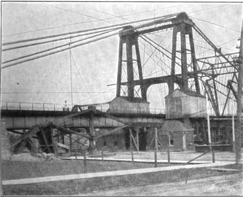
ADJUSTMENT TOGGLE IN TEMPORARY ERECTION ANCHORAGE.
