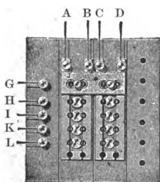
Fig. 19. Two-Circuit Way-Switch.
