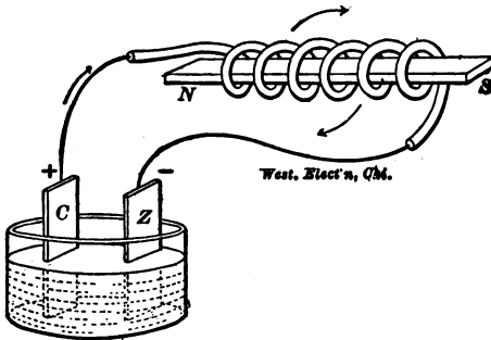
Fig. 7. Magnetized Iron Bar.
