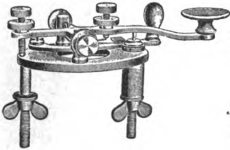
Fig. 10. The Key.
