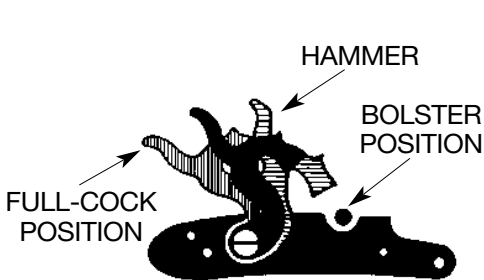
Percussion: External Lock Parts
