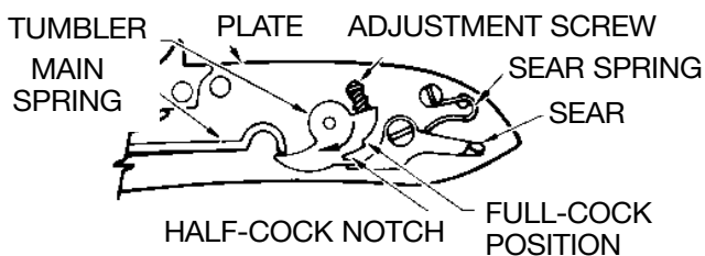
Internal Lock Parts
