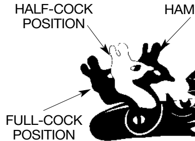
Flintlock: External Lock Parts
