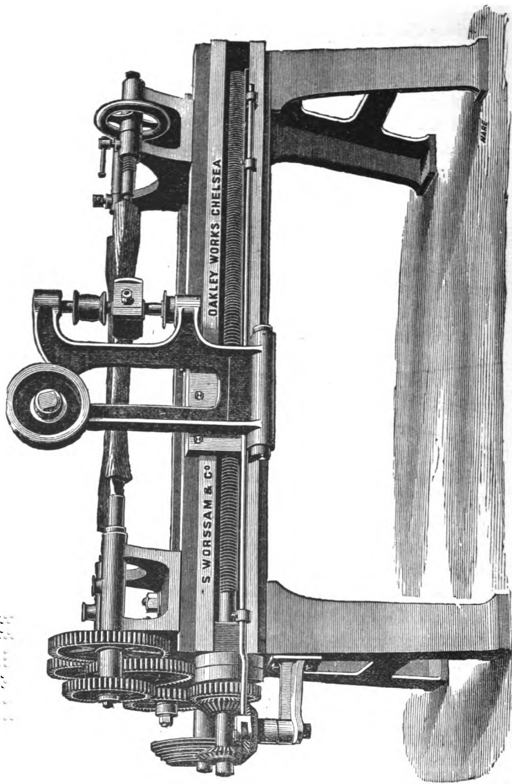
Fig 103. COPYING LATHE.
