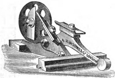
Fig. 22. CONCENTRIC SLIDE.
