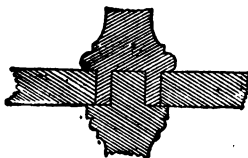
Fig. 67. MORTISING PILLARS.
