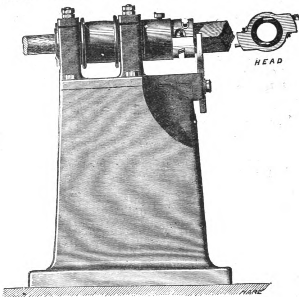
Fig. 24. SIMPLE ROUNDING MACHINE.
