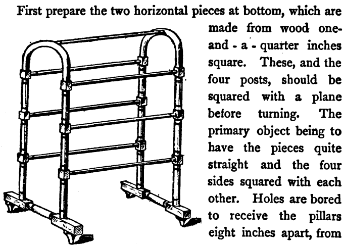
Fig. 82. TOWEL-RAIL.
