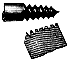
Fig. 31. SCREW TOOL FOR CUTTING THREAD ON CONE.
