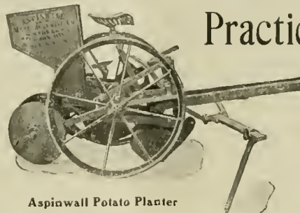
Aspinwall Potato Planter
