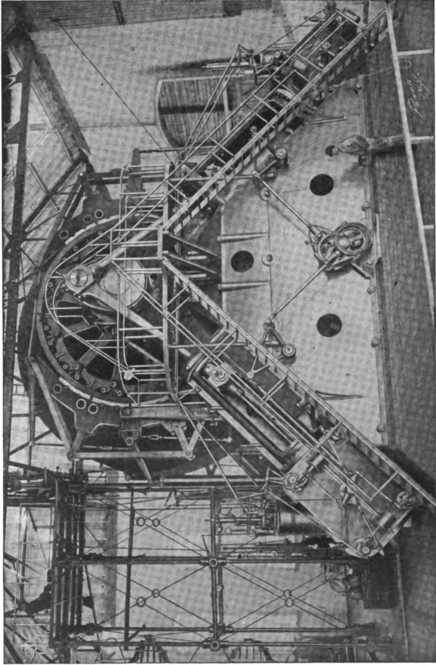
TAMARAK HOISTING ENGINE AT MINE. Nordberg Manufacturing Co
