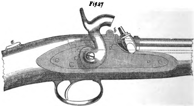
WESTLEY RICHARDS' RIFLE CLOSED. (HALF SIZE.)
