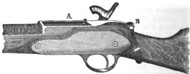
MACKENZIE AND WENTWORTH'S RIFLE CLOSED.
