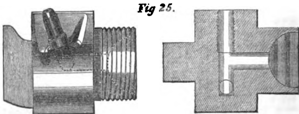
JOE MANTON'S BREECH. (FULL SIZE.)
