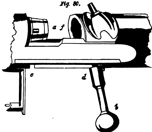
PRINCE'S RIFLE, OPEN.
