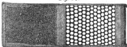
PERFORATED COPPER DISC. (FULL SIZE.) SECTION OF LOADED CARTRIDGE. (FULL SIZE.)
