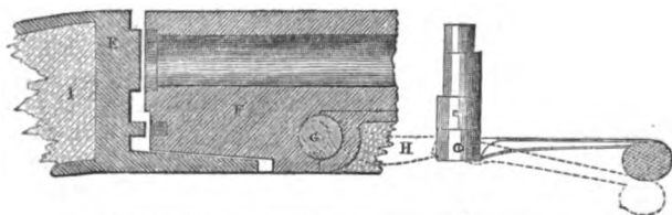
LONGITUDINAL SECTION OF DOUGALL'S GUN AND PLAN OF ECCENTRIC BOLT.
