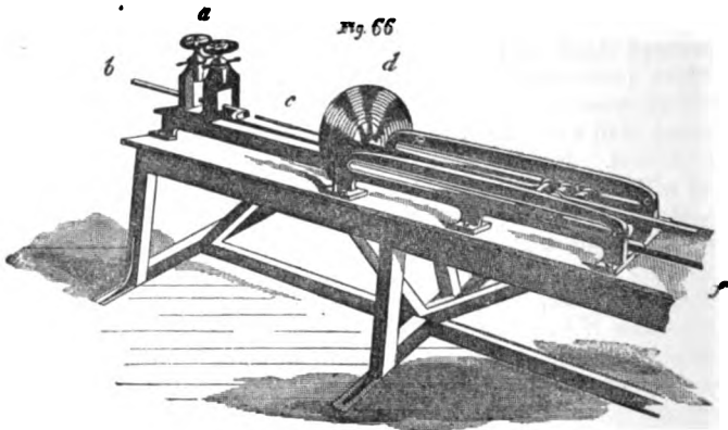
RIFLING MACHINE.
