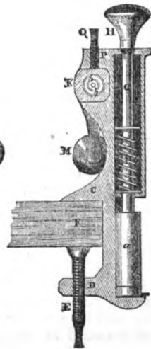
JEFFRIES' CARTRIDGE FILLING MACHINE.
