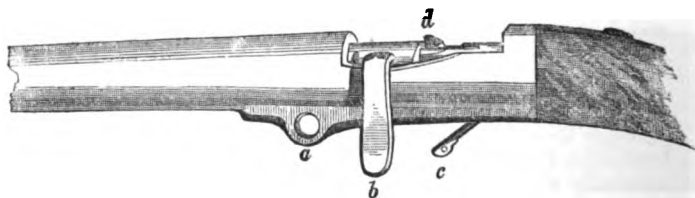
NEEDHAM'S BREECH-LOADING PUNT GUN.
