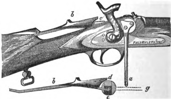
THE FIELD RIFLE OPEN, WITH THE PLUNGER AND CYLINDER SHOWN SEPARATELY.
