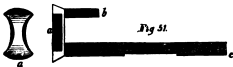
CARTRIDGE EXTRACTOR. (FULL SIZE.)
