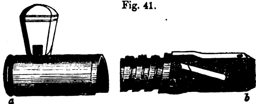
BREECH PLUG AND LOCK-CYLINDER. (HALF SIZE.)
