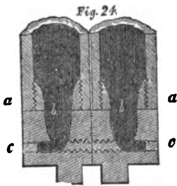
MODERN BREECH. (HALF SIZE.)
