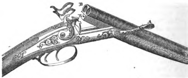
DOUGALL'S LOCKFAST BREECH-LOADER OPEN.
