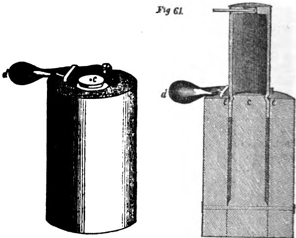
TRULOCK AND HARRIS'S CARTRIDGE-LOADING TOOL.
