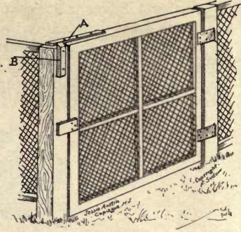
A PRACTICAL POULTRY-YARD GATE
