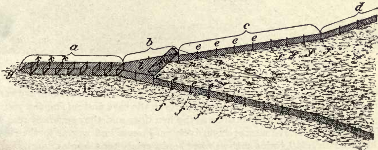
A QUAIL AND PARTRIDGE TRAP
