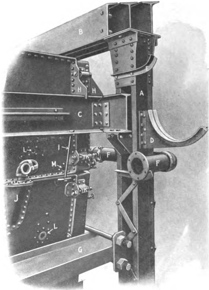
FIG. 43. — Water-jacket furnace. Method of supporting jackets
