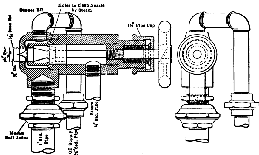
FIG. 73. — Shelby oil-burner
