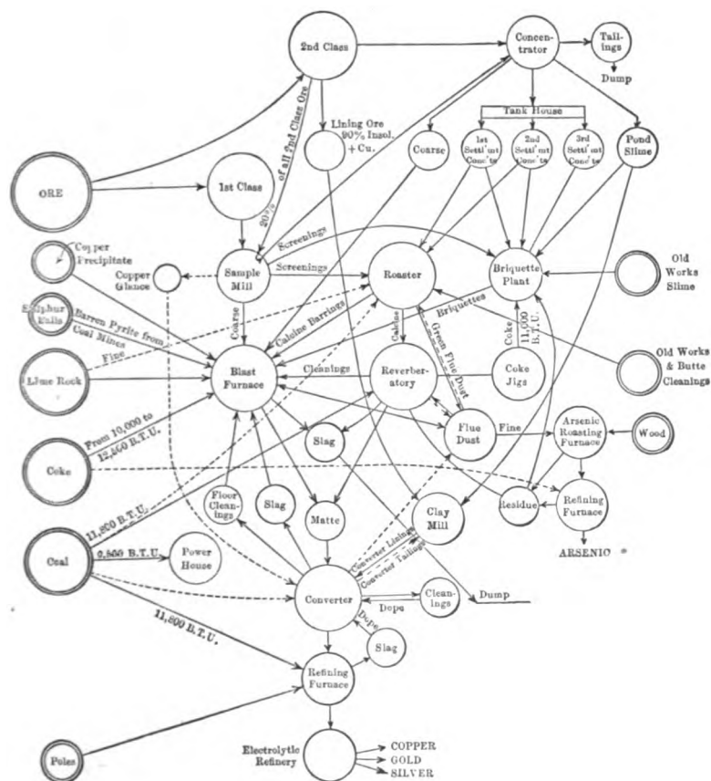
FIG. 52. — Washoe flow-sheet
