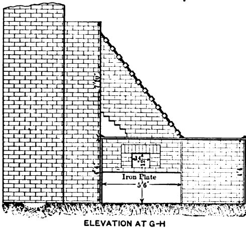
FIG. 78. — Boston and Colorado wood-burning reverberatory — front elevation
