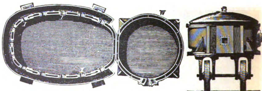
FIG. 27. — Furnace with trapped forehearth — cross-section
