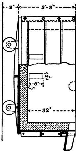
FIG. 35. — Siphon-tap forehearth — plan
