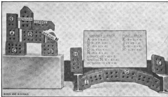
FIG. 110. — Special brick used in chimney
