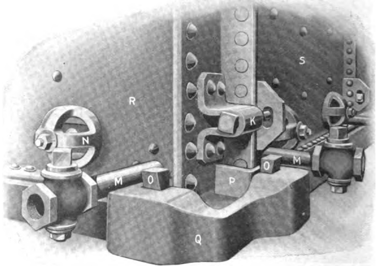
FIG. 41. — Lower corner of furnace
