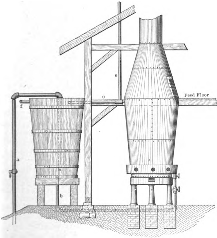
FIG. 21. — Early type of water-jacket furnace
