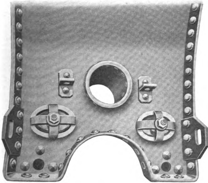
FIG. 39. — Exterior of jacket
