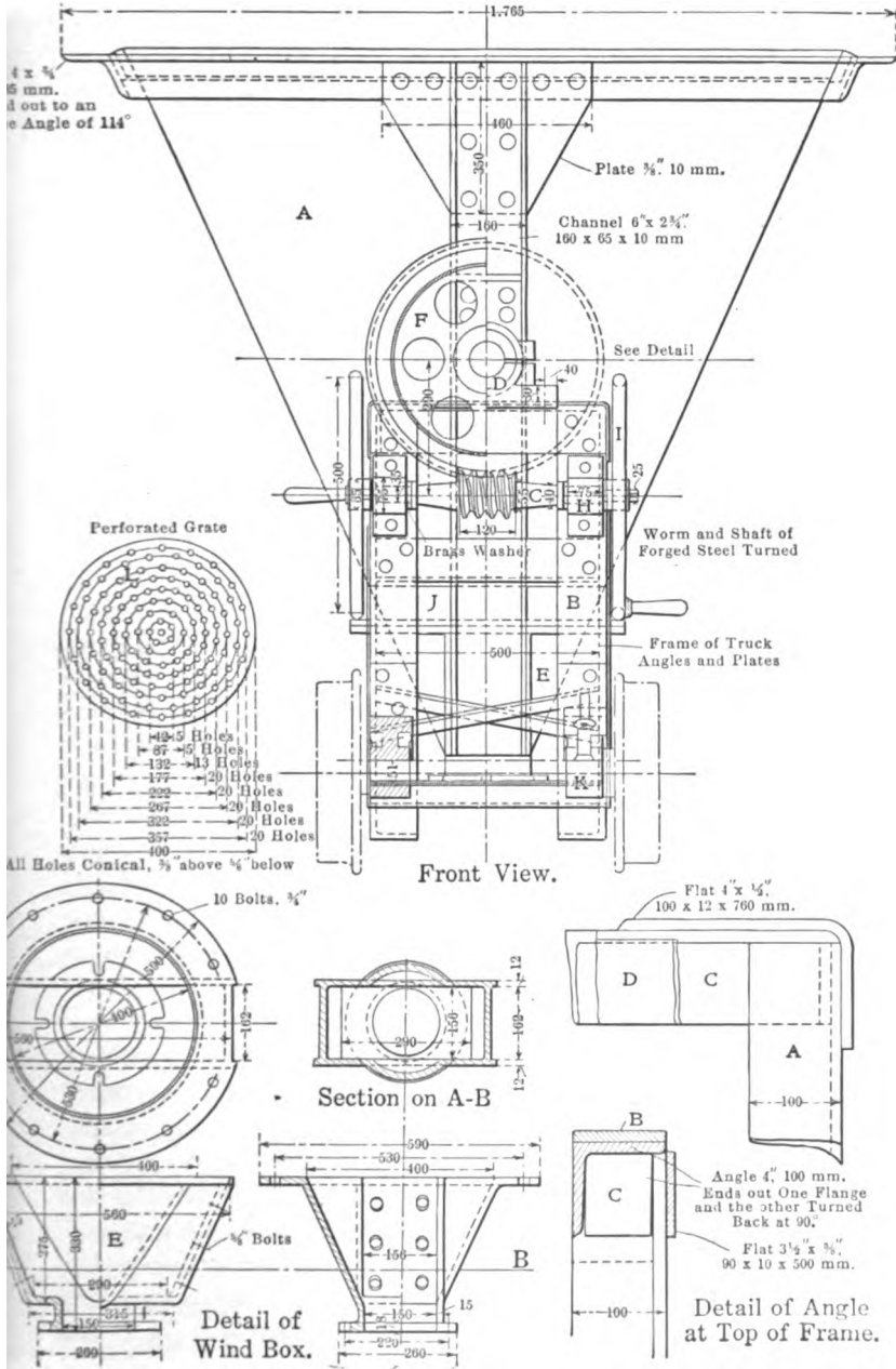
FIG. 85. — Collins sintering-pot. Details of grate and wind-box
