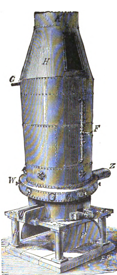
FIG. 22. — Furnace for oxidized ores — elevation
