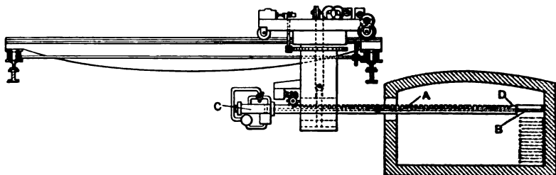
FIG. 103. — Clark and Artisell charging-crane
