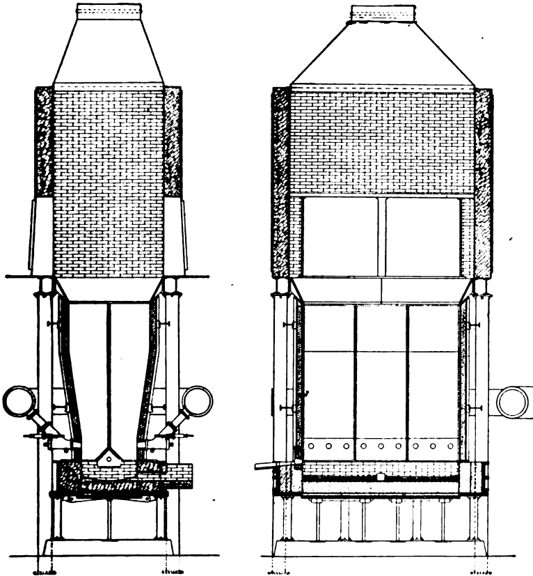
FIGS. 31-32. — Matting furnace with inside crucible — vertical section
