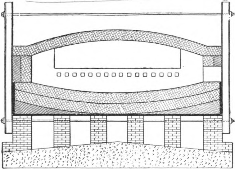
FIG. 107. — Cross-section of melting furnace at Michigan smelter
