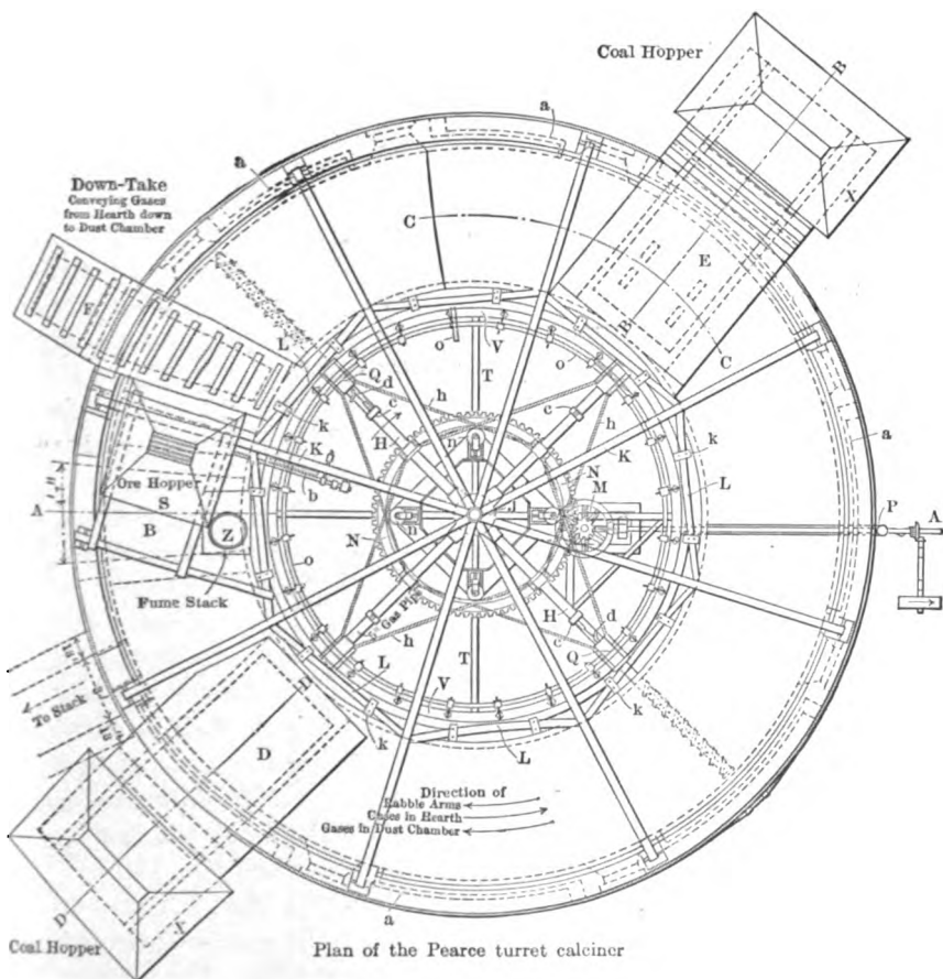
FIG. 11. — Pearce turret furnace — plan
