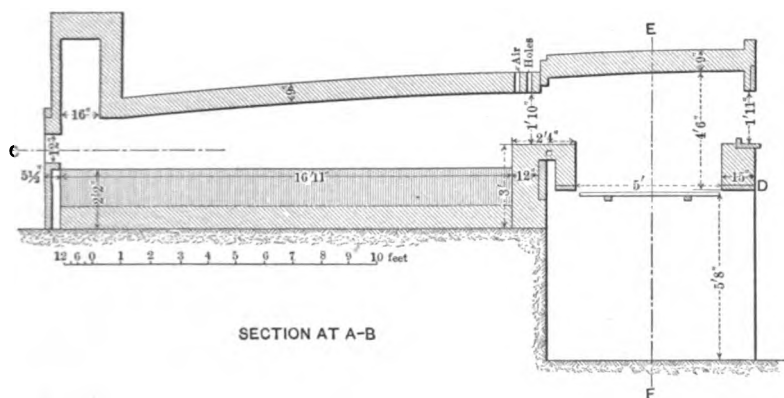
FIG. 76. — Boston and Colorado wood-burning reverberatory — longitudinal section
