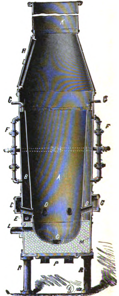
FIG. 23. — Furnace for oxidized ores — vertical section
