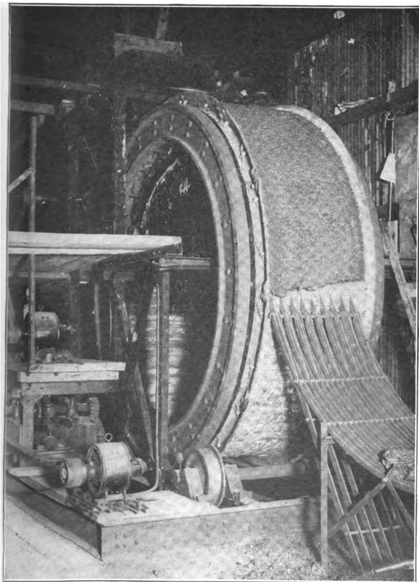
FIG. 87. — Dwight Lloyd drum sintering machine
