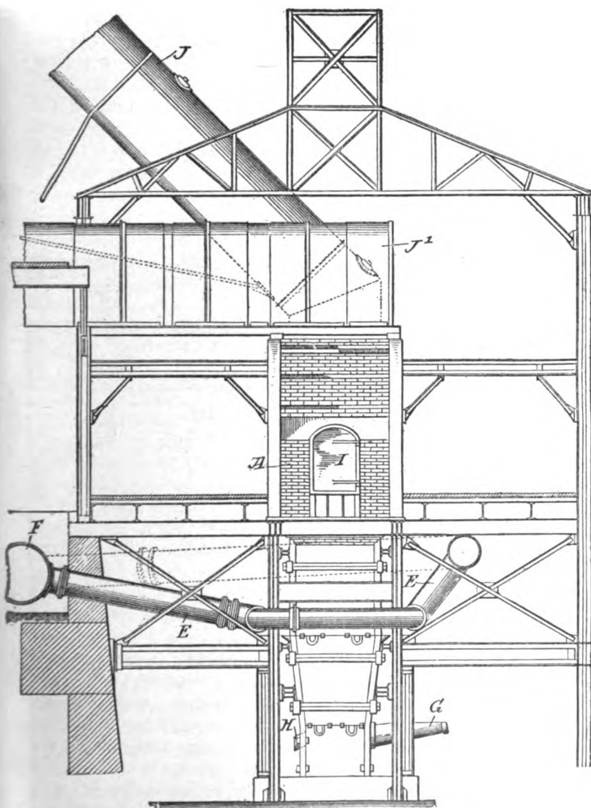
FIG. 55. — Washoe blast-furnace — end elevation
