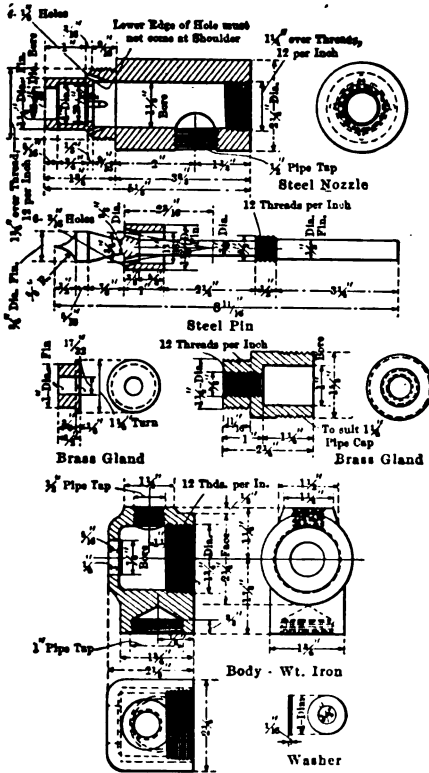
FIG. 74. — Shelby oil-burner — details
