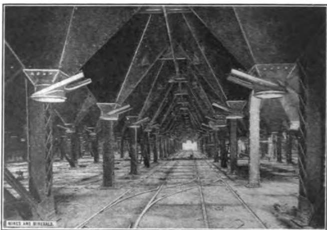
FIG. 112. — Basement, showing hoppers below dust-collecting chambers
