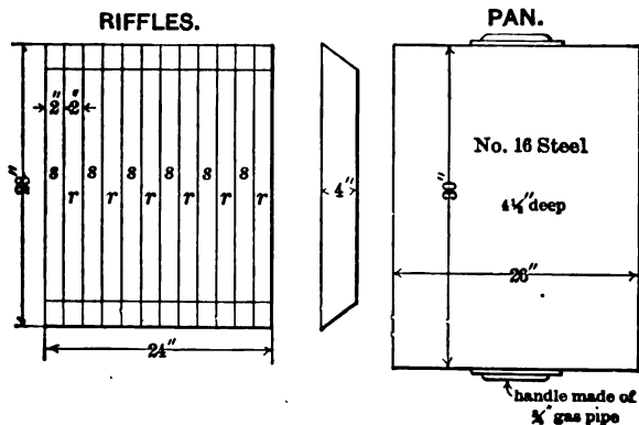
FIGS. 4 AND 5. — Riffle sampler
