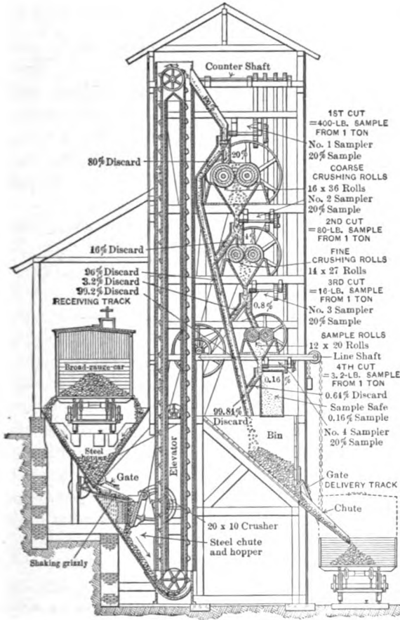
FIG. 7. — Sampling-mill
