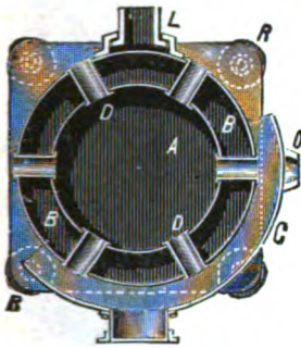
FIG. 24. — Furnace for oxidized ores — cross-section
