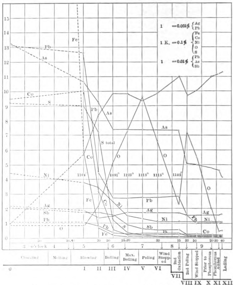
FIG. 102. — Removal of impurities during refining
