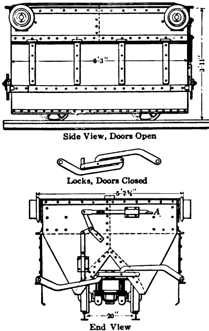
FIG. 47. — Furnace-charging car
