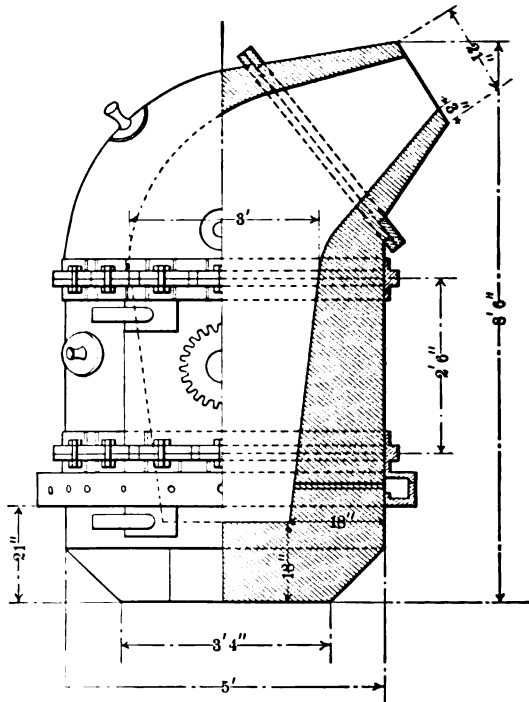
FIG. 89. — Parrot converter
