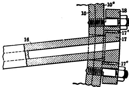
FIG. 97. — Basic-lined converter — the cast-iron tuyere
