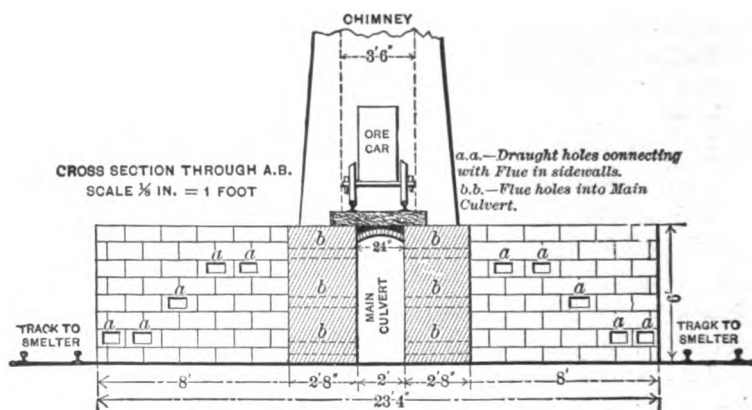
FIG. 19. — Roast stalls for ore — section
