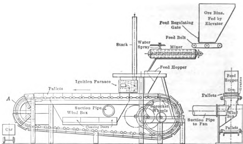
Fig. 86. — Dwight-Lloyd straight-line blast-roasting machine
