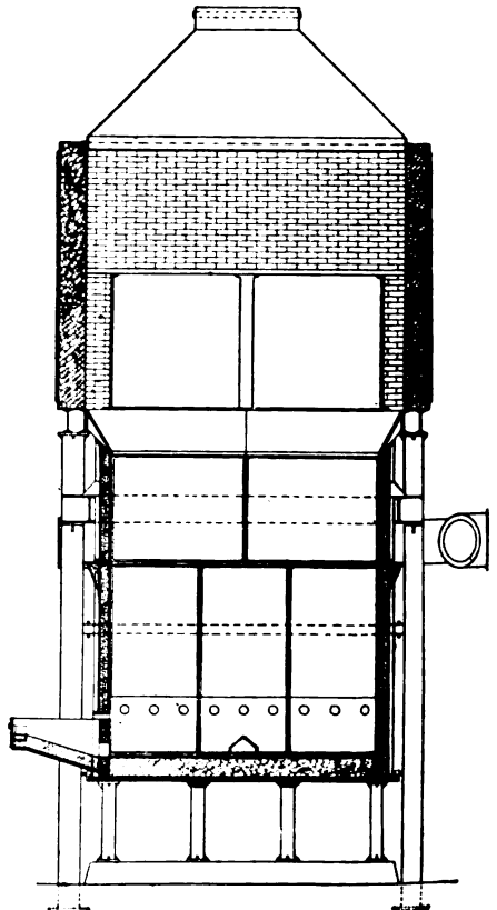
FIG. 30. — Standard matting furnace — vertical section
