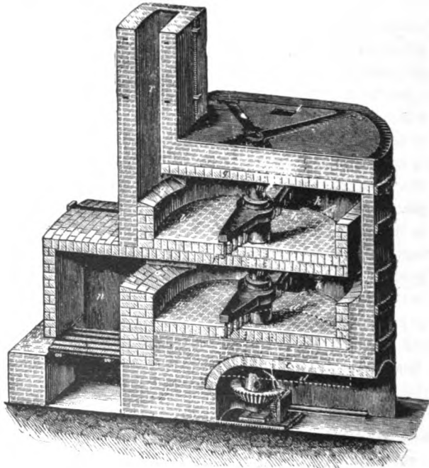
FIG. 8. — Parke's roasting furnace
