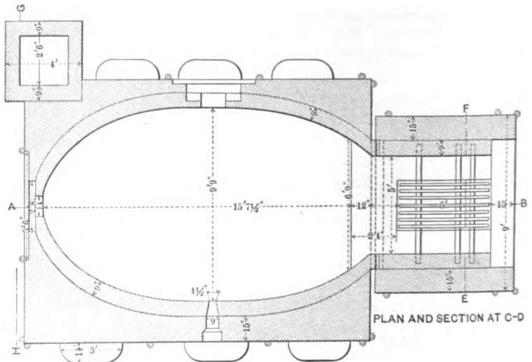
FIG. 77. — Boston and Colorado wood-burning reverberatory — sectional plan
