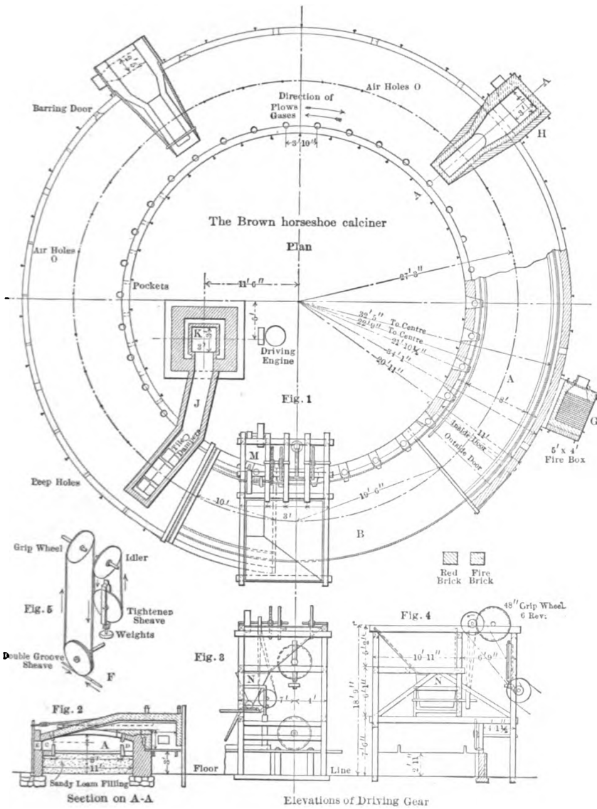
FIG. 10. — The Brown horseshoe calciner
