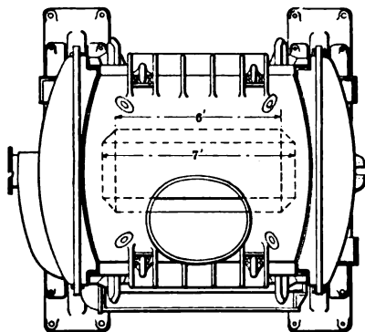
Fig. 92. — Barrel converter — top view
