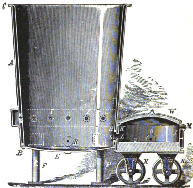
FIG. 26. — Furnace with trapped forehearth — vertical section
