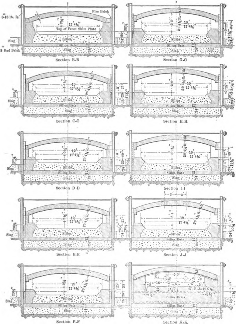
FIG. 70. — Washoe reverberatory — cross-sections
