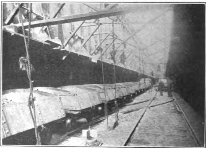
FIG. 57. — Washoe smelter charging train receiving load from ore-bins
