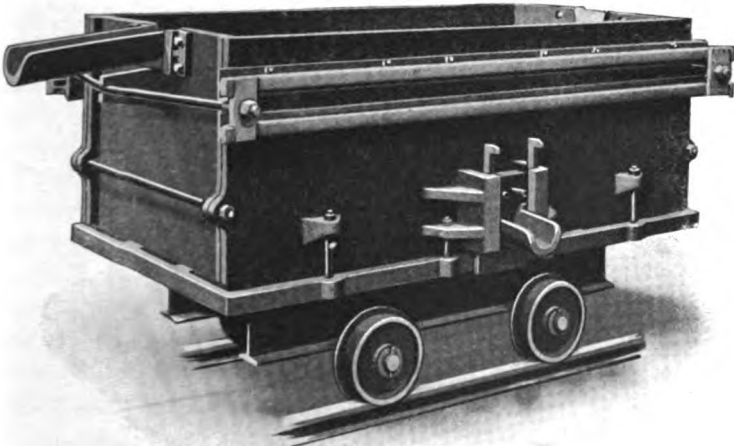
FIG. 34. — Portable forehearth
