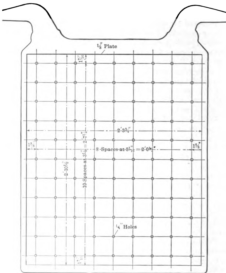
FIG. 106. — Templet for sampling anodes
