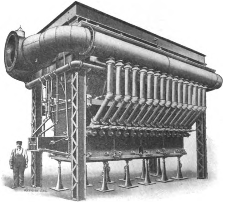
FIG. 41. — Copper-matting furnace
