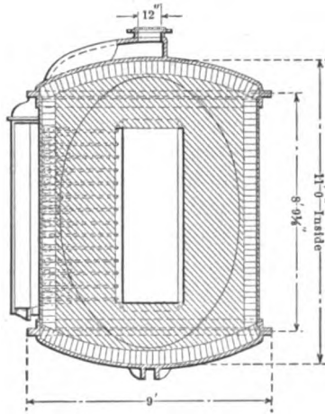
Fig. 94. — Barrel converter — longitudinal section
