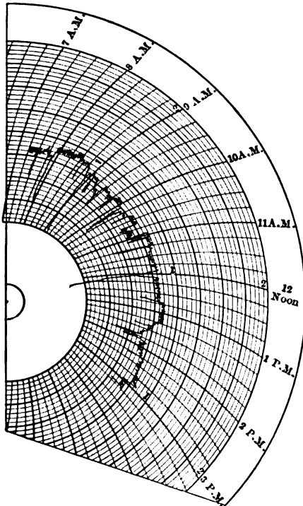
FIG. 72. — Washoe reverberatory draught-pressure
