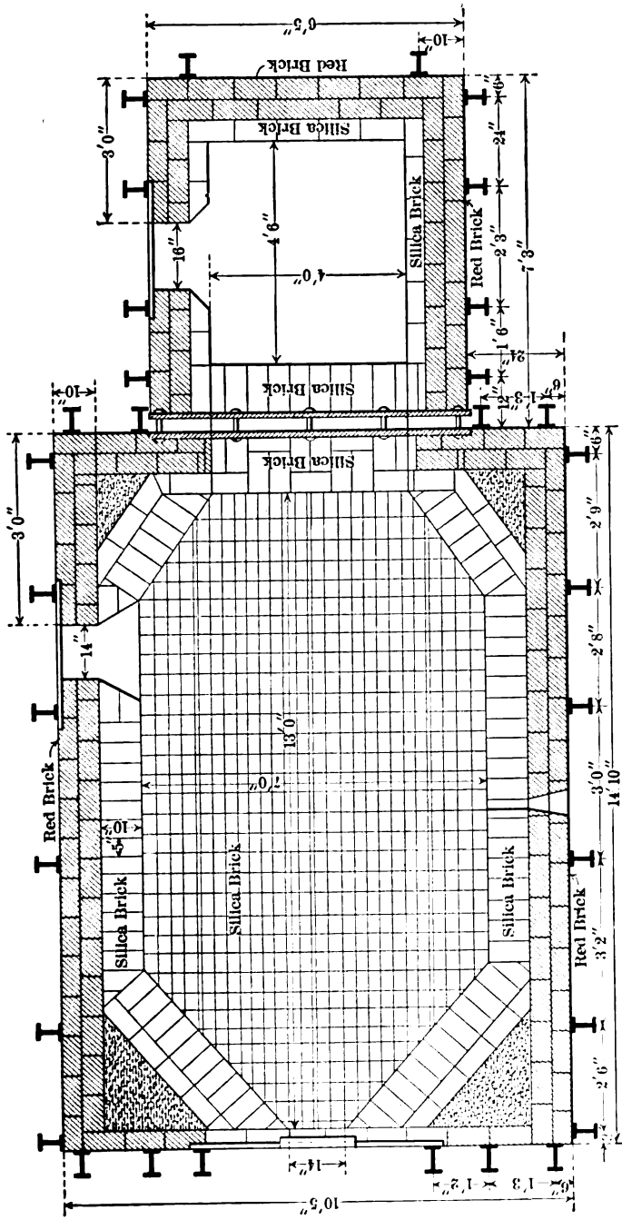
Fig. 82. — Home-made wood-burning reverberatory — sectional plan
