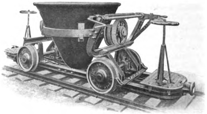
FIG. 117. — Screw-dump slag-pot
