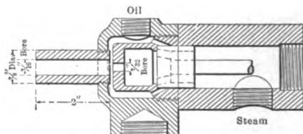
Fig. 75. — Shelby oil-burner — Modified type
