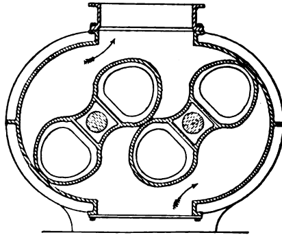
FIG. 48. — Cross-section through center of rotary-piston blower
