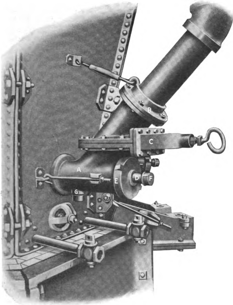
FIG. 42. — Water-jacket furnace tuyere-connections
