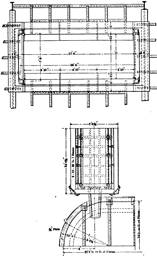
FIG. 62b. — Cananea blast-furnace — plan
