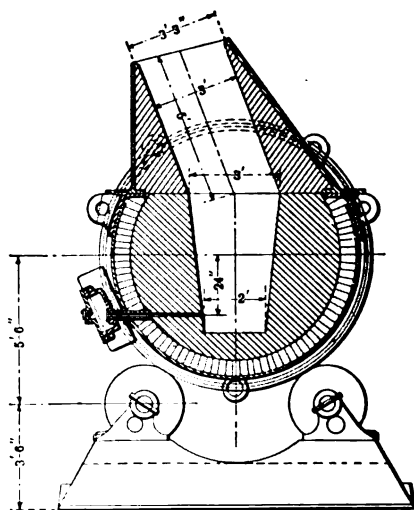
FIG. 93. — Barrel converter — vertical section
