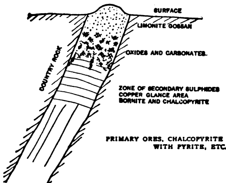
FIG. 1. — Weathering of ore in a vein
