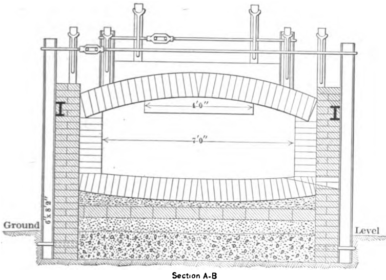
FIG. 80. — Home-made wood-burning reverberatory — cross-section
