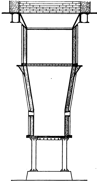
FIG. 28. — Water-jackets — vertical section
