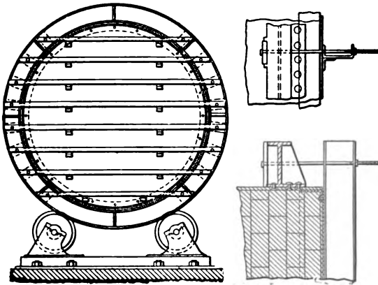
FIG. 101. — Basic-lined converter — section of head and details of clamp-bars
