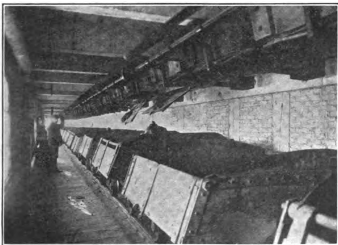
FIG. 58. — Washoe smelter. Charging train loading briquettes
