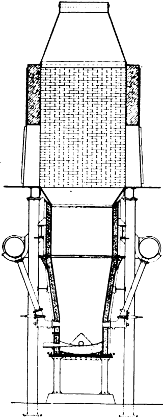
FIG. 29. — Standard matting furnace — vertical section
