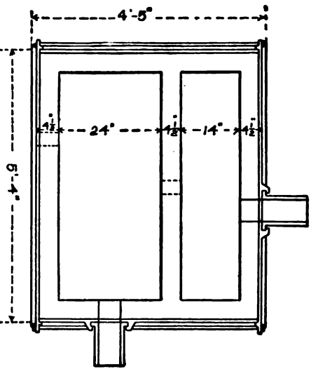
FIG. 36. — Siphon-tap forehearth — longitudinal section
