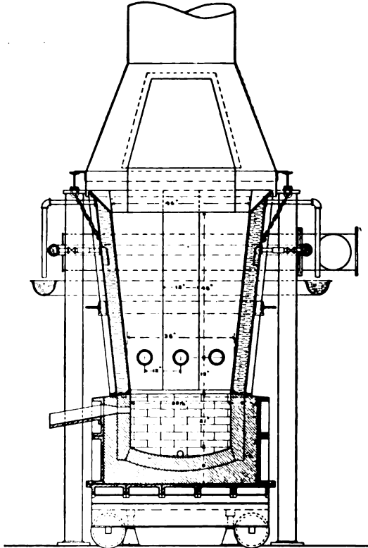
FIG. 46. — Sectionalized water-jacket furnace — rectangular
