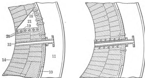
FIG. 99. — Basic-lined converter. Brackets to confine lining
