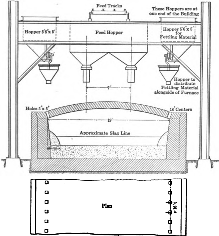
FIG. 71. — Cananea reverberatory. Method of continuous fettling
