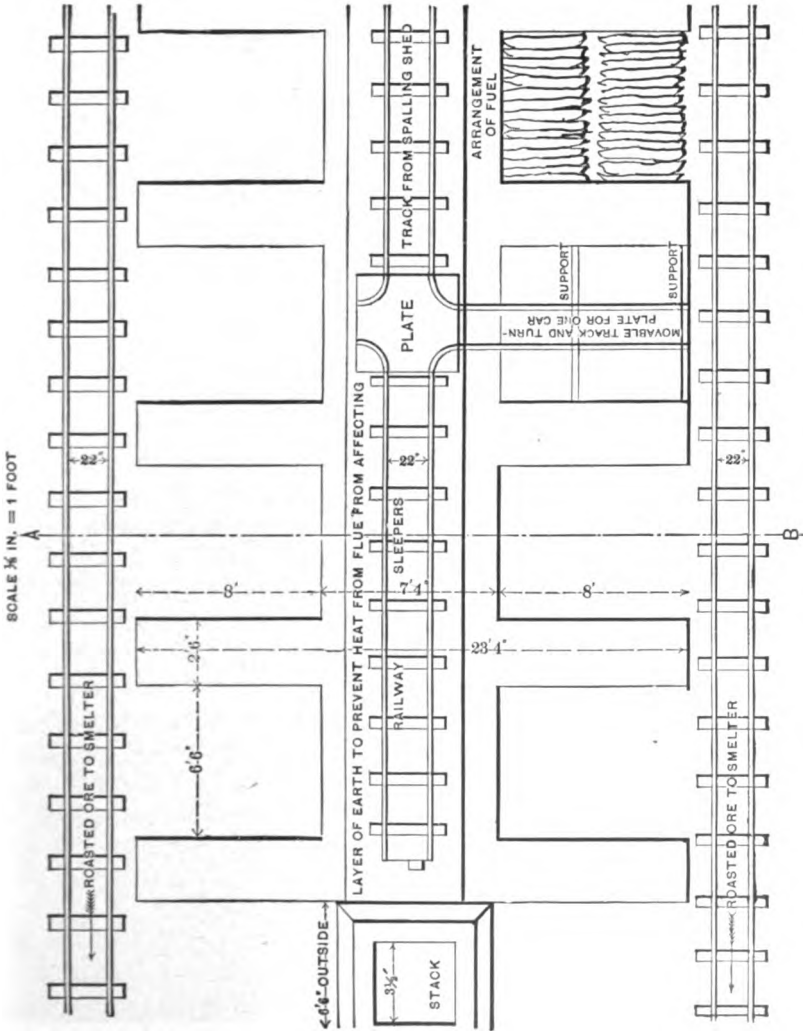
FIG. 20. — Roast stalls for ore — plan
