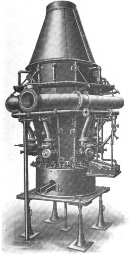
FIG. 45. — Sectionalized 10-sided furnace
