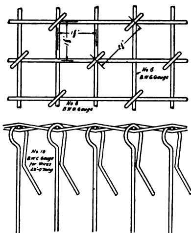
FIG. 113. — Method of hanging wires in dust-chamber
