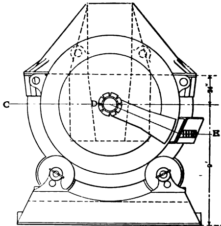
FIG. 91. — Barrel converter — end elevation
