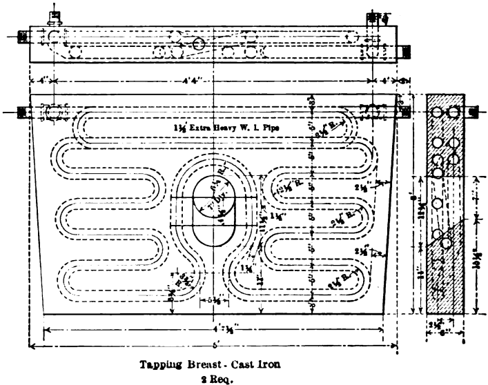
FIG. 64. — Cananea blast-furnace cast-iron tapping breast
