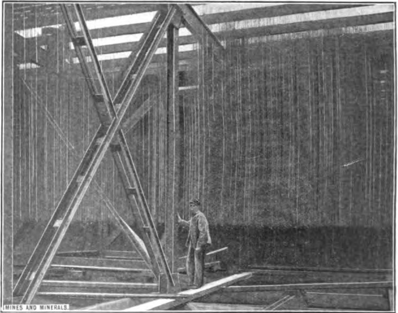
FIG. 114. — Interior of dust-chamber after hanging wires
