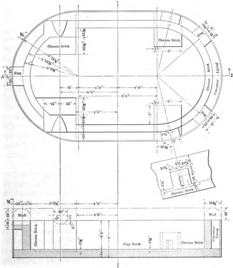
FIG. 68. — Cananea blast-furnace. Method of lining a settler
