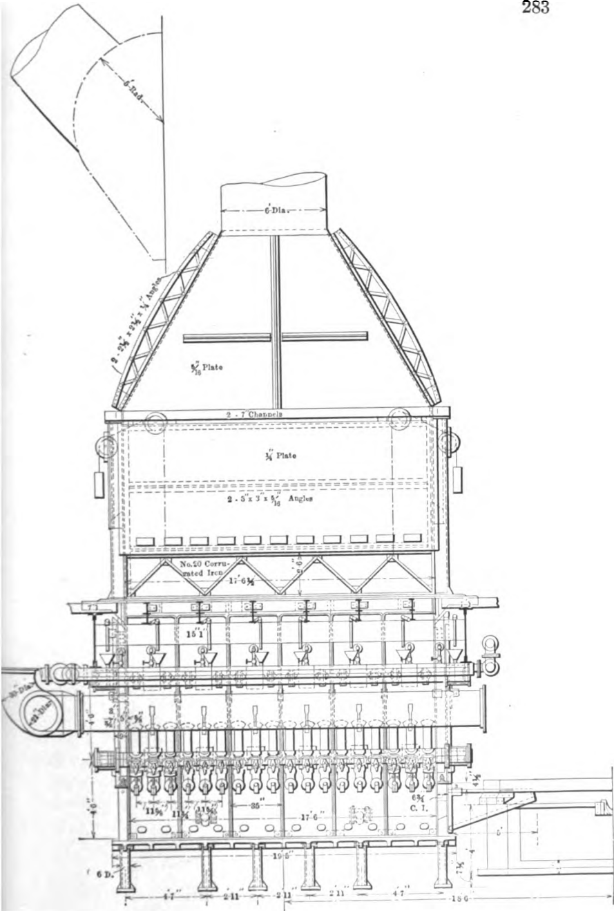
FIG. 62. — Cananea blast furnace — side
