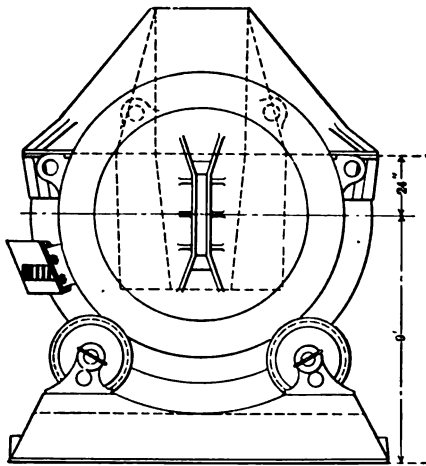
FIG. 90. — Barrel converter — end elevation
