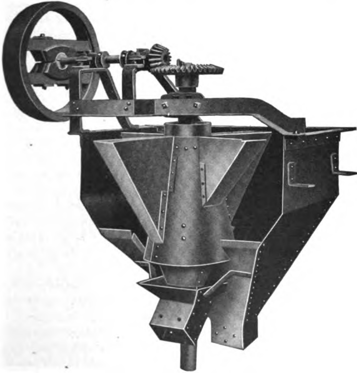
FIG. 6. — The Vezin automatic sampler
