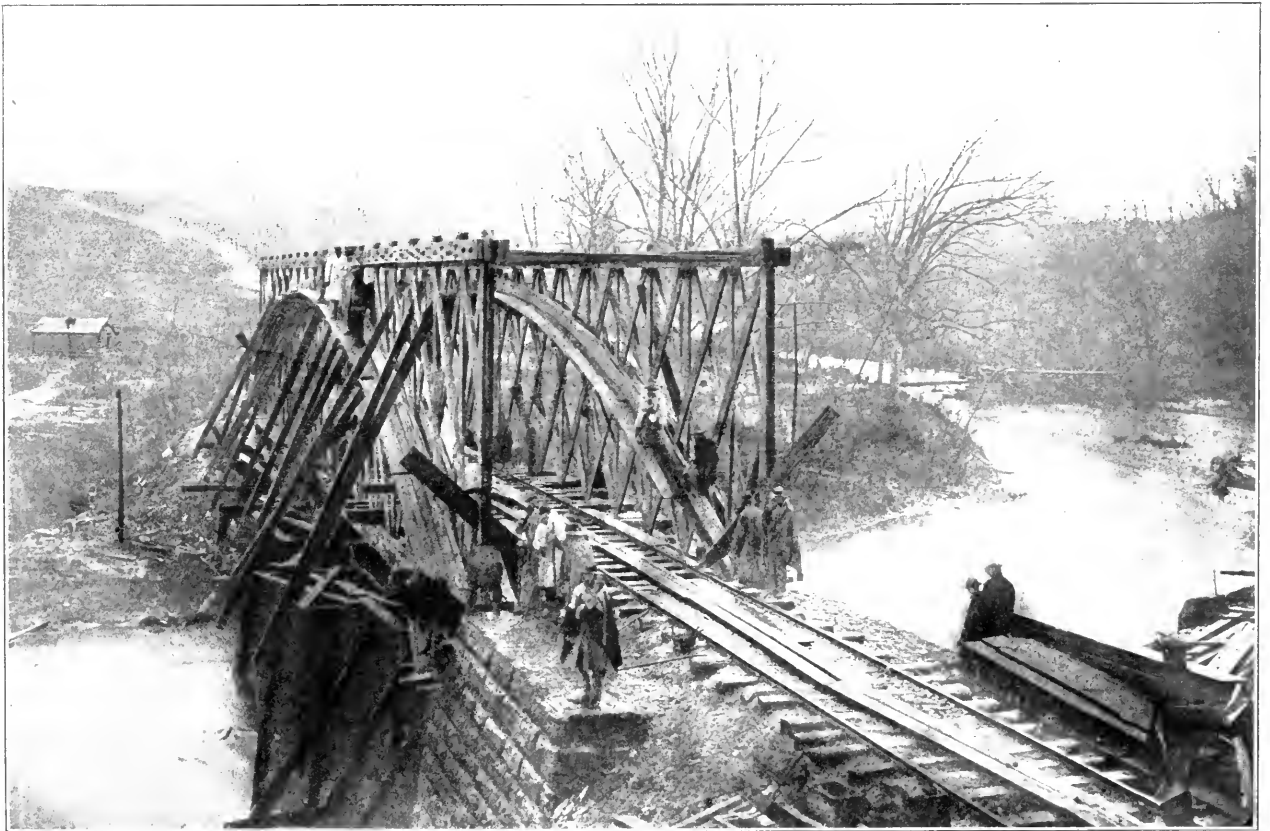
REINFORCED WITH TRUSSES—TRANSFORMED INTO A STANDARD BRIDGE
