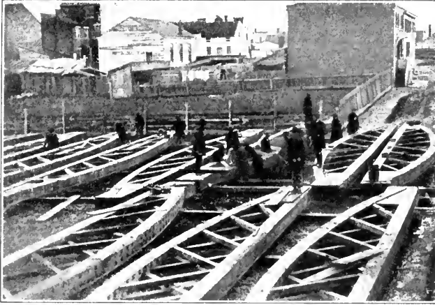
BUILDING PORTABLE BRIDGE-TRUSSES
