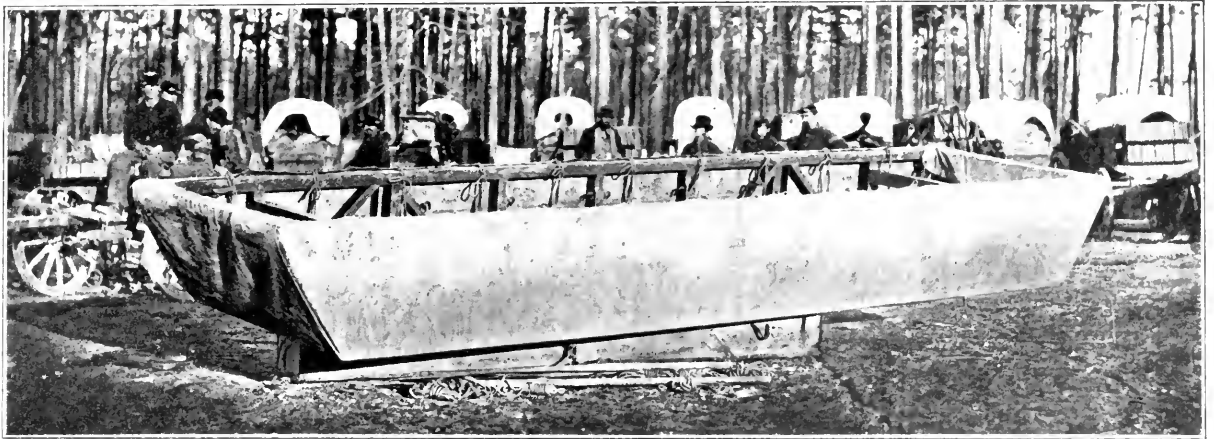
A CANVAS PONTOON BOAT ASSEMBLED READY FOR BUSINESS—MARCH, 1864
