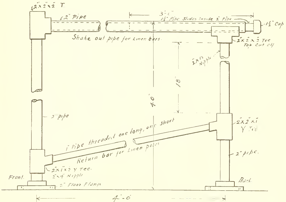
4'-0" Shake Out Stand With Slide Bar 2 Wanted.
