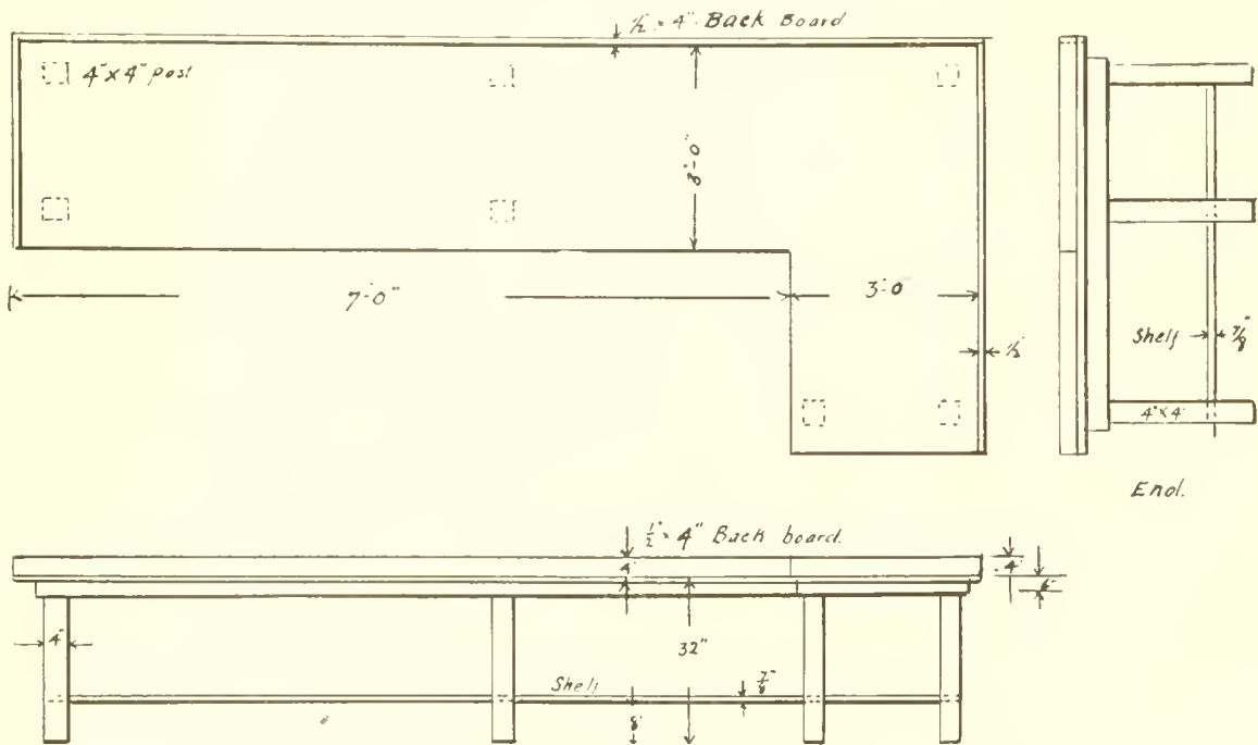
Assemble Table. One Wanted
