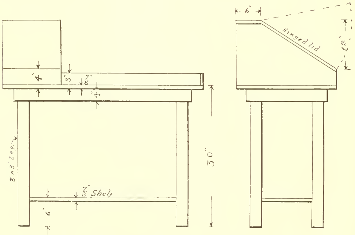
Lister Table and Desk. One Wanted
