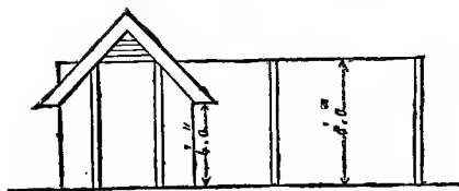
END ELEVATION.
