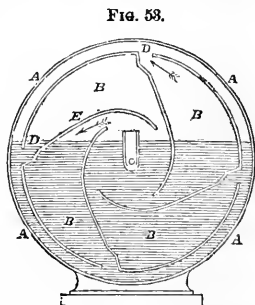
Fig. 53. Meter for measuring the flow of Gas.
