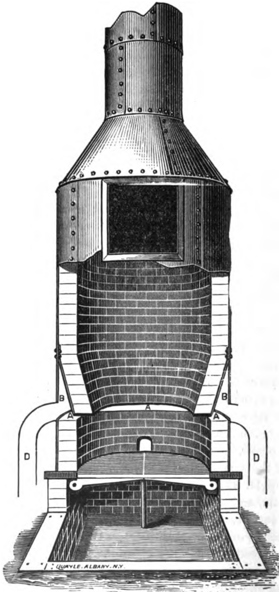
MACKENZIE CUPOLA.
