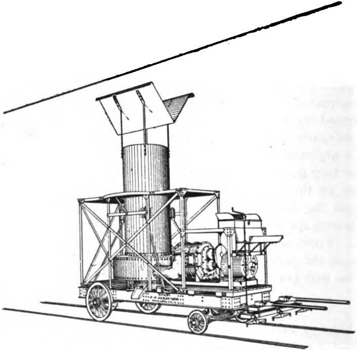
PAXON TRUCK AND TRACK CUPOLA.
