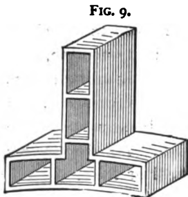
REVERSED T TUYERE.
