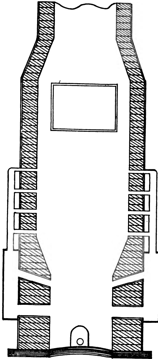
STEWART'S CUPOLA.
