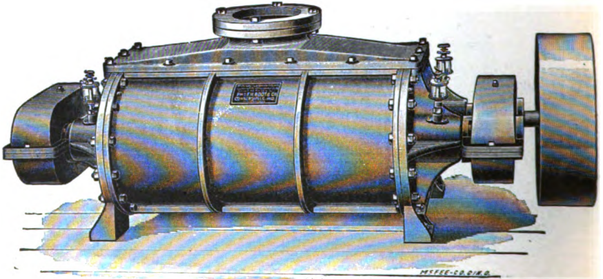
ROOT'S HORIZONTAL PRESSURE BLOWER.
