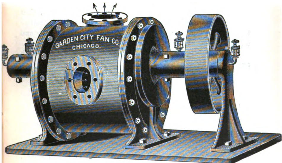
GARDEN CITY POSITIVE BLAST BLOWER.
