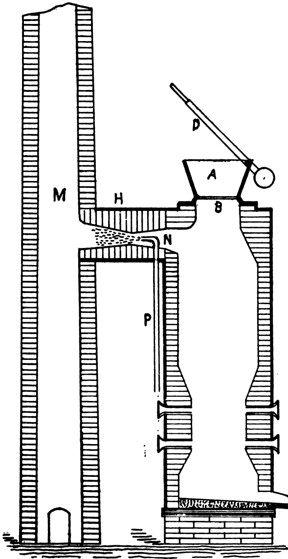
WOODWARD'S STEAM-JET CUPOLA.
