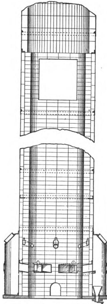
SECTION OF PAXSON HOT BLAST CALLIAU CUPOLA.
