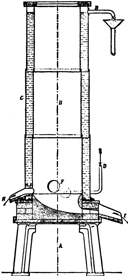
DR. OTTO GMELIN'S CUPOLA.
