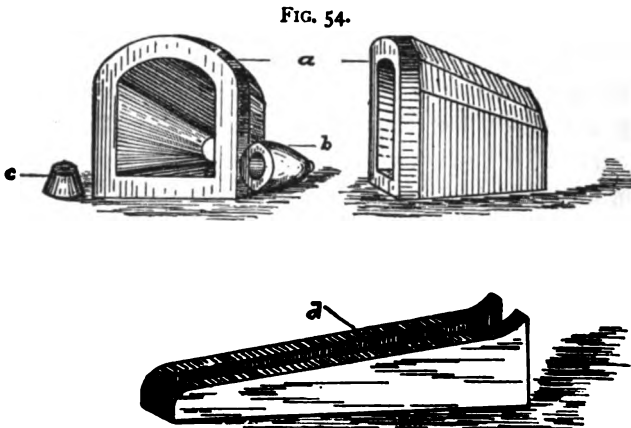
MOOR'S PATENT CUPOLA BREAST AND RUNNER.
