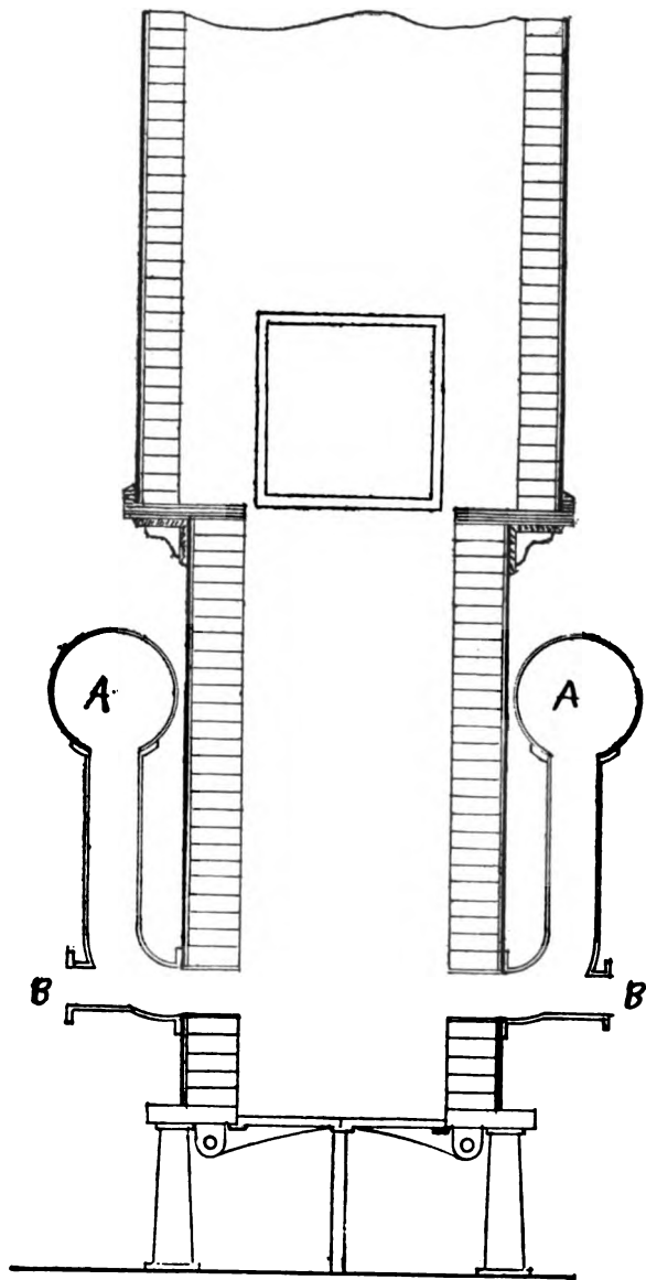
SPARK CATHING DEVICE IN MODERN CUPOLA.
