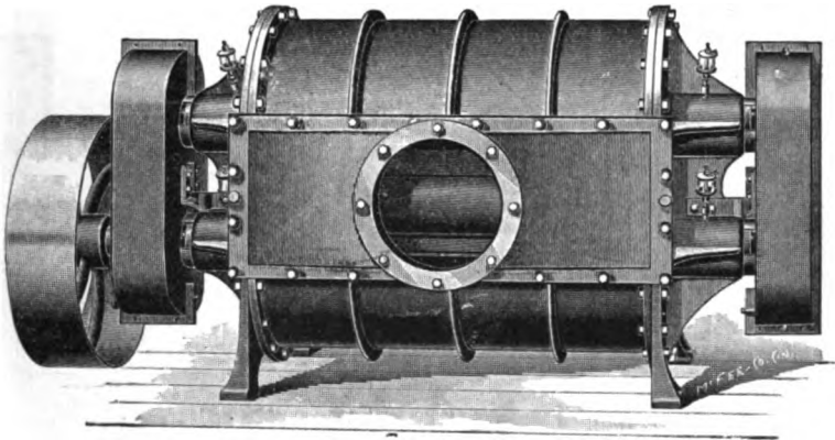
ROOT'S VERTICAL PRESSURE BLOWER.
