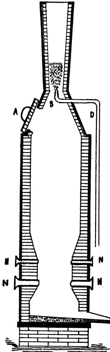
WOODWARD STEAM-JET CUPOLA.
