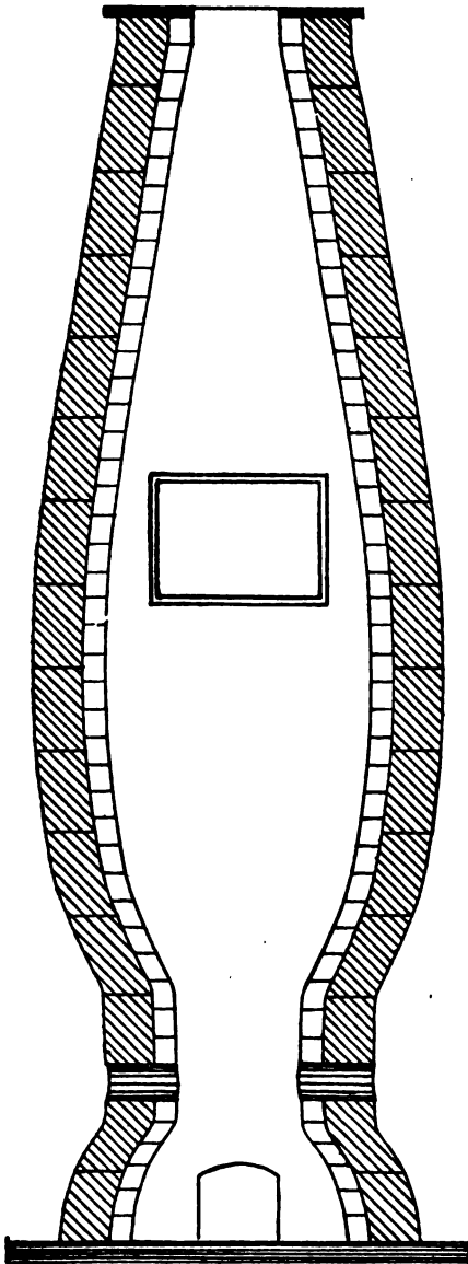
EXPANDING CUPOLA.
