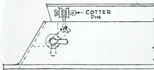
ELEVATION DAMPER OPEN
