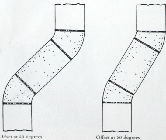
Sketch showing offsets made with 45 degree and 60 degree offset fittings
