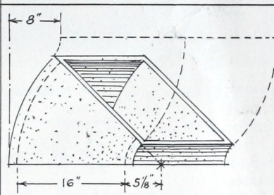
OFFSET FOR 13" X 18" FLUE PRICE $5.00 EACH.
