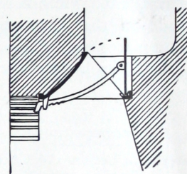
Drawing showing Damper with front flange omitted for use in fireplace having curved arch. These are made to order without extra charge.
