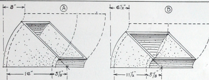
OFFSETS FOR 13" X 13" FLUES SEE NOTE ABOVE. PRICE $4.25 EACH
