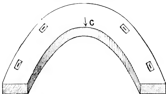
FIG. 76.—Toe of hind shoe showing the edge which cuts the heel of fore-foot.
