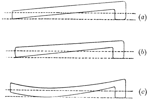
FIG. 39.—The dotted lines show the effect of wear and its relation to the shape of the shoe.
