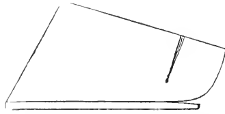
FIG. 85.—Bearing relieved at wrong place by "springing" the heel.
