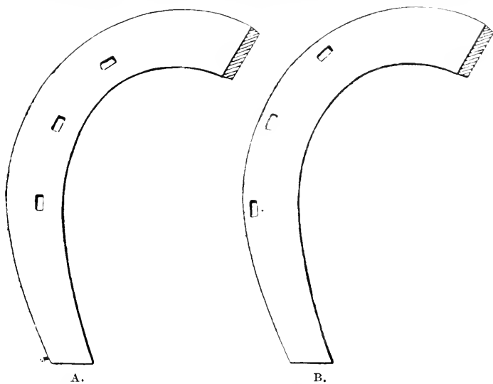
FIG. 42.—Wrongly placed Nail-holes (A too coarse, B too fine).
