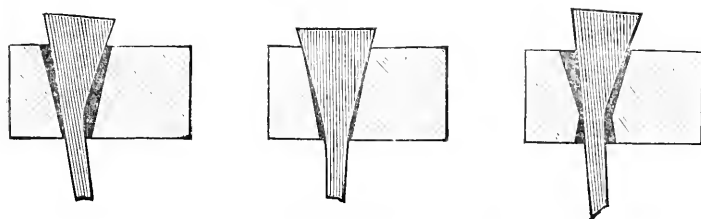
FIG. 41.—Good and bad nail-holes.
