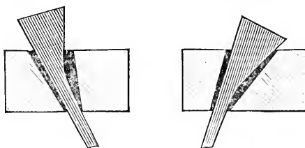
FIG. 43.—Nail-holes "pitched" in and out.
