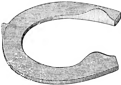
FIG. 89.—Shoe with heel clips for sandcrack.
