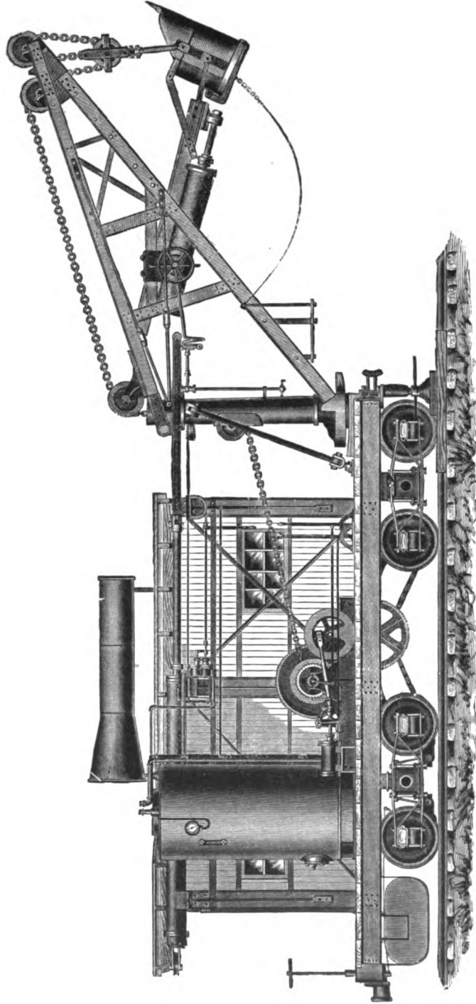
FIG. 6.—CLEMENT STEAM SHOVEL ; Industrial Works, Bay City, Mich.
