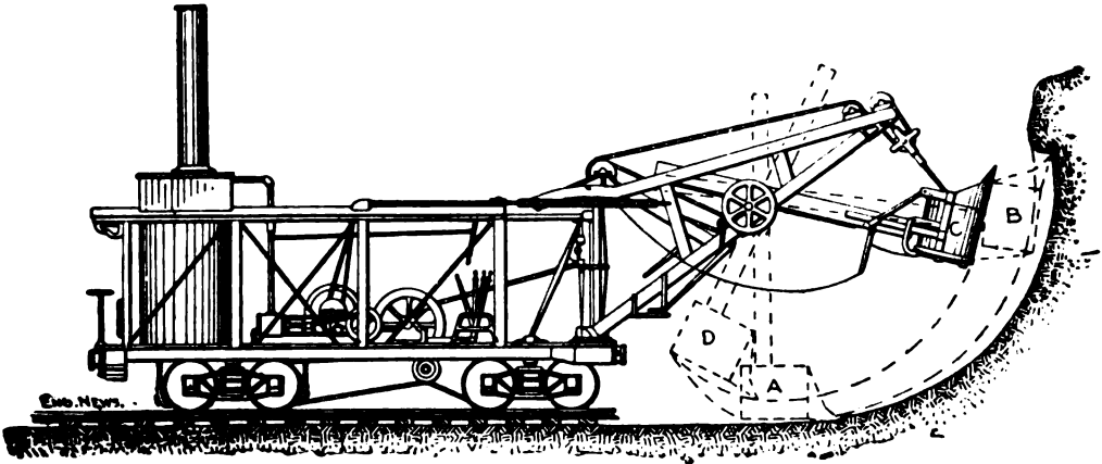
Fig. 15.—Showing Series of Operations for Excavating.
