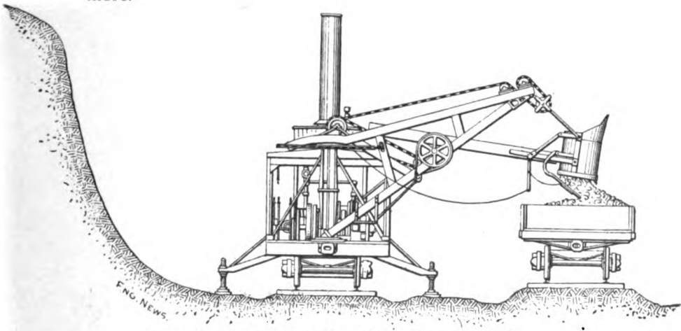
Fig. 16.—Loading Earth from Steam Shovel Onto Cars.
