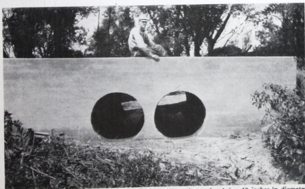
Figure 23. A double culvert built in Lee County, Iowa, each opening being 42 inches in diameter and 20 feet long. The wing walls are 20 feet long, 8 feet high and 10 inches thick. This was built with the Merrillat Culvert Core Company's form at a total cost of $112.
