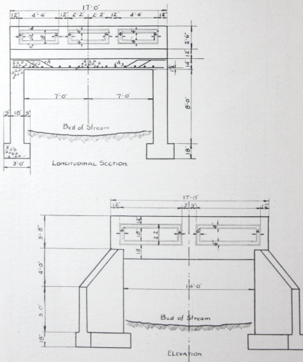
Figure 38. Section and elevation of bridge shown in Figure 40.
