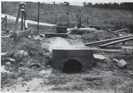
Figure 51. Two Concrete Culverts near Rice Lake, Wisconsin. 24-inch diameter; 17-feet long. Built over forms of Concrete Form & Engine Co., at cost of $10.25 each.
