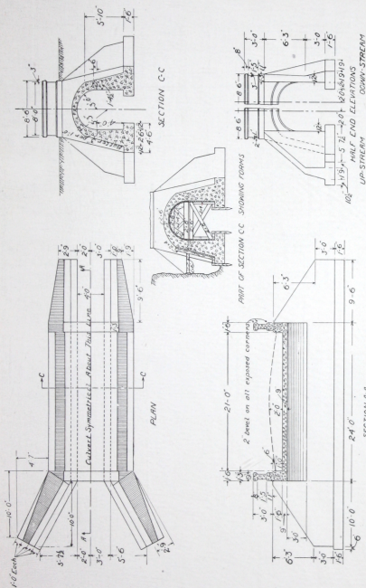
PLAN FOR A PLAIN CONCRETE ARCH CULVERT
