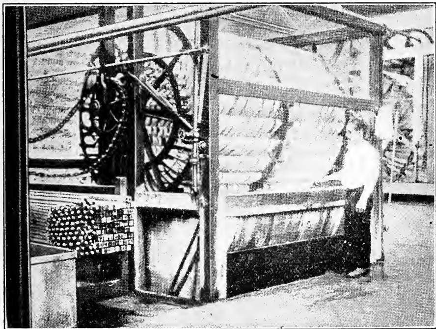
FIG. 83. — Dyeing. Skein dyeing by machinery.
