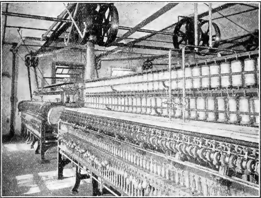
FIG. 55. — Flax spinning.
