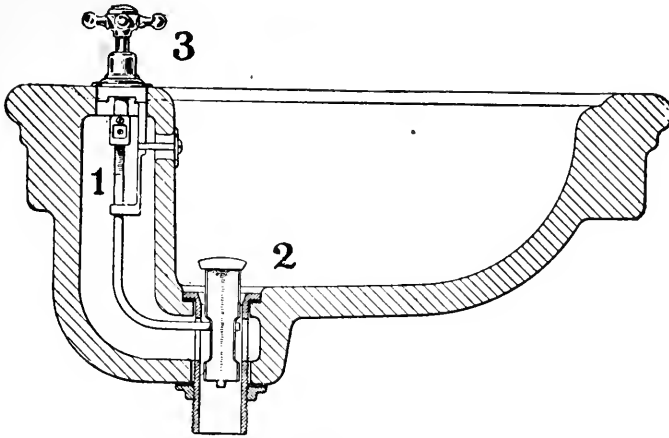
FIG. 17. — Cross section of a basin.
