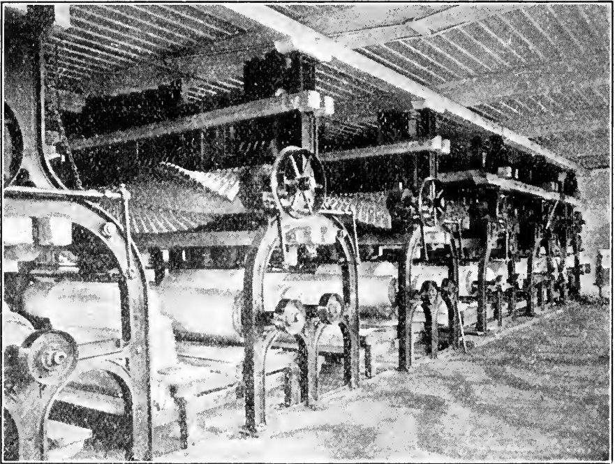
FIG. 62. — Beetling, a finishing process of linen.
