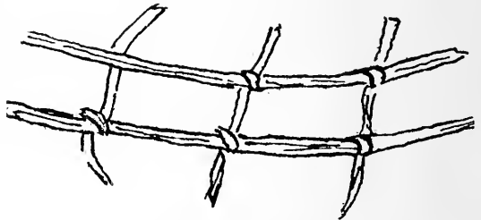
FIG. 144.—Detail of method of twisting spokes about head wires.
