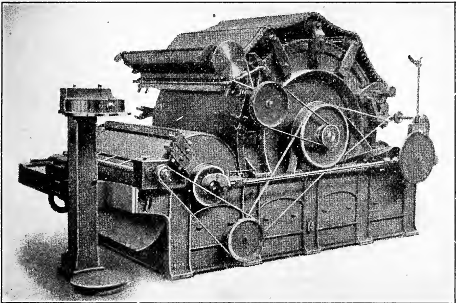
FIG. 44. — Revolving flat card for cotton. Delivery side.
