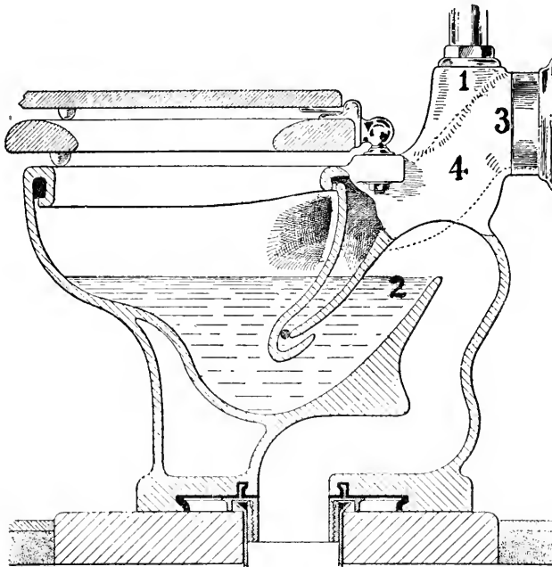
FIG. 18. — Cross section of a siphon water-closet.
