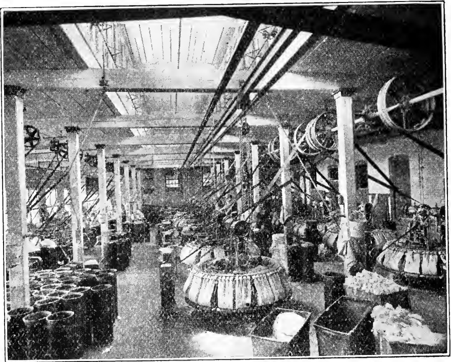
FIG. 68. — Wool combing. This machine is used in the manufacture of high grade wools. There is much waste.
