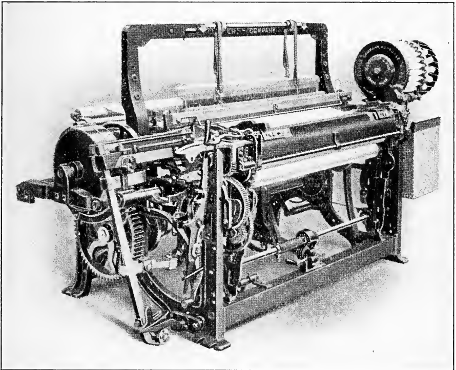
FIG. 50. — Northrup loom for weaving plain material.
