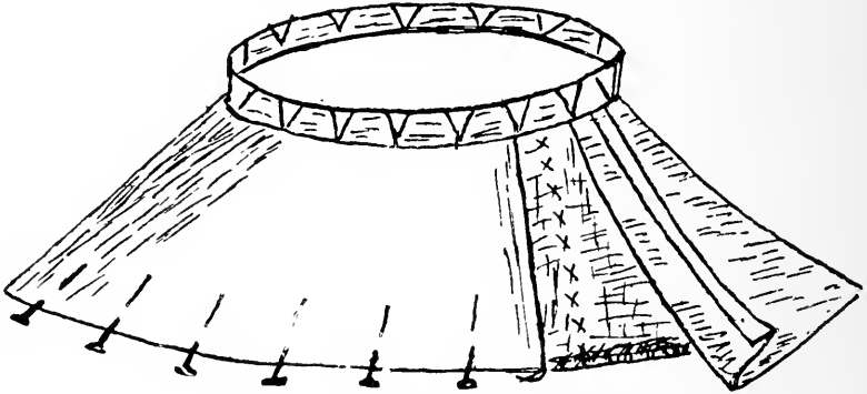
FIG. 142. — Covering buckram frame.
