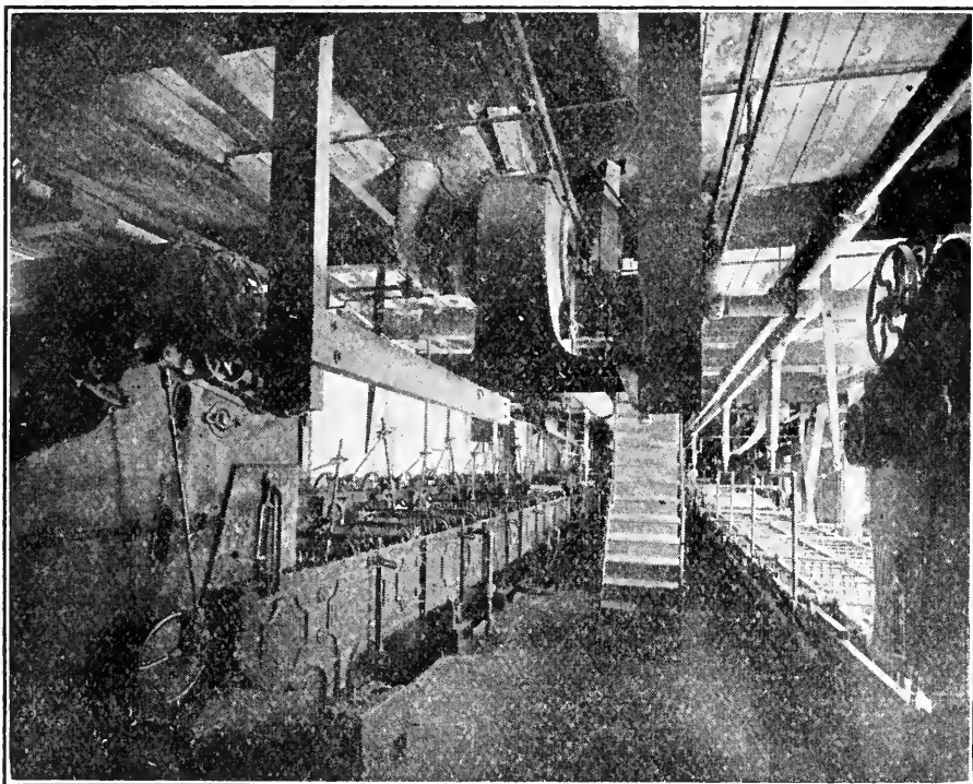
FIG. 66. — Wool washing or scouring. Notice the rakes in the machines which move the wool back and forth in scouring.
