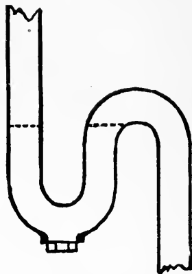
FIG. 14. — Cross section of an S trap.
