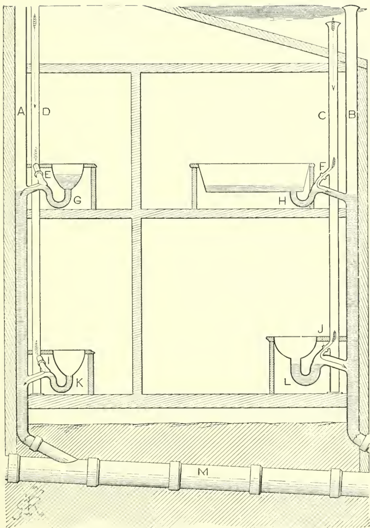
PLATE 14 - NON-SIPHONING TRAPS
